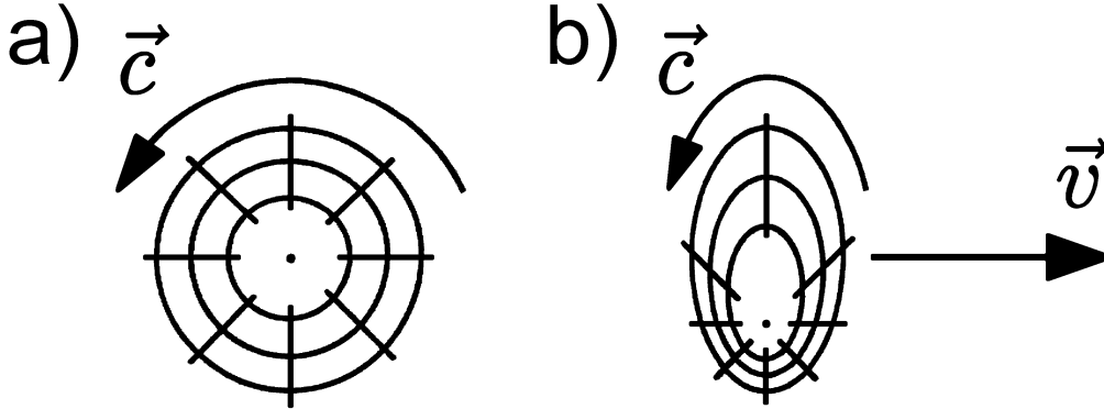
Figure 4: Schematic diagram of a localised-photon model: a) at rest (the proper frame), and b) moving at speed \vec{v} , where the object as a whole is Lorentz contracted in the direction of motion and the circulating photon is alternately red and blue shifted. The ticks mark equal intervals in phase, and the line density represents the momentum density.
