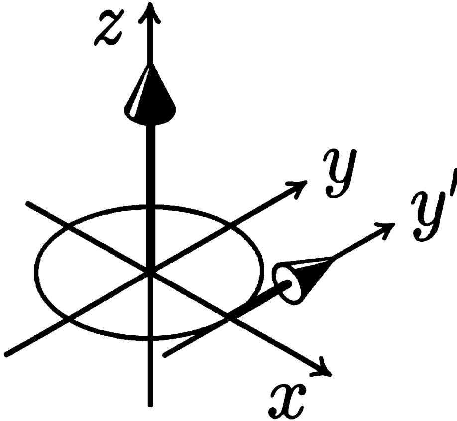
Figure 3: Definition of a co-ordinate system with the z -axis passing through the center of the torus. At any instant an element of field will be rotating both around the z -axis (orbital spin), and about a perpendicular axis tangential to the eye of the torus (intrinsic photon angular momentum). The tangential spin-axis performs a rotation in the x, y -plane about the z -axis with frequency 2\omega_C and radius \lambda_C/4\pi .
