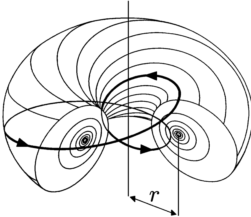
Figure 2: Schematic of the internal energy flow in the model. The lines of flow (geodesics) circulate twice around a family of nested toroidal surfaces before closing on themselves. The left-handed case is illustrated. For clarity, one complete double-loop path is emphasised. The toroidal structure is characterised by a length r = \lambda_C/4\pi .
