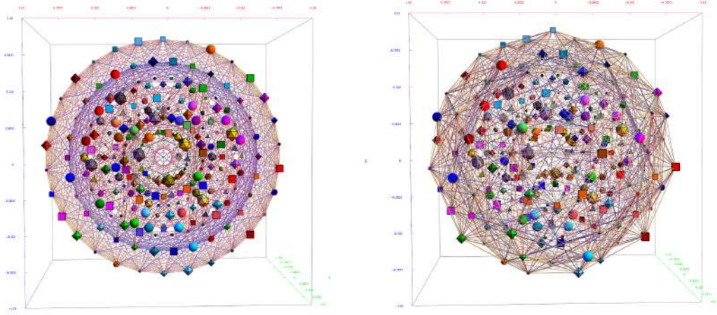
FIG. 11: E_8 showing the Petrie projection face orientation in 2D and 3D perspective with vertices as physics particle assignments. Vertex shape, size, color/shade are assigned based on extended Standard Model particle assignments. Only 1220 of 6720 edges are shown in order to prevent occlusion of vertices in 3D perspective.
