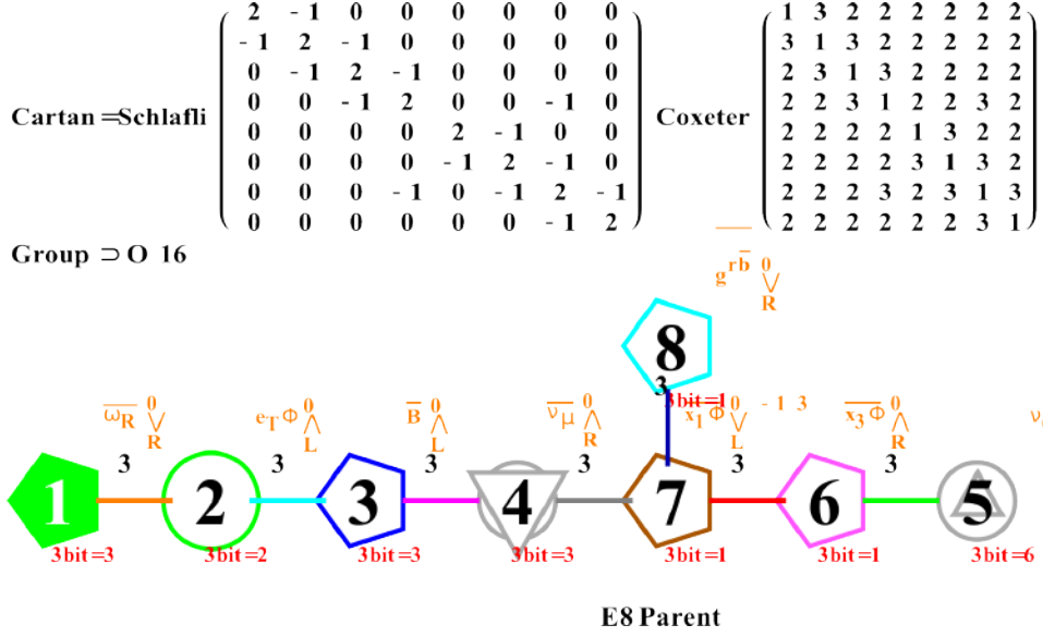
FIG. 7: E_8 Dynkin diagram with Cartan, Schlafli, and Coxeter matrices
