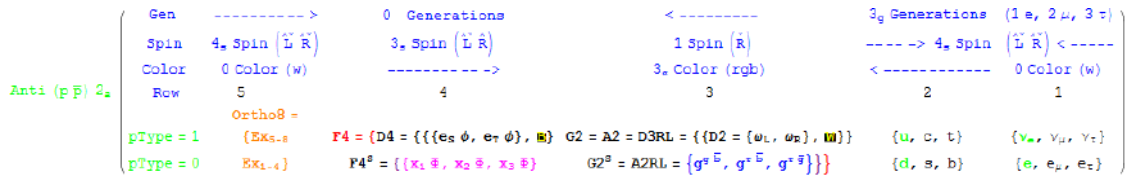
FIG. 10: Particle flavors in row / column groups with boson {group} coloring based on Lie group assignments ( F_4 , F_4^B , D_4 \& G_2 , G_2^B )
