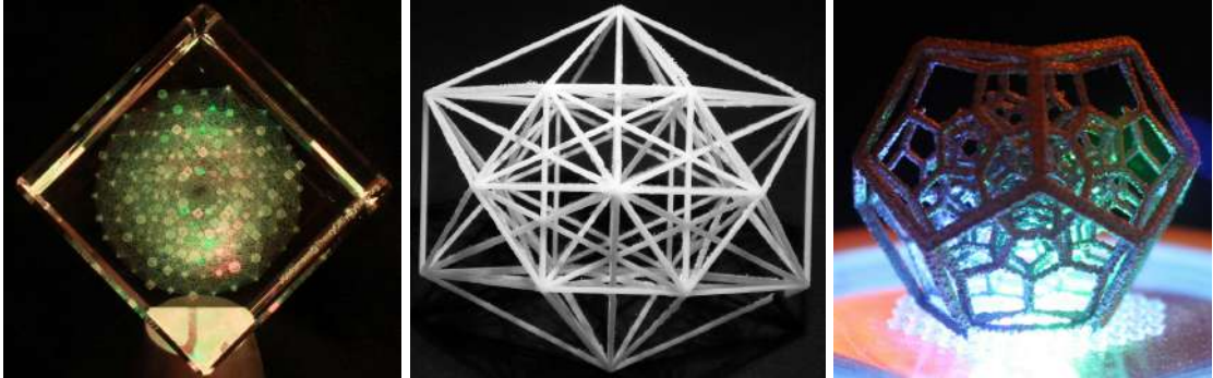
FIG. 14: The E_8 to H_4 3D projection model used to laser etch optical crystal
