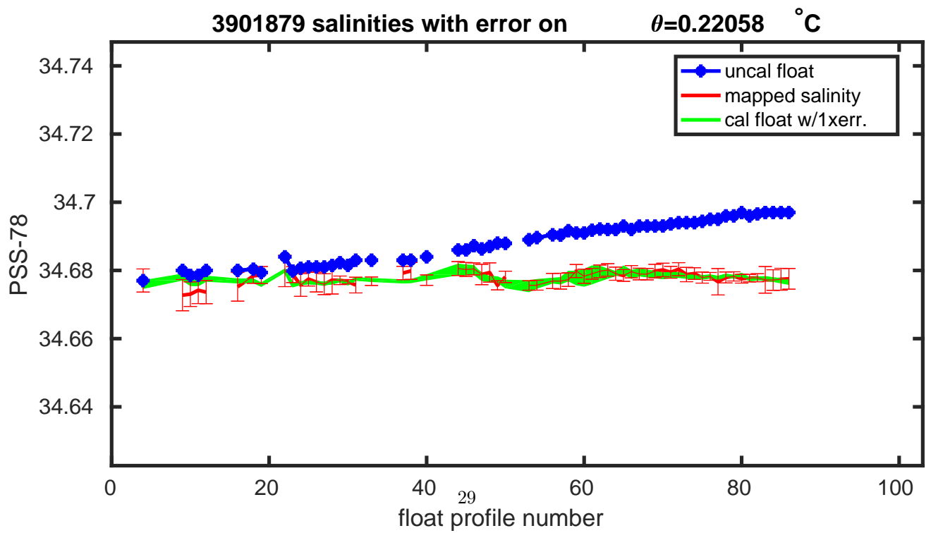
Figure 20: Float 3901879. Salinities with errors on \theta .
