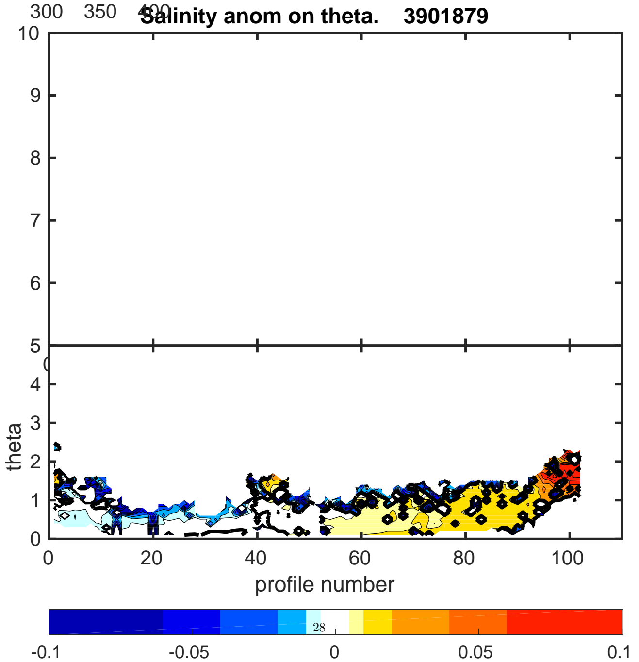
Figure 19: Float 3901879. Salinity anomaly on Theta
