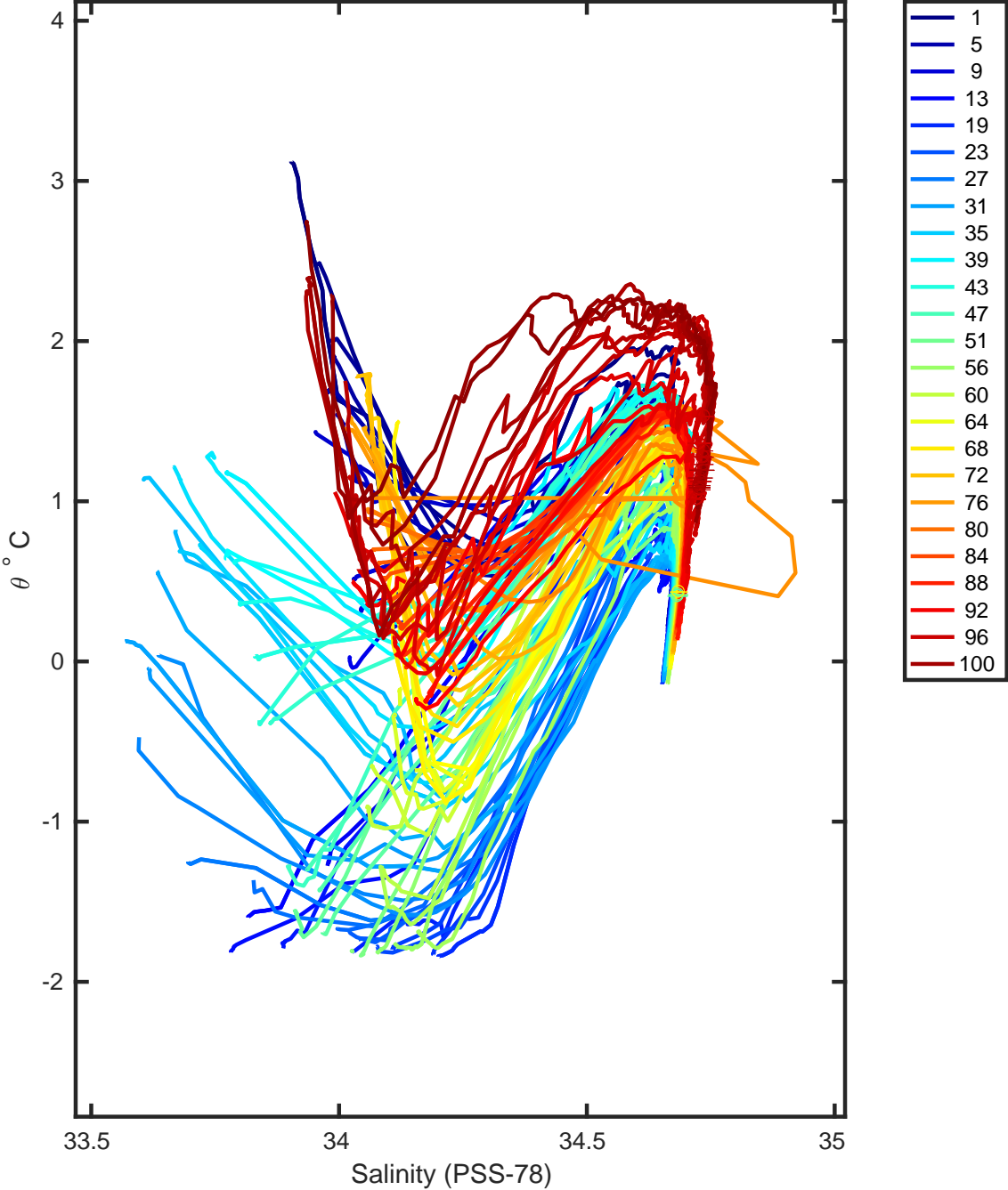
Figure 10: Float 3901879. Calibrated float data and mapped salinity.
