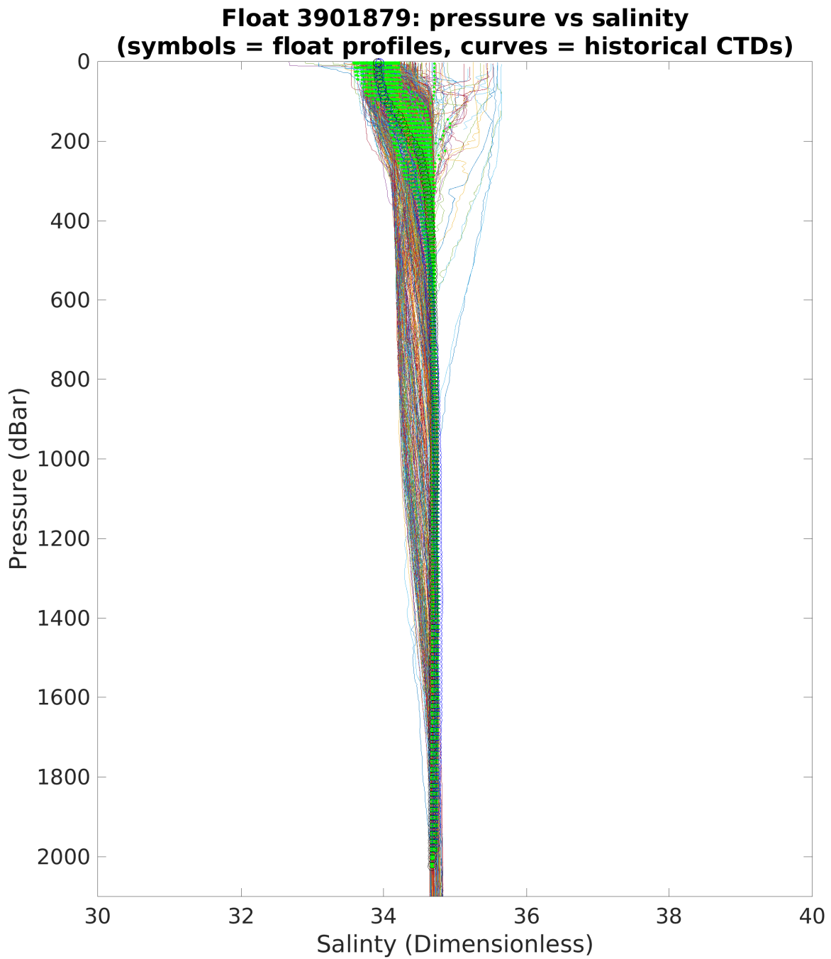
Figure 4: Float 3901879. Float profile of salinity (dimensionless) plotted with climatology from the spatial range of 10^\circ . The black and blue cycles indicates the first and the last Argo profile, respectively. Green symbols represent other Argo profiles.
