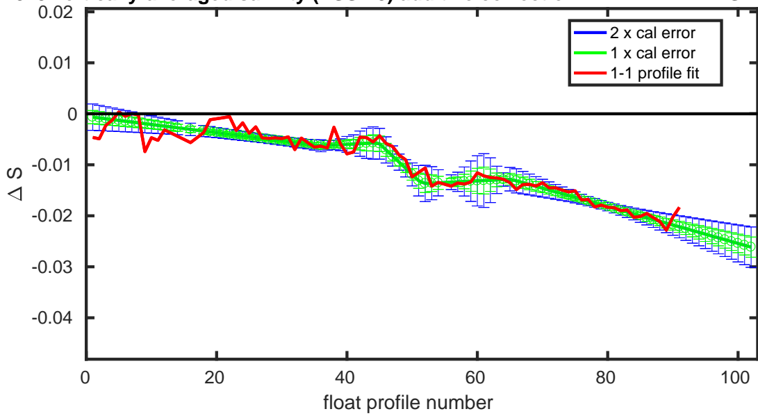
Figure 17: Float 3901879. Potential conductivity (top) and vertically averaged salinity (bottom) with errors.
