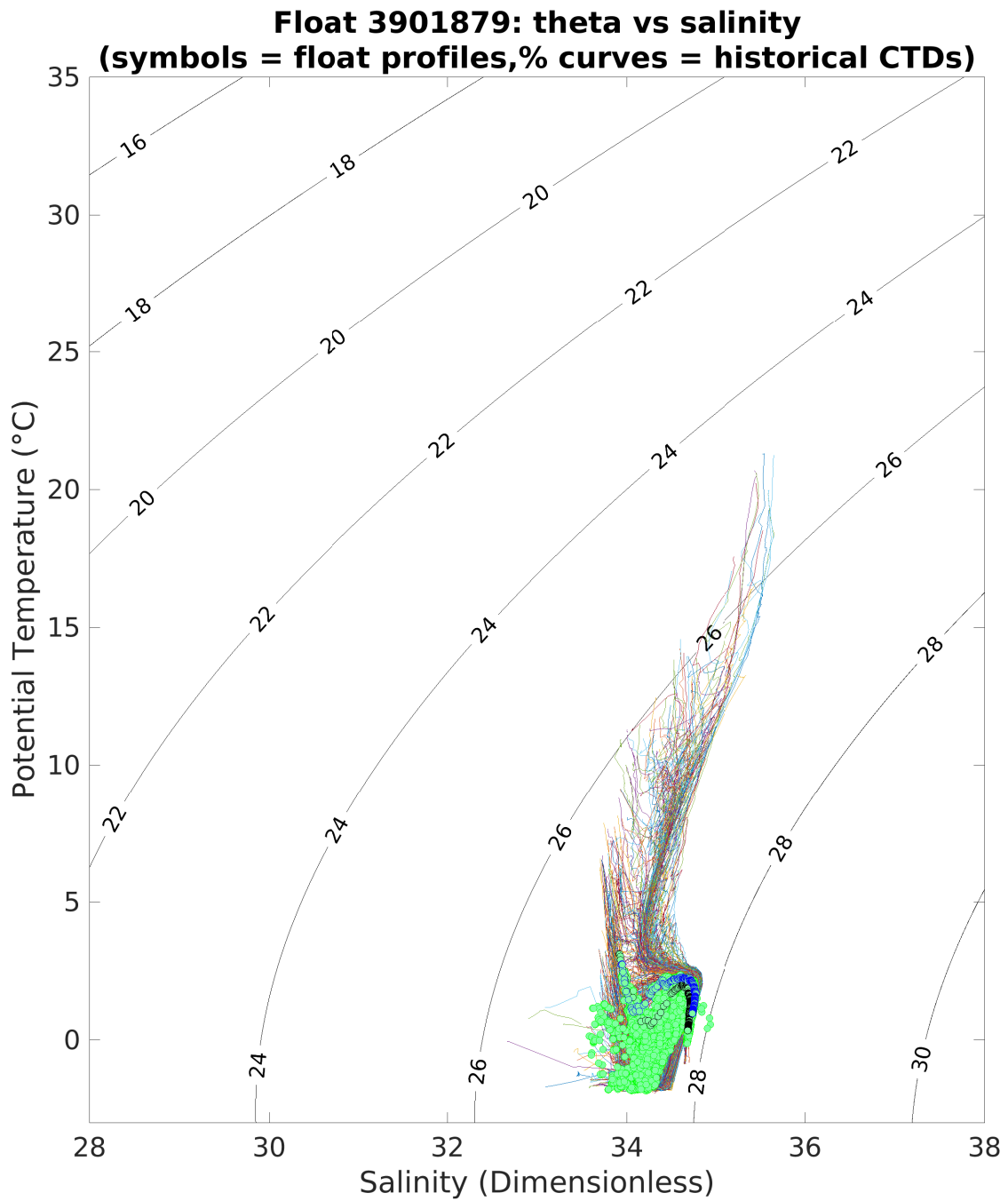
Figure 5: Float 3901879. Theta/S plotted with climatology from the spatial range of 10°. The black and blue circles indicate the first and the last Argo profile, respectively. Green symbols represent other Argo profiles.
