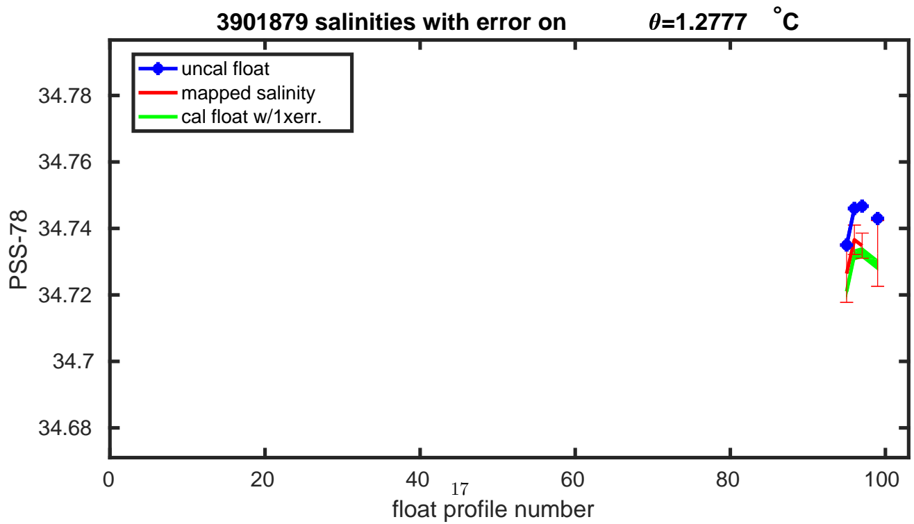
Figure 12: Float 3901879. Salinities with errors on \theta levels.
