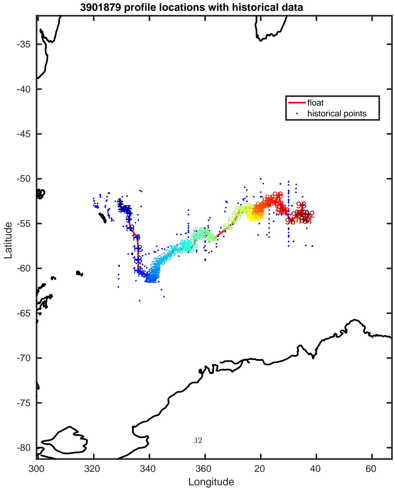
Figure 7: Float 3901879. Trajectory of the float with historical CTD data. The black contours indicate the bathymetry at 0, 200, 1000 and 2000 m.
