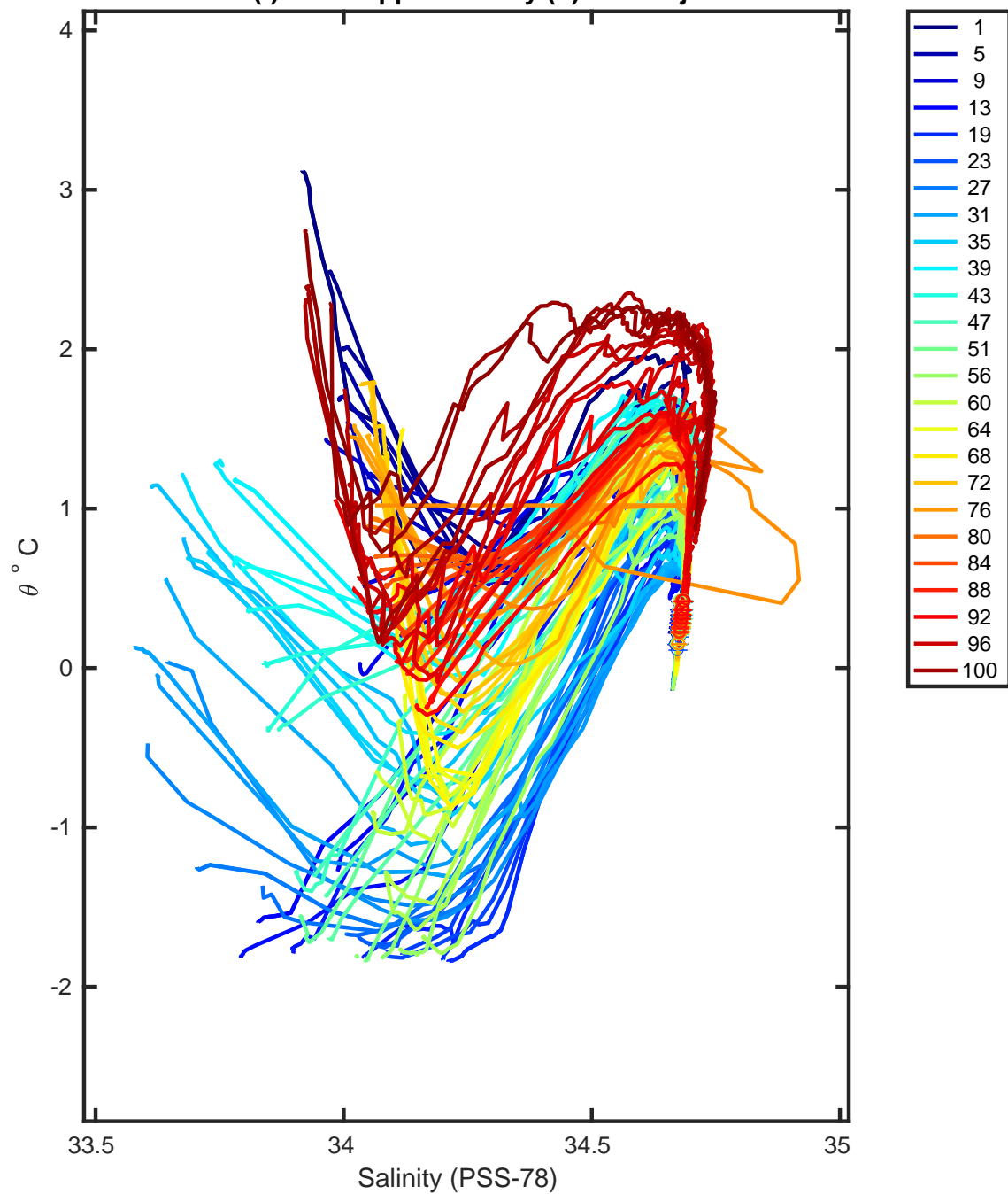
Figure 18: Float 3901879. Calibrated float data and mapped salinity.
