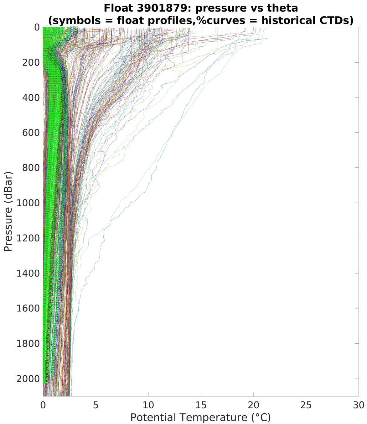
Figure 3: Float 3901879. Float profile of potential temperature (°C) plotted with climatology from the spatial range of 10°. The black and blue cycles indicates the first and the last Argo profile, respectively. Green symbols represent other Argo profiles.
