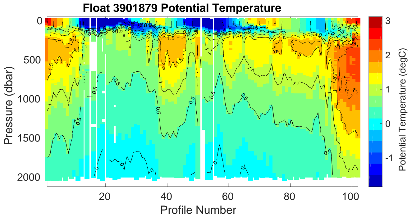
Figure 1: Float 3901879. Time series of the vertical distribution of potential temperature ( ^{\circ}\text{C} ).
