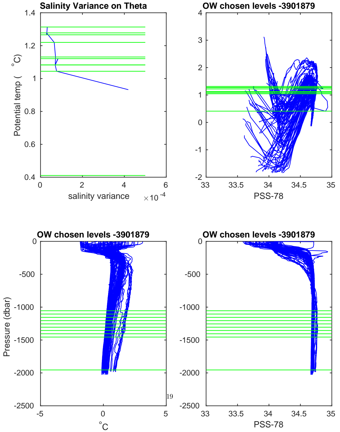
Figure 14: Float 3901879. Salinity, salinity variance on theta and OW chosen levels.
