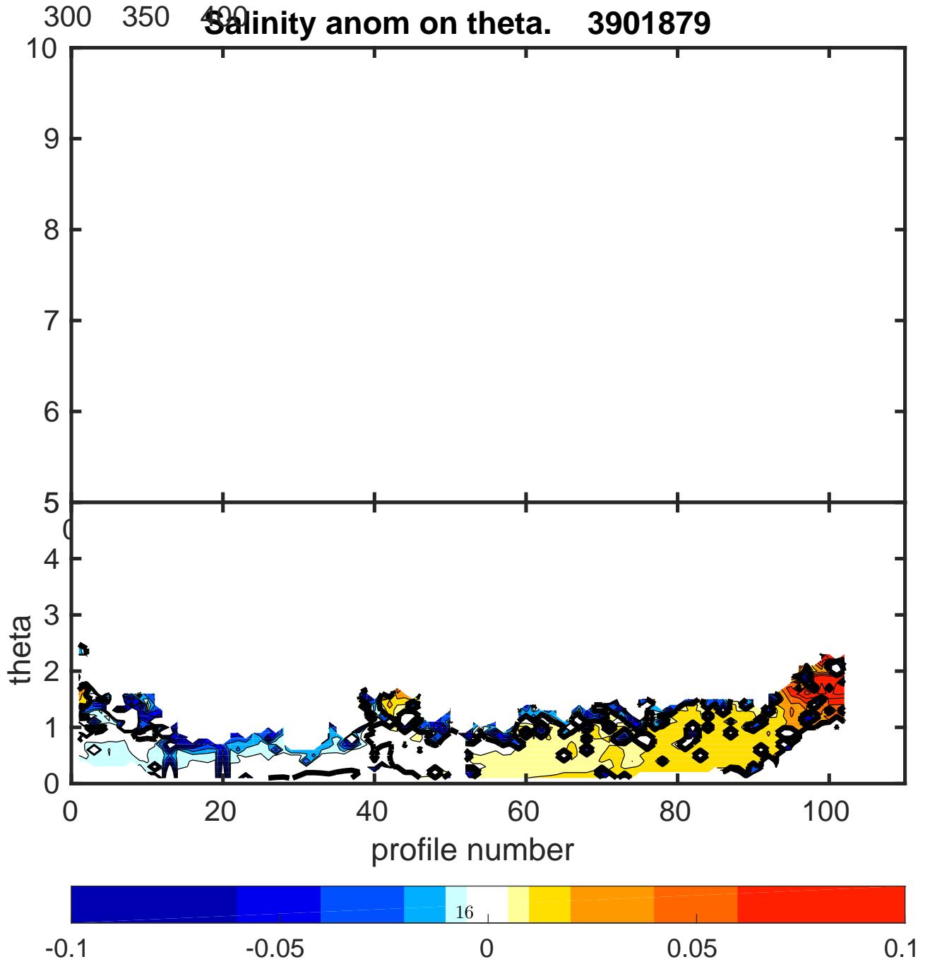
Figure 11: Float 3901879. Salinity anomaly on \theta levels.
