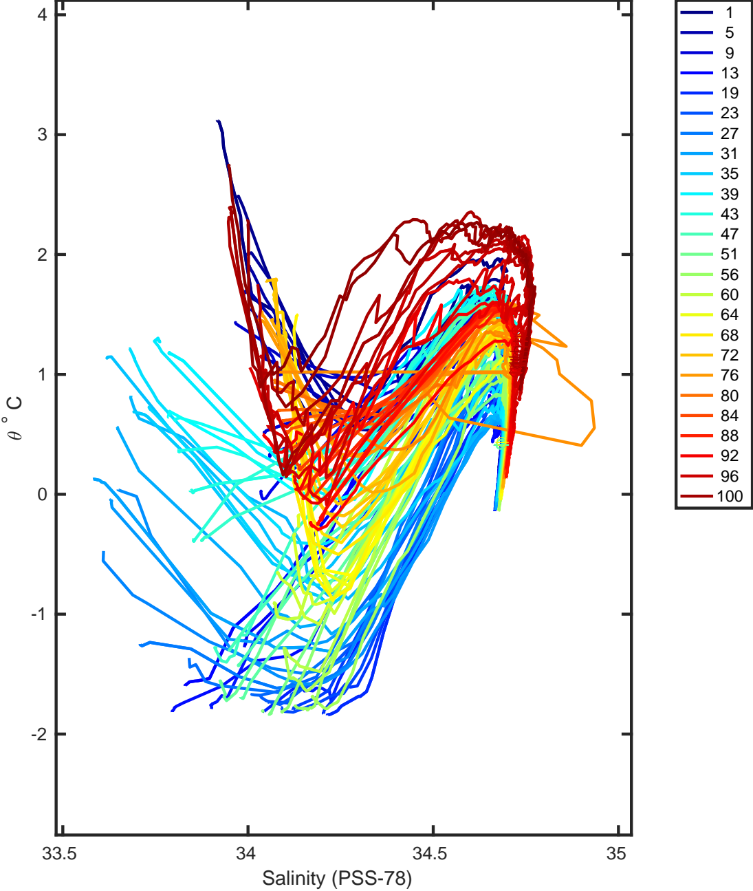
Figure 8: Float 3901879. Uncalibrated float data and mapped salinity.
