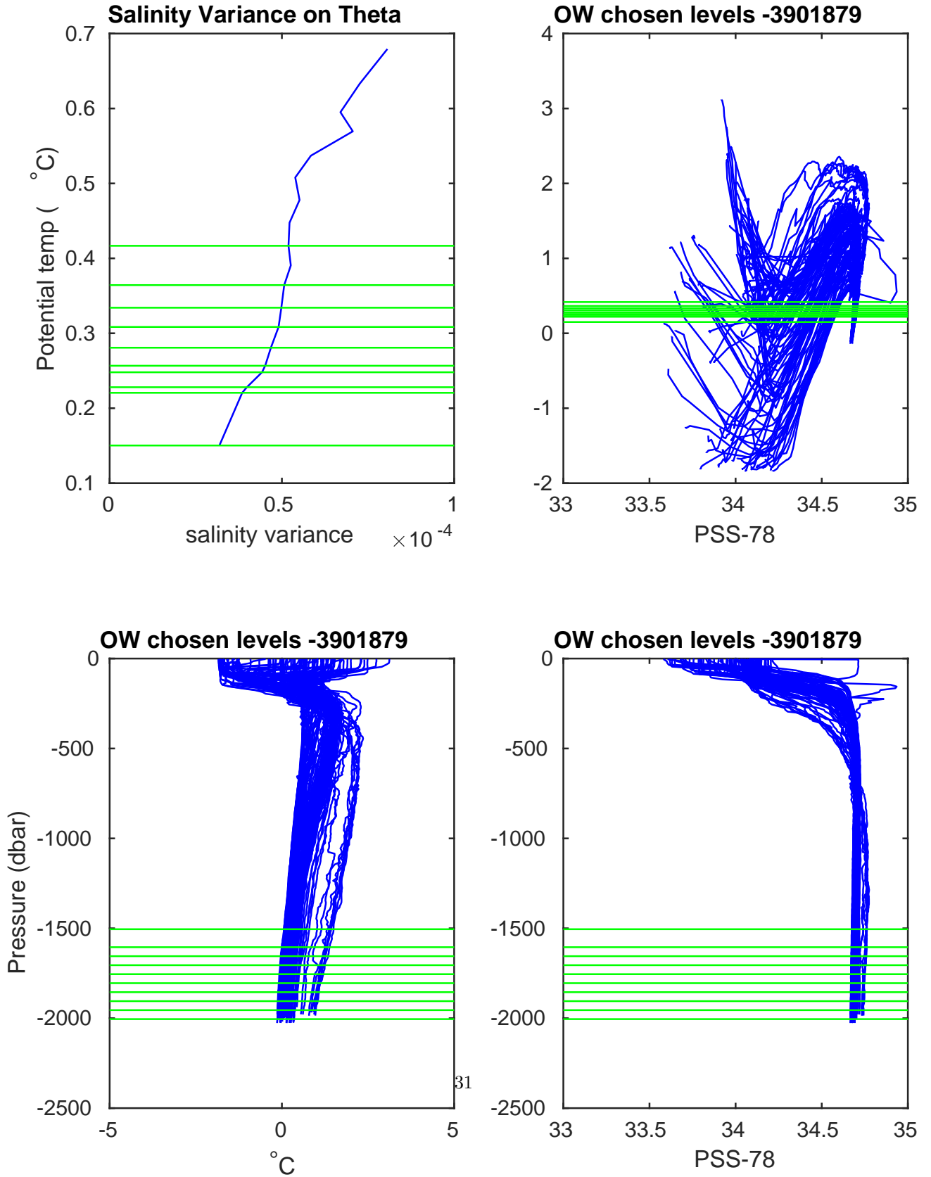
Figure 22: Float 3901879. Salinity, salinity variance on theta and OW chosen levels.
