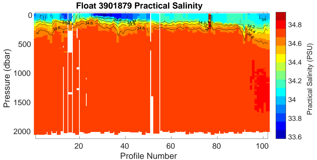
Figure 2: Float 3901879. Time series of the vertical distribution of practical salinity (PSU).
