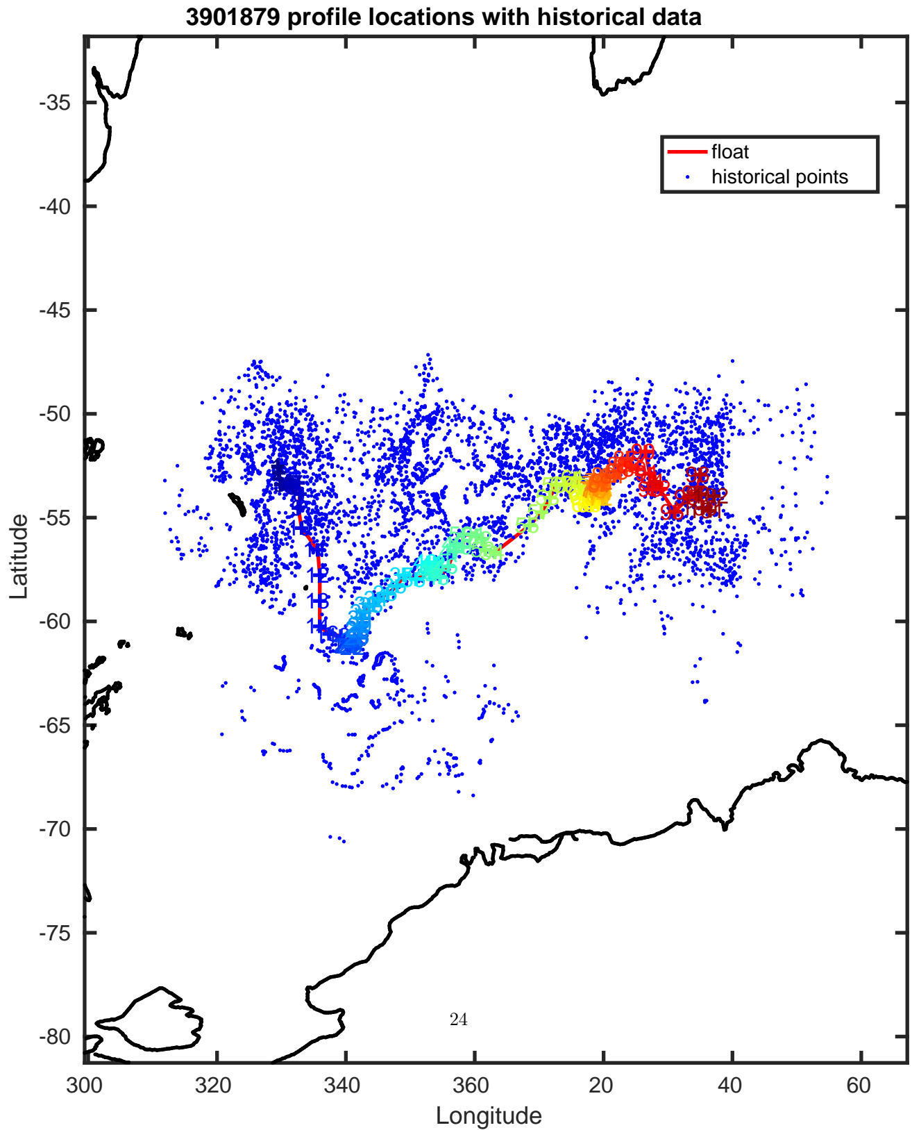
Figure 15: Float 3901879. Trajectory of the float with historical CTD data. The black contours indicate the bathymetry at 0, 200, 1000 and 2000 m.
