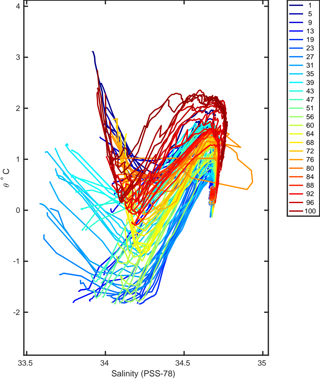
Figure 16: Float 3901879. Uncalibrated float data and mapped salinity.
