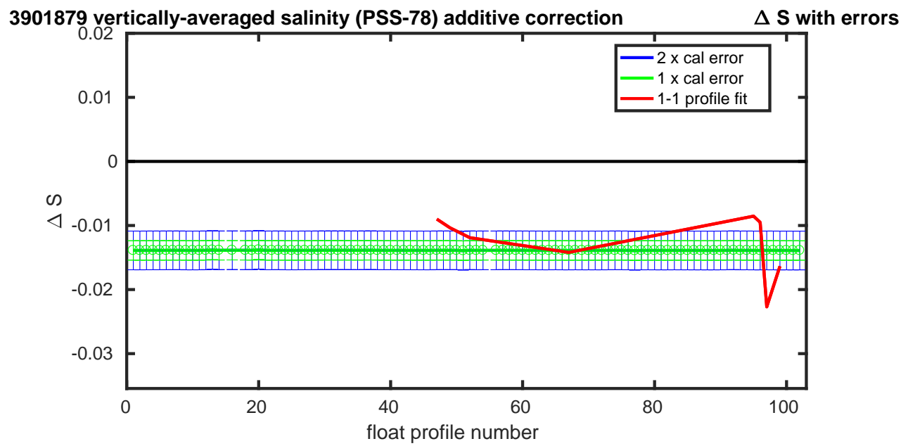
Figure 9: Float 3901879. Potential conductivity (top) and vertically averaged salinity (bottom) with errors.
