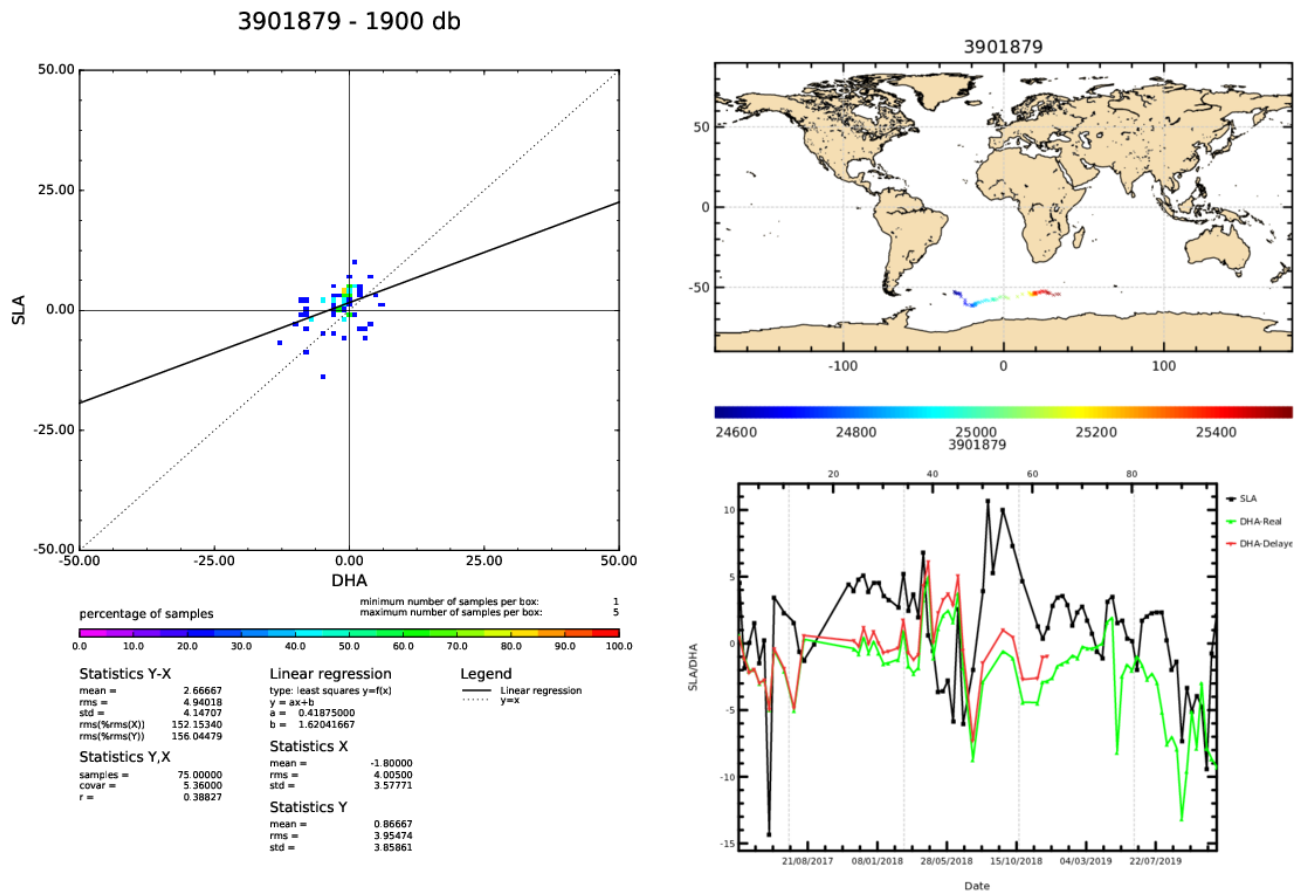
Figure 6: Float 3901879. The comparison between the Sea Surface Height (SSH) from the satellite altimetry and Dynamic Height Anomaly (DHA) extracted from the Argo float temperature and salinity data
