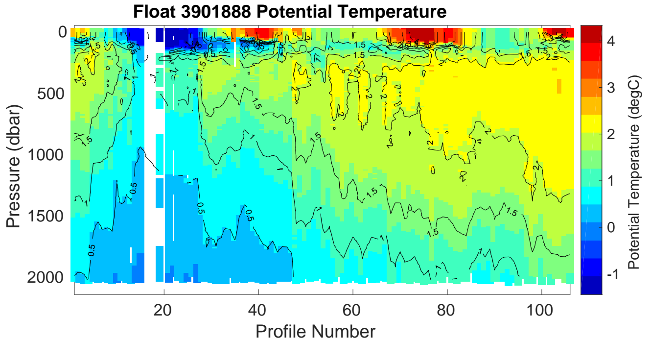
Figure 1: Float 3901888. Time series of the vertical distribution of potential temperature ( ^{\circ}\text{C} ).
