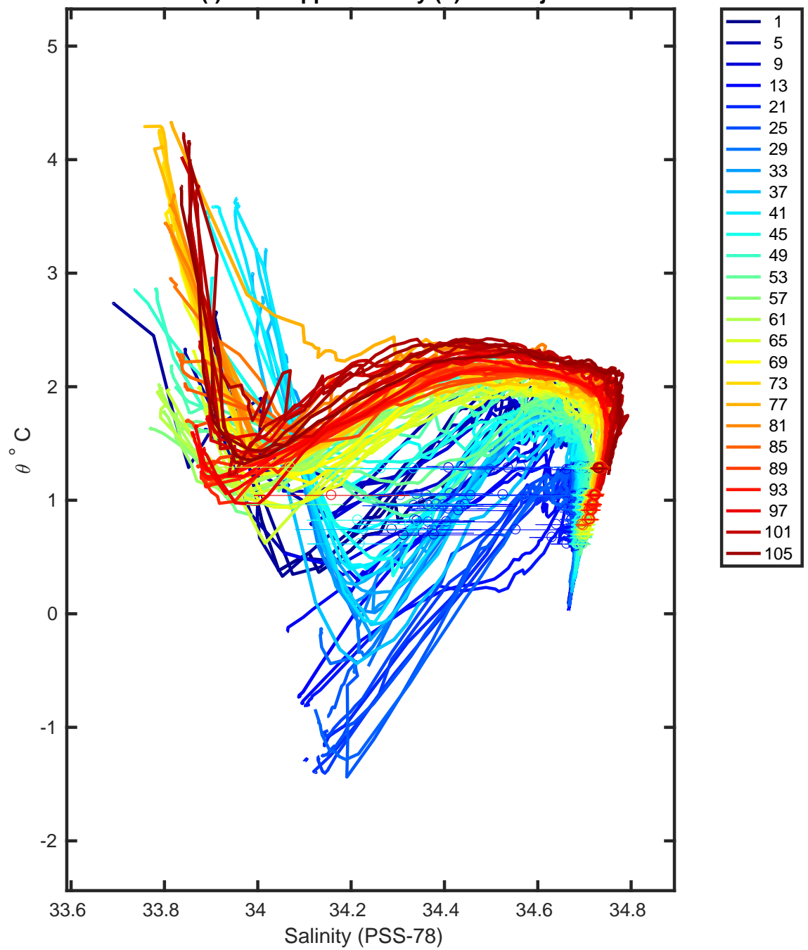
Figure 18: Float 3901888. Calibrated float data and mapped salinity.
