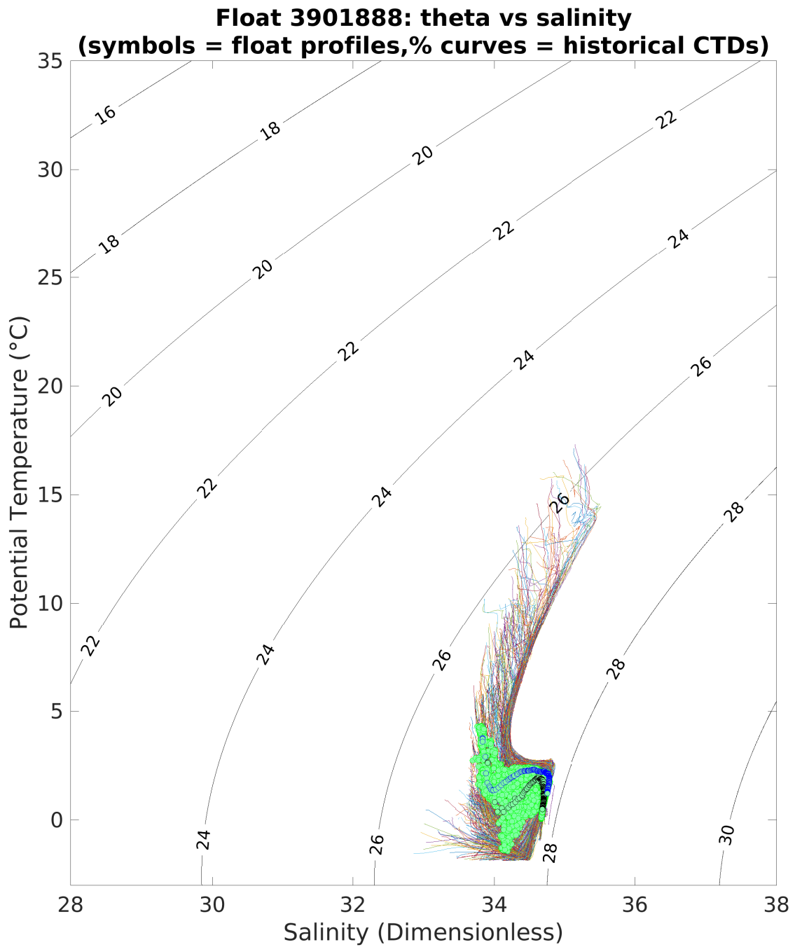
Figure 5: Float 3901888. Theta/S plotted with climatology from the spatial range of 10°. The black and blue cycles indicates the first and the last Argo profile, respectively. Green symbols represent other Argo profiles.
