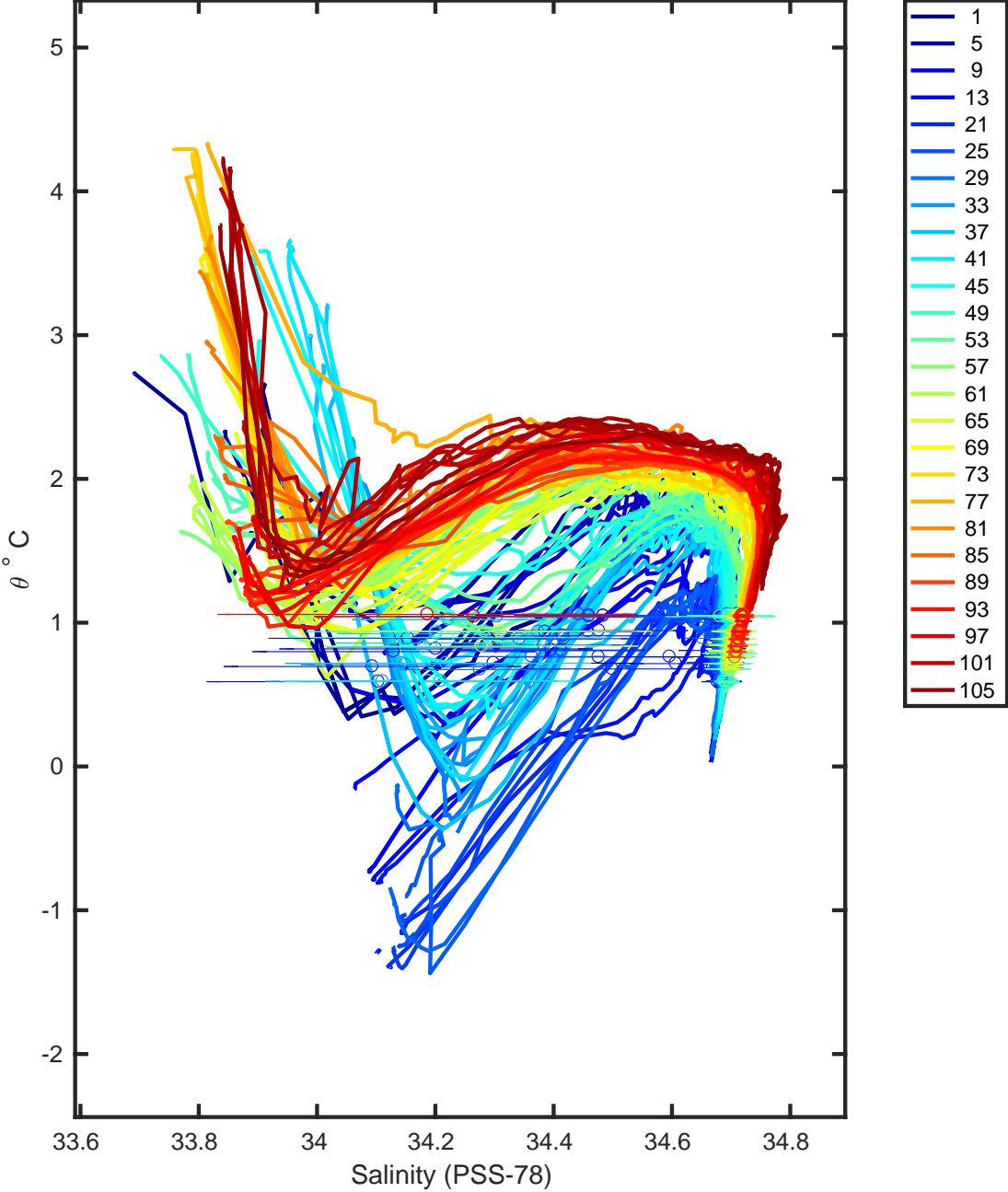
Figure 8: Float 3901888. Uncalibrated float data and mapped salinity.
