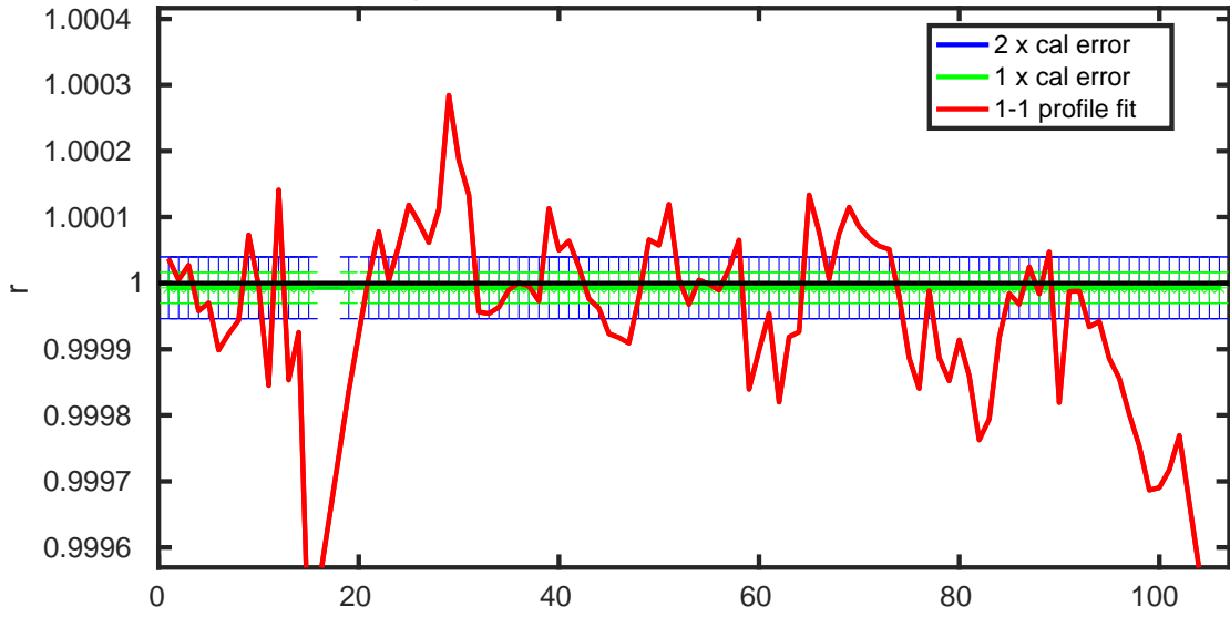
3901888 potential conductivity (mmho/cm) multiplicative correction r with errors
