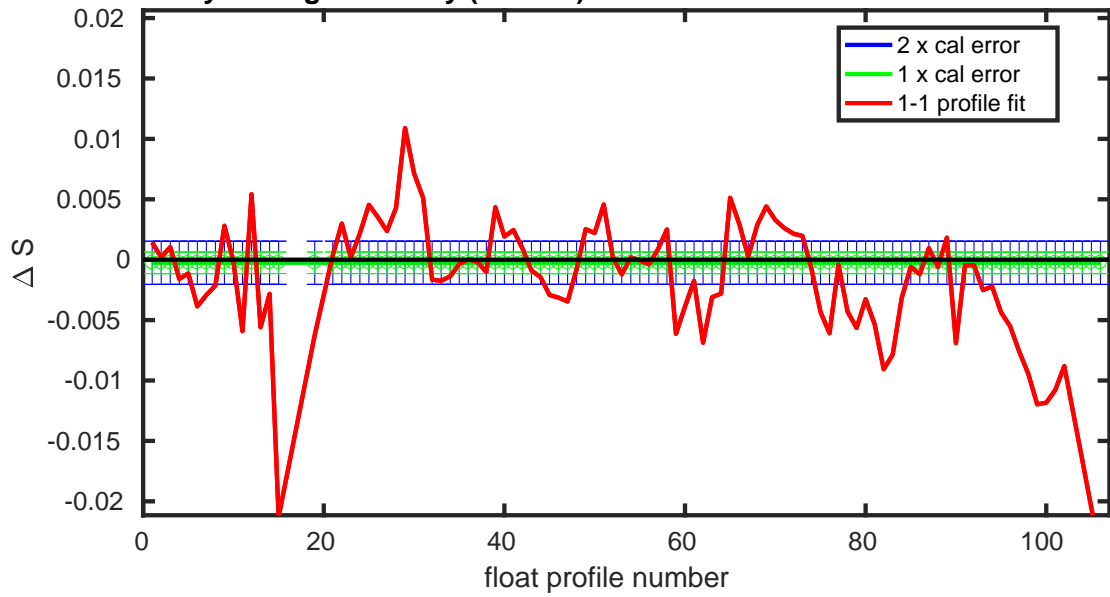
Figure 17: Float 3901888. Potential conductivity (top) and vertically averaged salinity (bottom) with errors.
