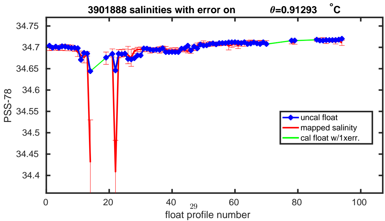
Figure 20: Float 3901888. Salinities with errors on \theta .
