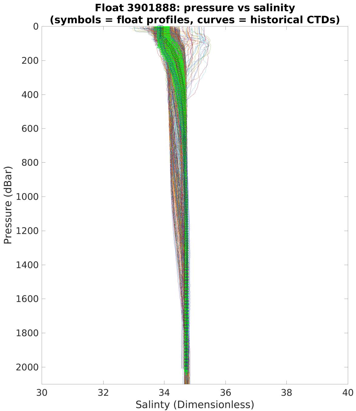
Figure 4: Float 3901888. Float profile of salinity (dimensionless) plotted with climatology from the spatial range of 10^\circ . The black and blue cycles indicates the first and the last Argo profile, respectively. Green symbols represent other Argo profiles.
