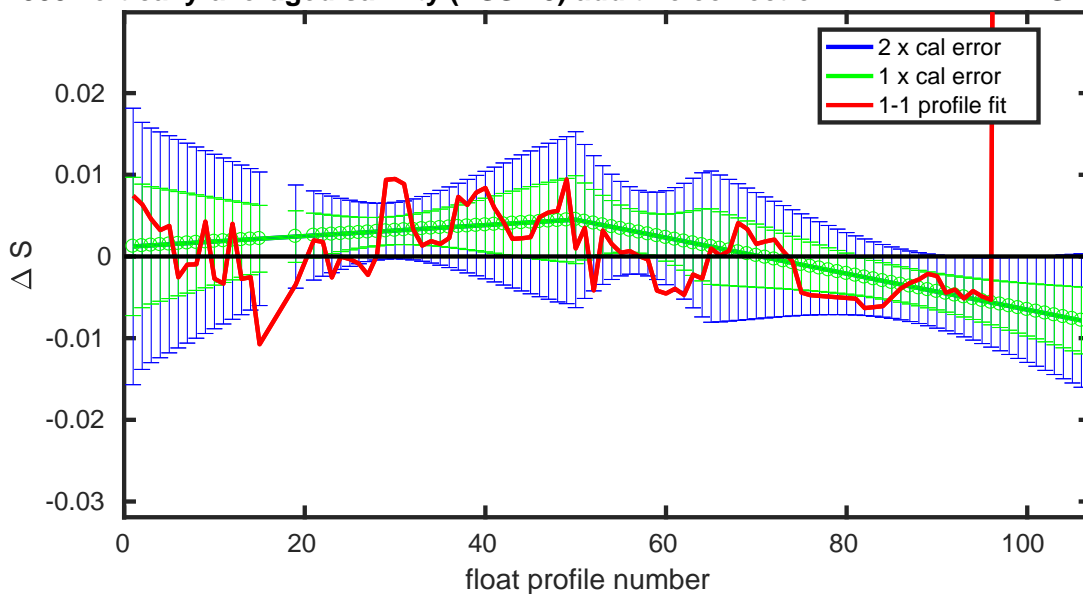
Figure 9: Float 3901888. Potential conductivity (top) and vertically averaged salinity (bottom) with errors.
