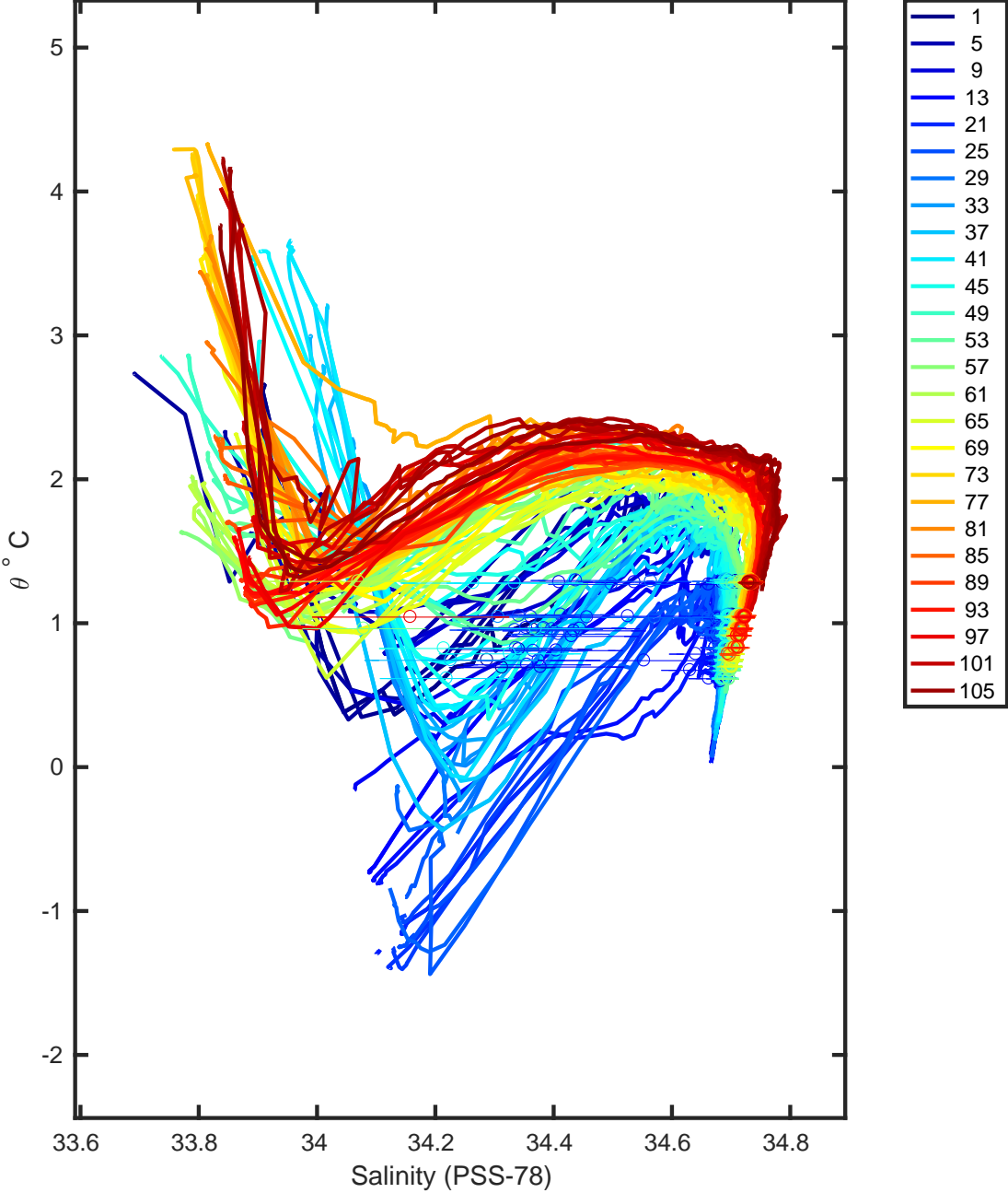
Figure 16: Float 3901888. Uncalibrated float data and mapped salinity.
