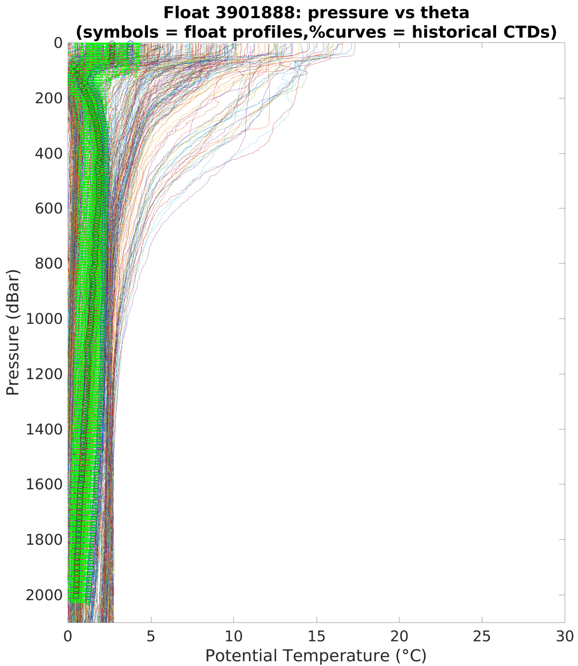
Figure 3: Float 3901888. Float profile of potential temperature (°C) plotted with climatology from the spatial range of 10°. The black and blue cycles indicates the first and the last Argo profile, respectively. Green symbols represent other Argo profiles.
