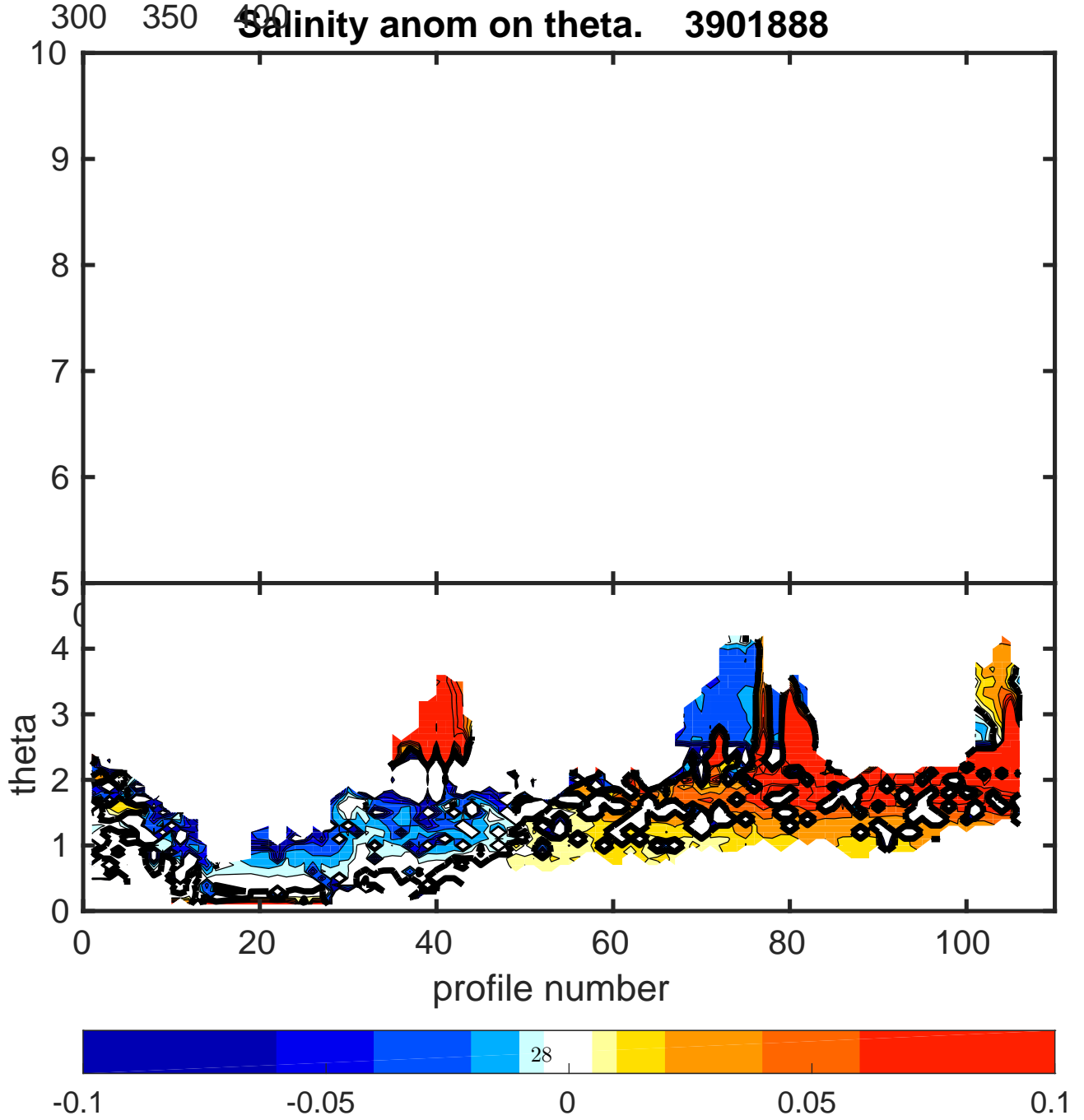
Figure 19: Float 3901888. Salinity anomaly on Theta
