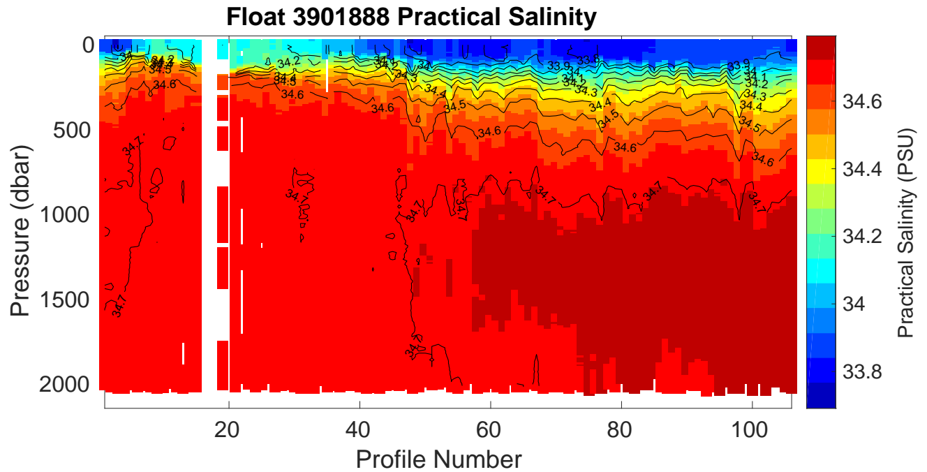
Figure 2: Float 3901888. Time series of the vertical distribution of practical salinity (PSU).
