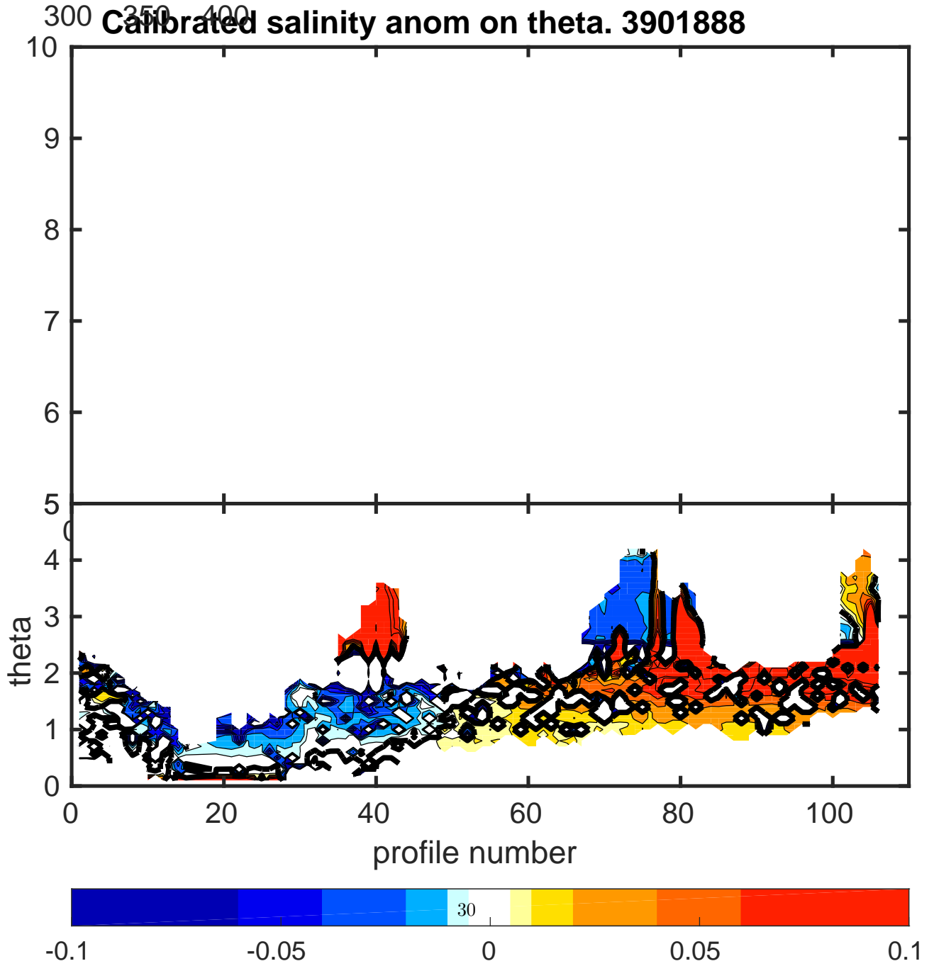
Figure 21: Float 3901888. Calibrated salinity anomaly on \theta .
