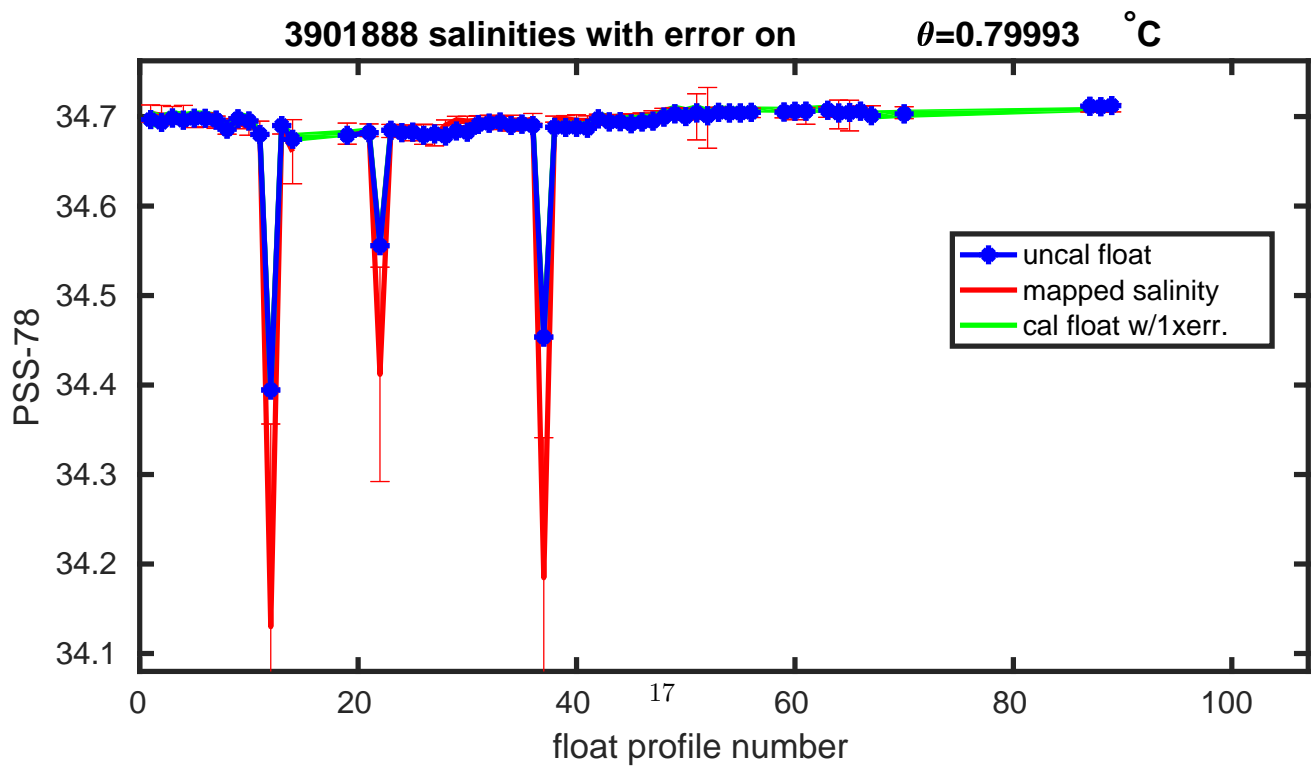
Figure 12: Float 3901888. Salinities with errors on \theta levels.
