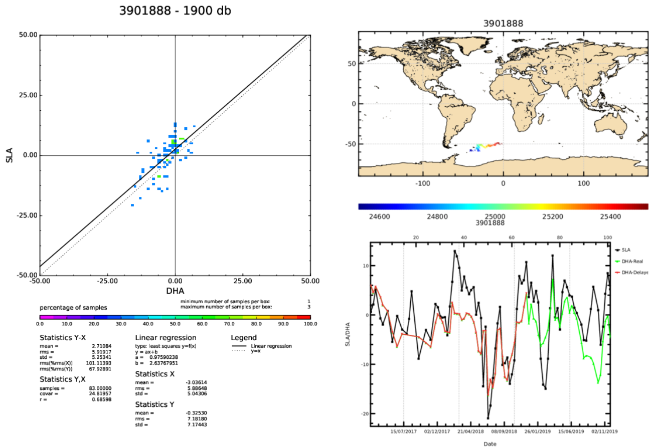
Figure 6: Float 3901888. The comparison between the Sea Surface Height (SSH) from the satellite altimetry and Dynamic Height Anomaly (DHA) extracted from the Argo float temperature and salinity data
