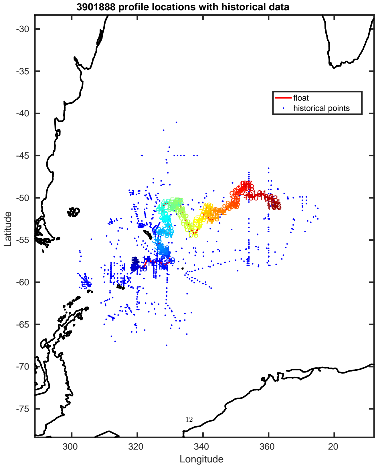
Figure 7: Float 3901888. Trajectory of the float with historical CTD data. The black contours indicate the bathymetry at 0, 200, 1000 and 2000 m.
