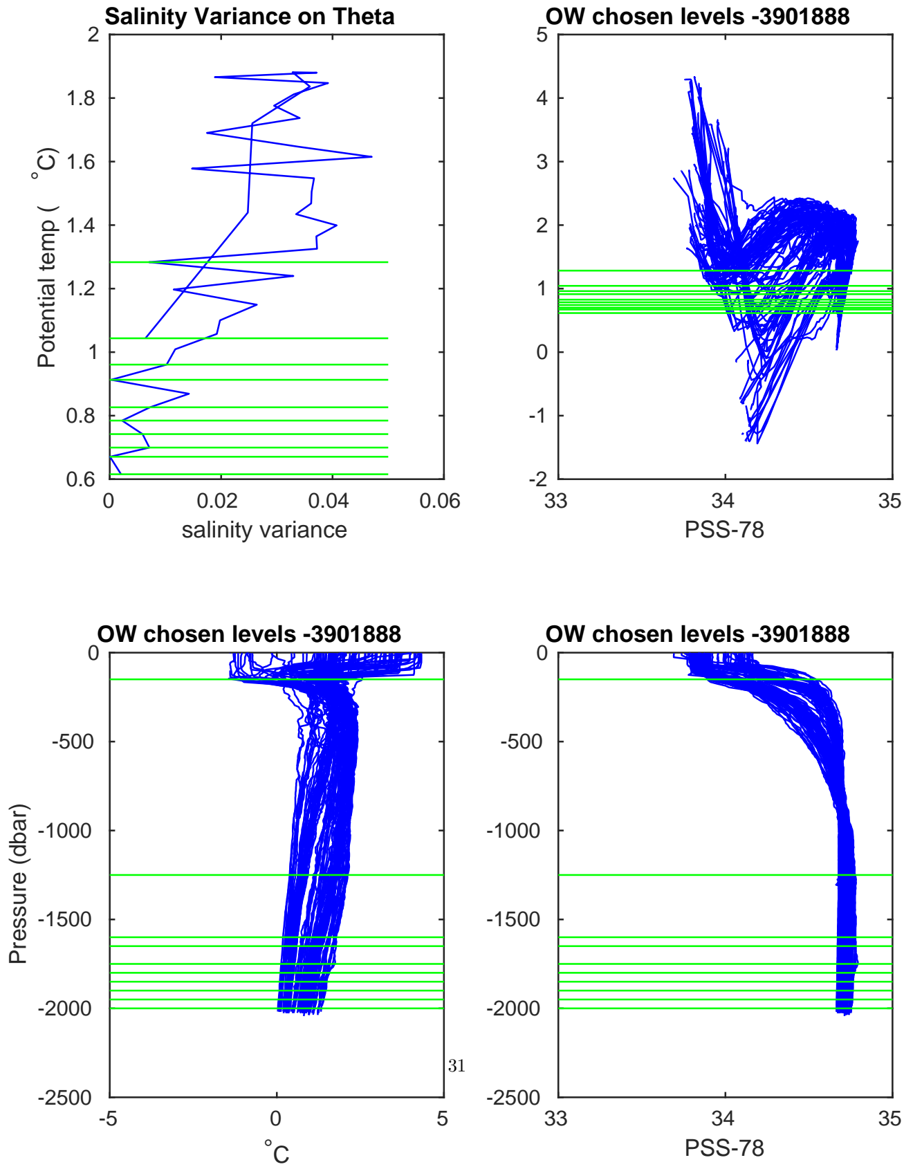
Figure 22: Float 3901888. Salinity, salinity variance on theta and OW chosen levels.
