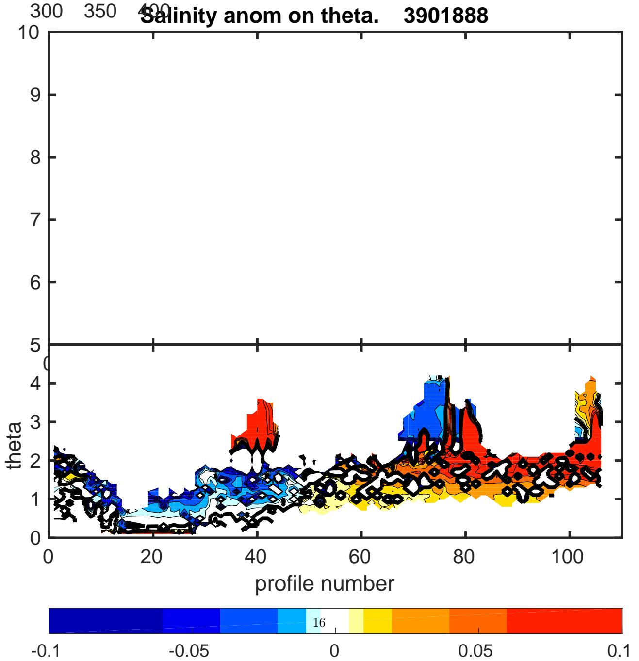
Figure 11: Float 3901888. Salinity anomaly on \theta levels.
