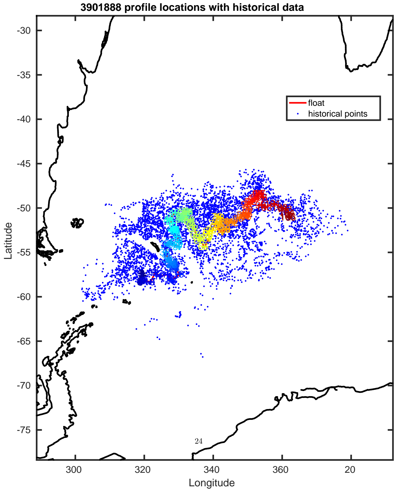
Figure 15: Float 3901888. Trajectory of the float with historical CTD data. The black contours indicate the bathymetry at 0, 200, 1000 and 2000 m.
