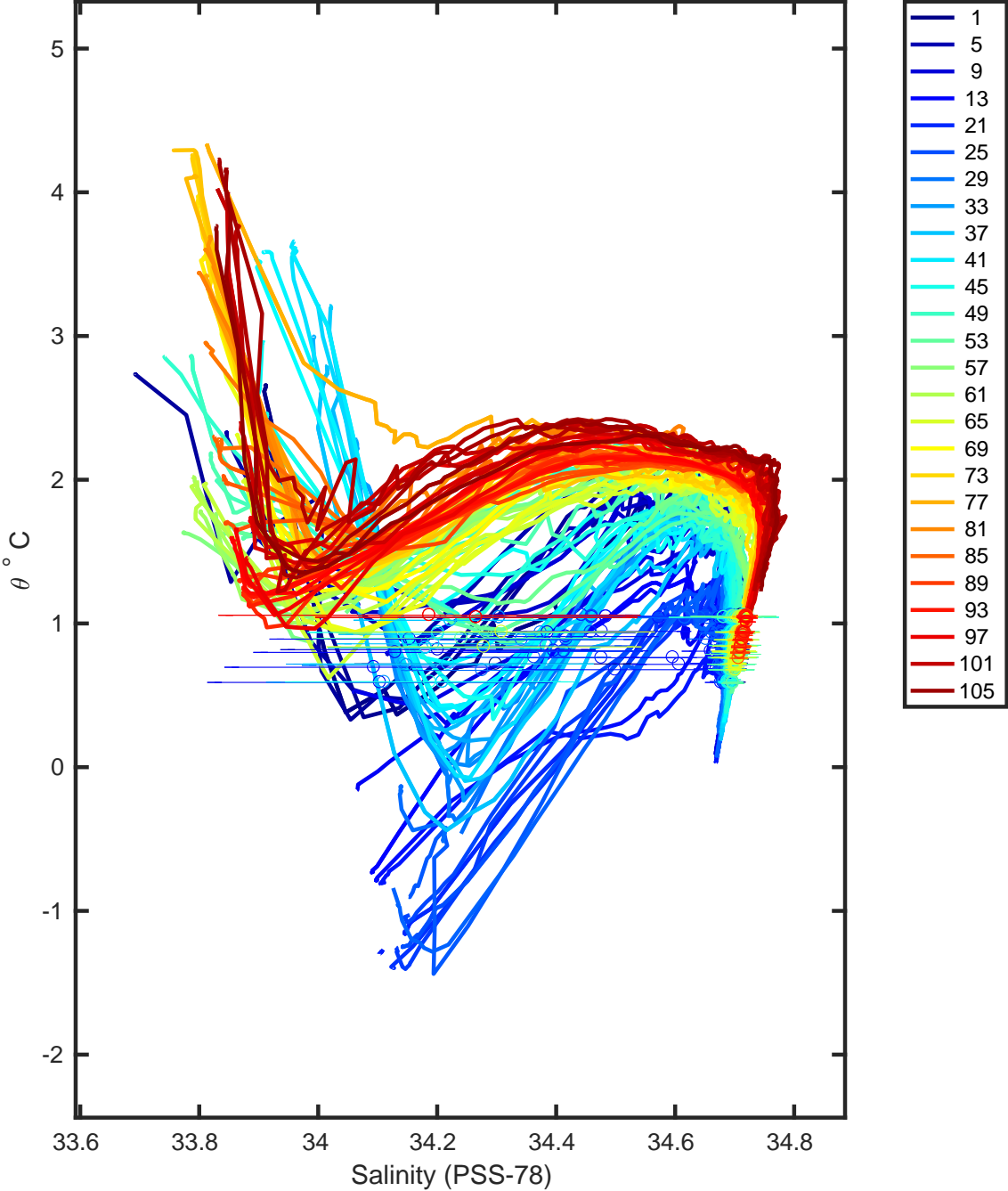
Figure 10: Float 3901888. Calibrated float data and mapped salinity.
