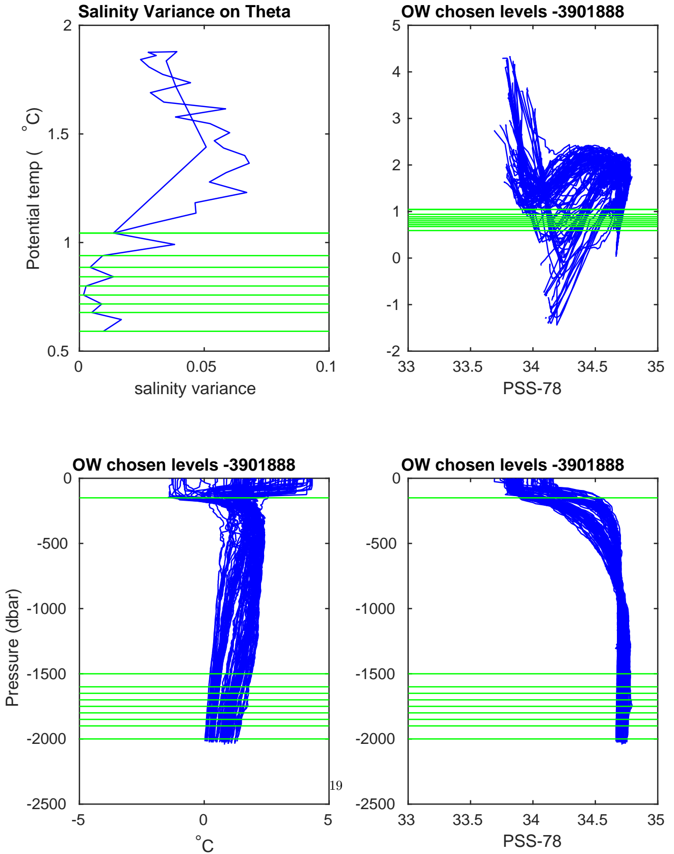
Figure 14: Float 3901888. Salinity, salinity variance on theta and OW chosen levels.
