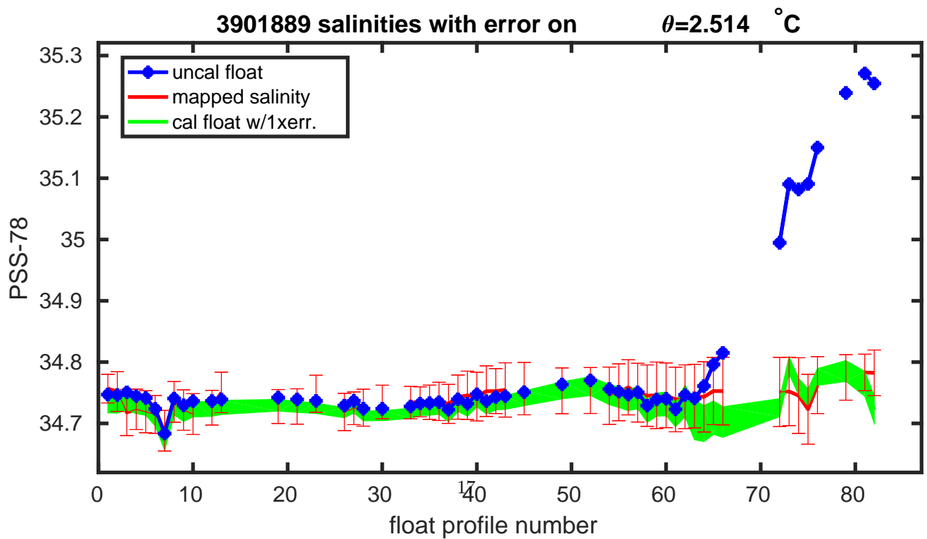
Figure 12: Float 3901889. Salinities with errors on \theta levels.
