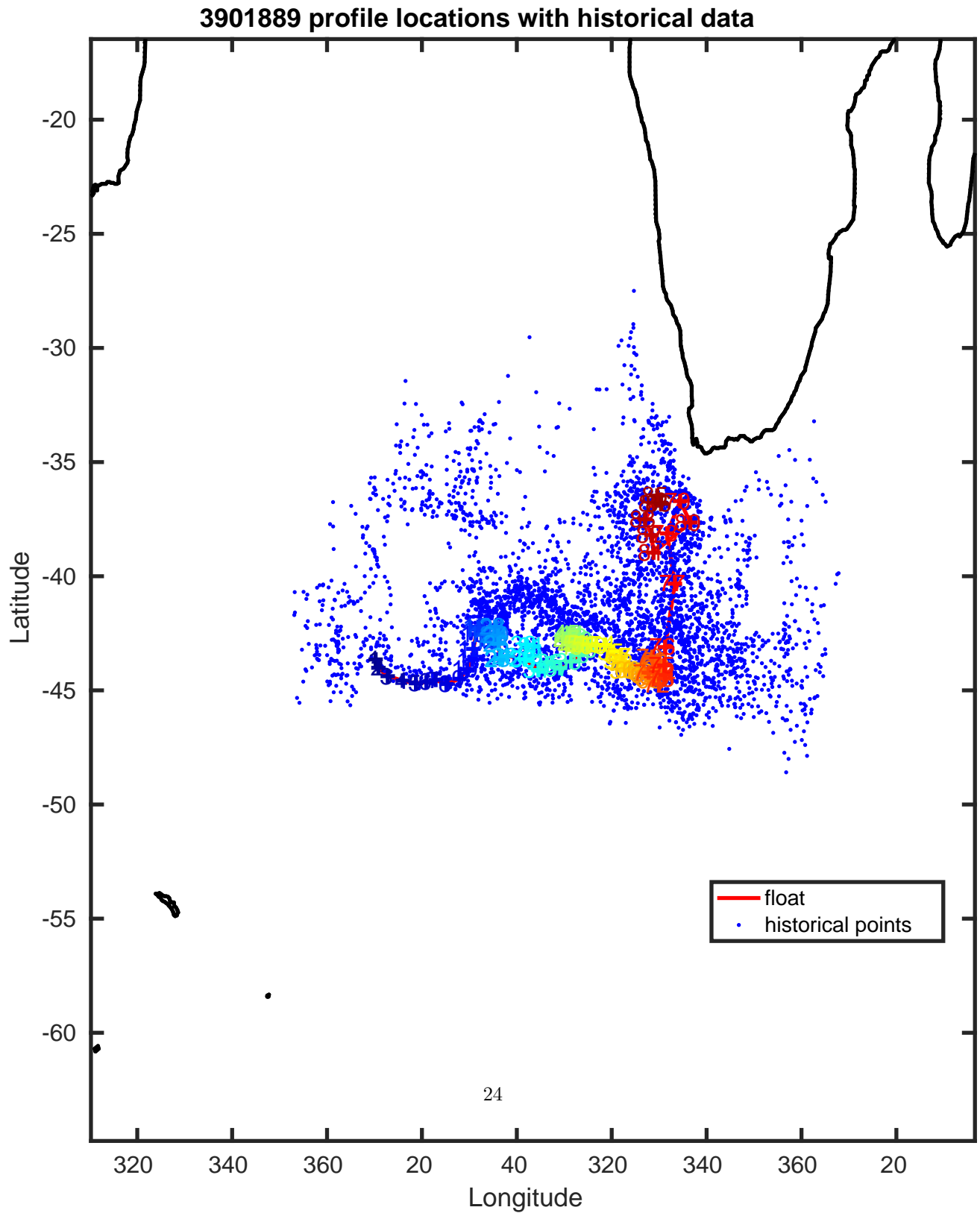
Figure 15: Float 3901889. Trajectory of the float with historical CTD data. The black contours indicate the bathymetry at 0, 200, 1000 and 2000 m.
