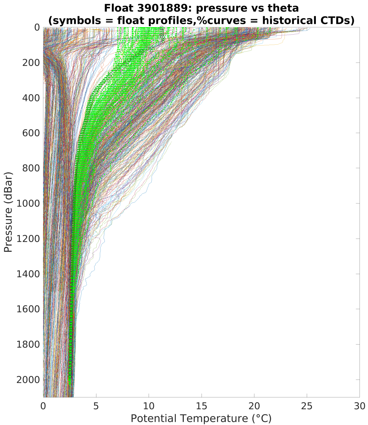
Figure 3: Float 3901889. Float profile of potential temperature (°C) plotted with climatology from the spatial range of 10 °. The black and blue cycles indicates the first and the last Argo profile, respectively. Green symbols represent other Argo profiles.
