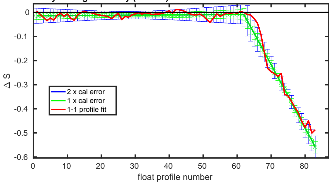
Figure 9: Float 3901889. Potential conductivity (top) and vertically averaged salinity (bottom) with errors.
