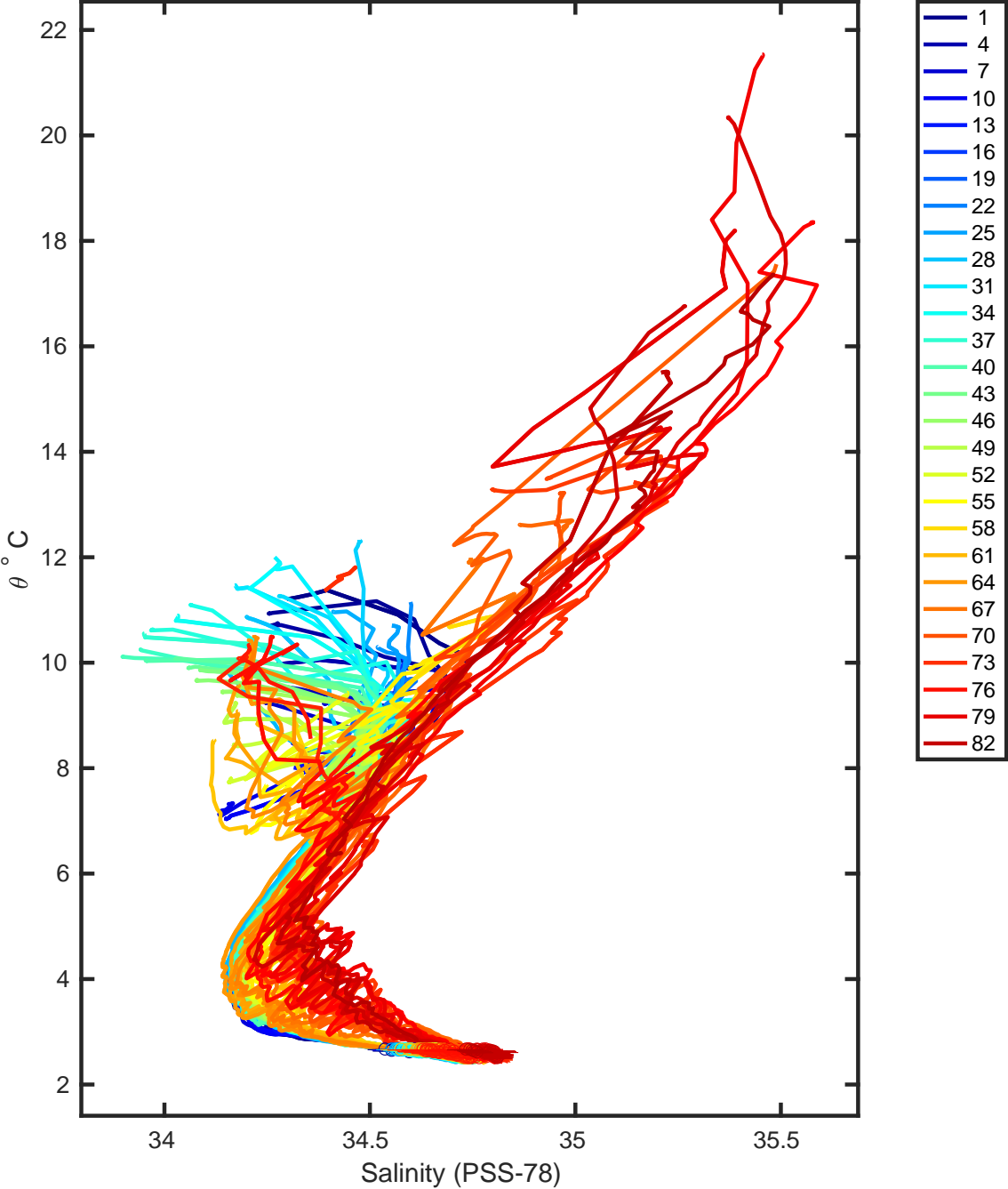
Figure 18: Float 3901889. Calibrated float data and mapped salinity.
