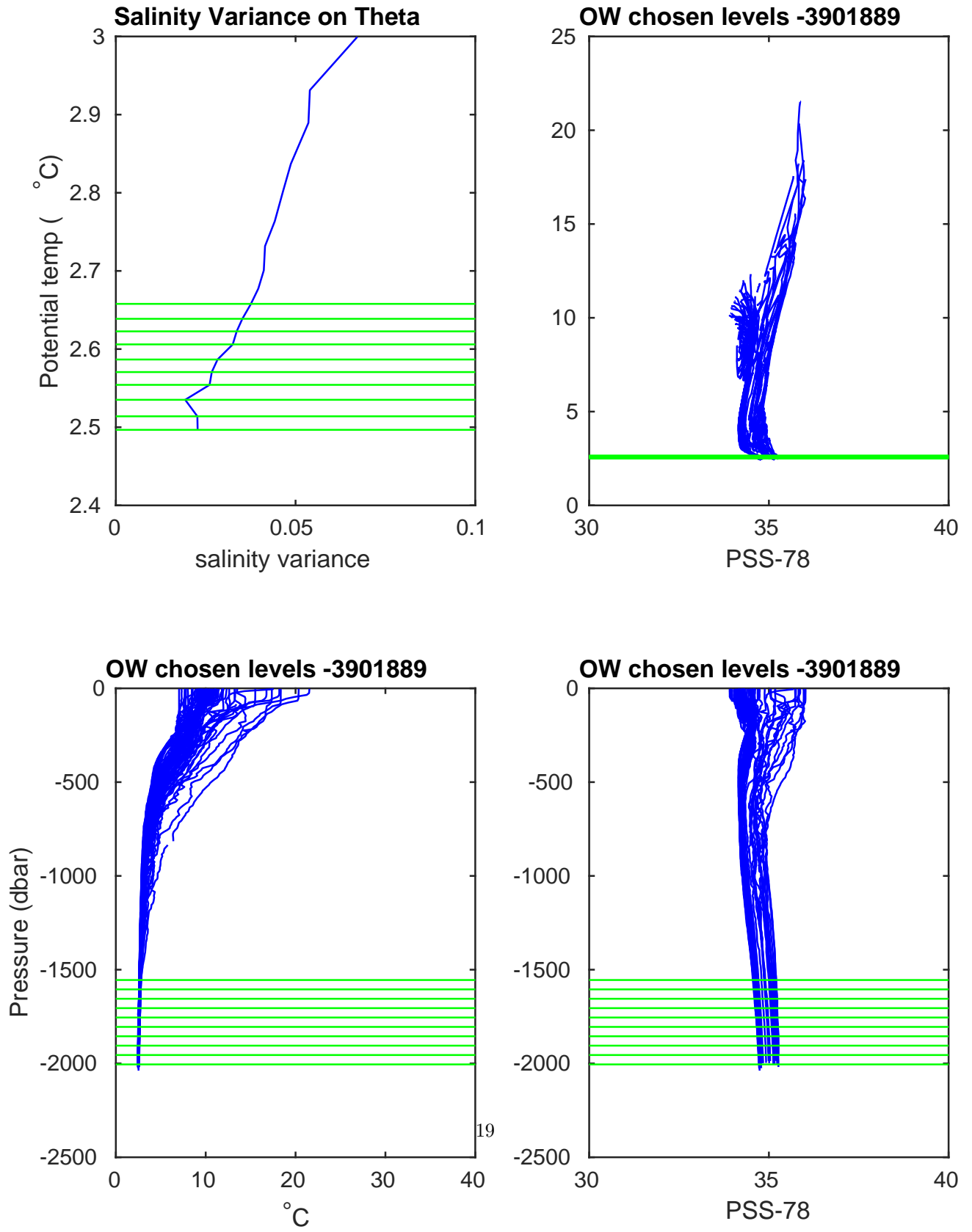
Figure 14: Float 3901889. Salinity, salinity variance on theta and OW chosen levels.
