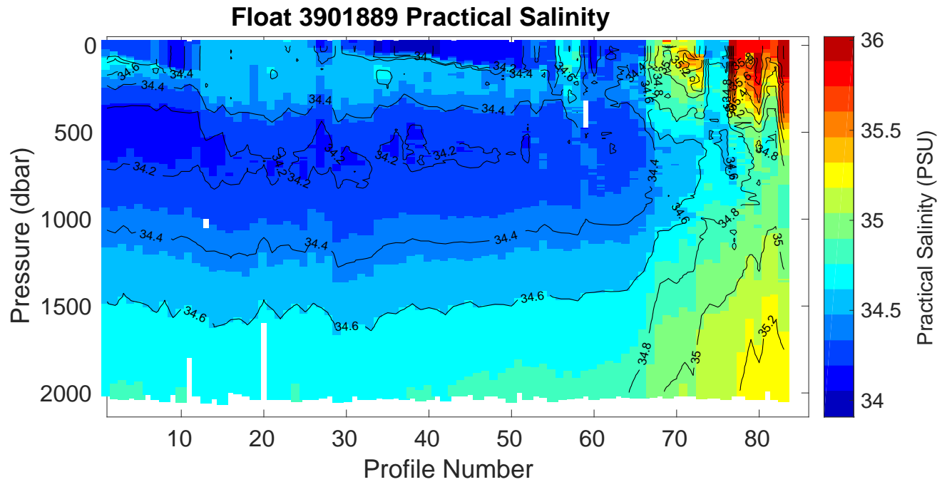
Figure 2: Float 3901889. Time series of the vertical distribution of practical salinity (PSU).
