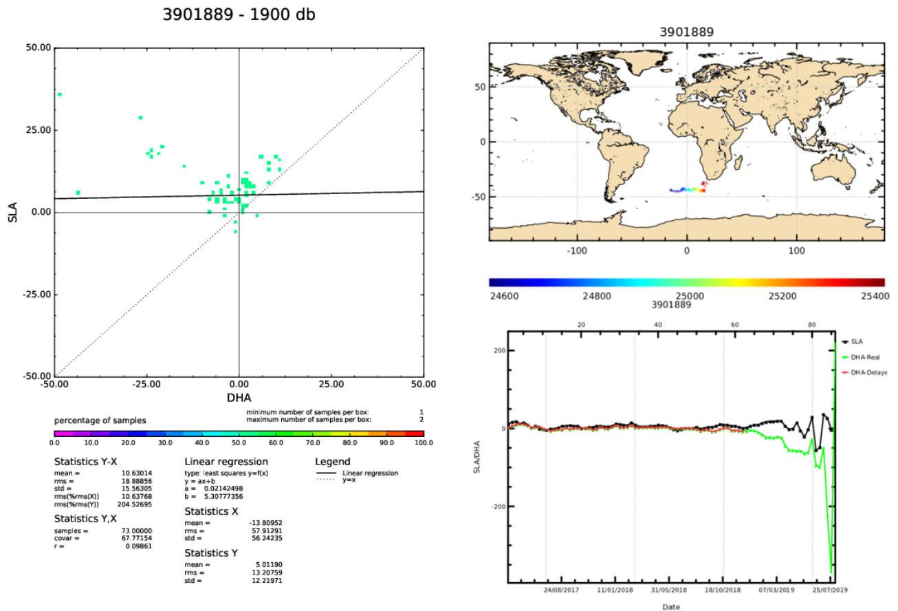
Figure 6: Float 3901889. The comparison between the Sea Surface Height (SSH) from the satellite altimetry and Dynamic Height Anomaly (DHA) extracted from the Argo float temperature and salinity data
