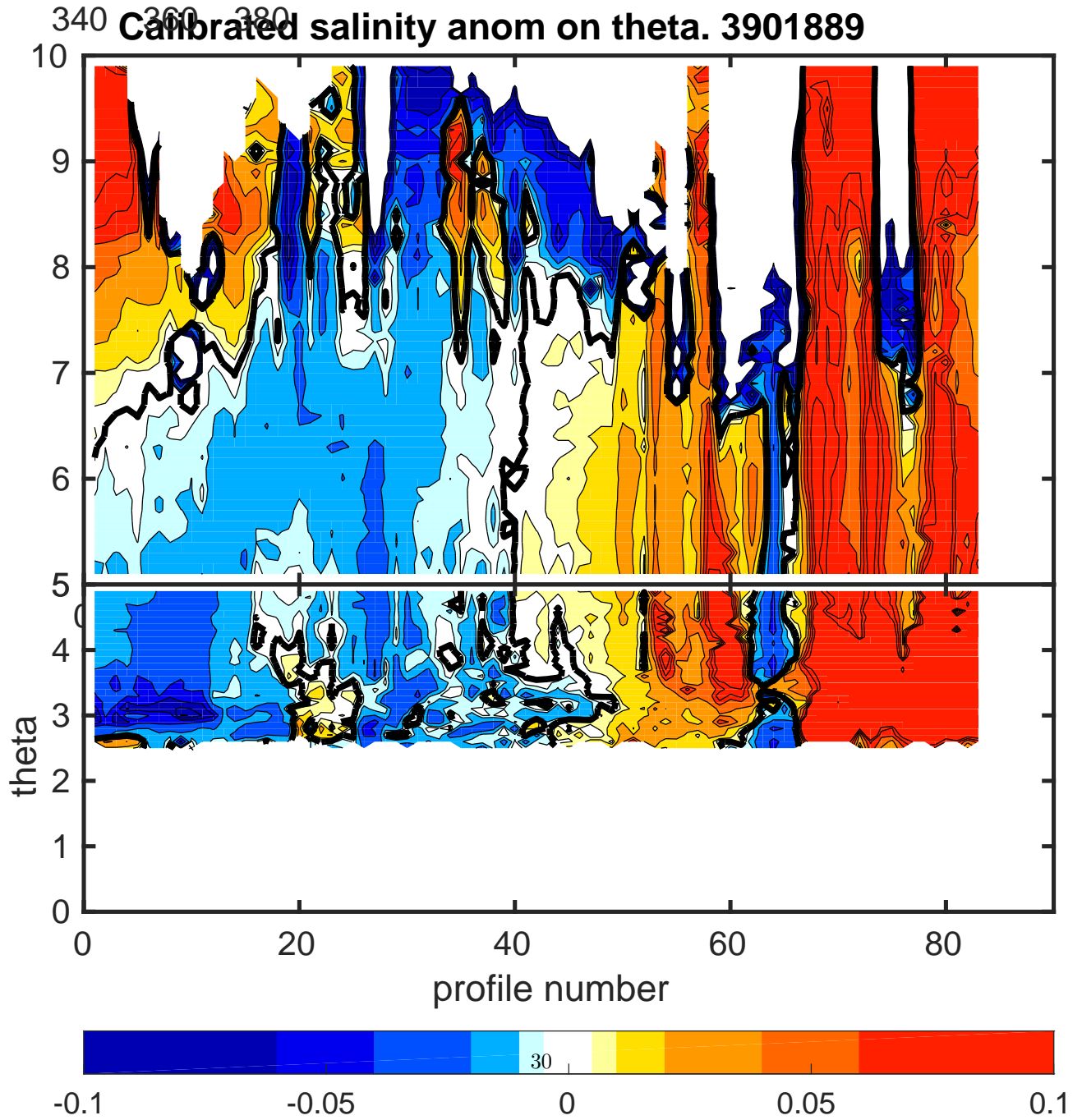
Figure 21: Float 3901889. Calibrated salinity anomaly on \theta .
