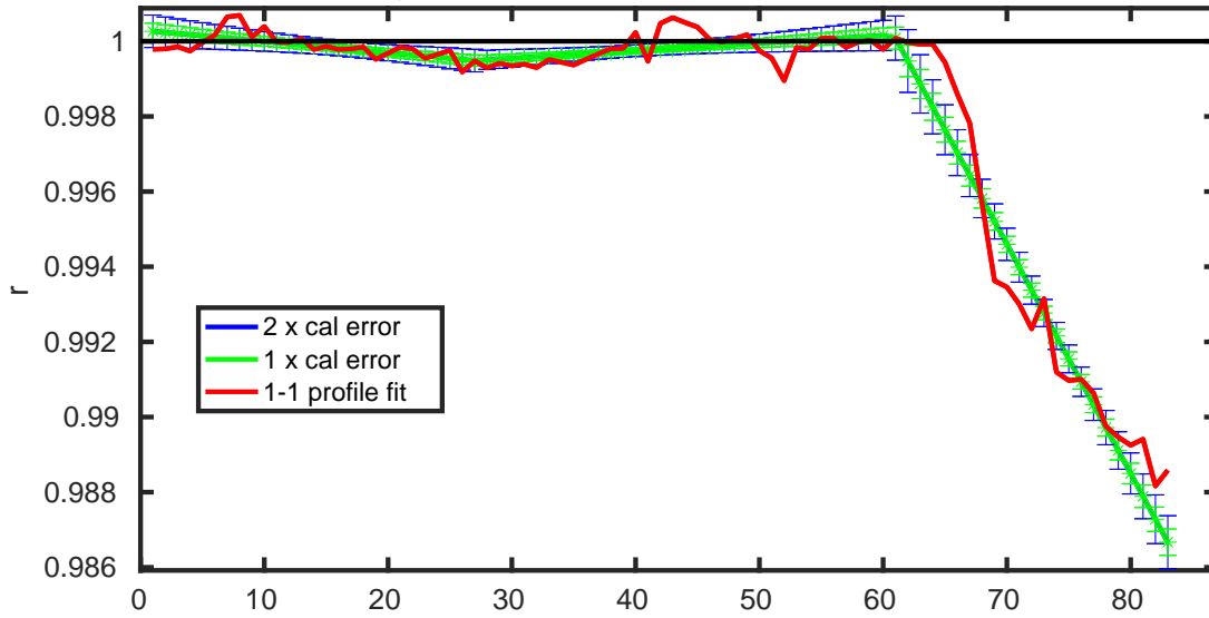
3901889 potential conductivity (mmho/cm) multiplicative correction r with errors
