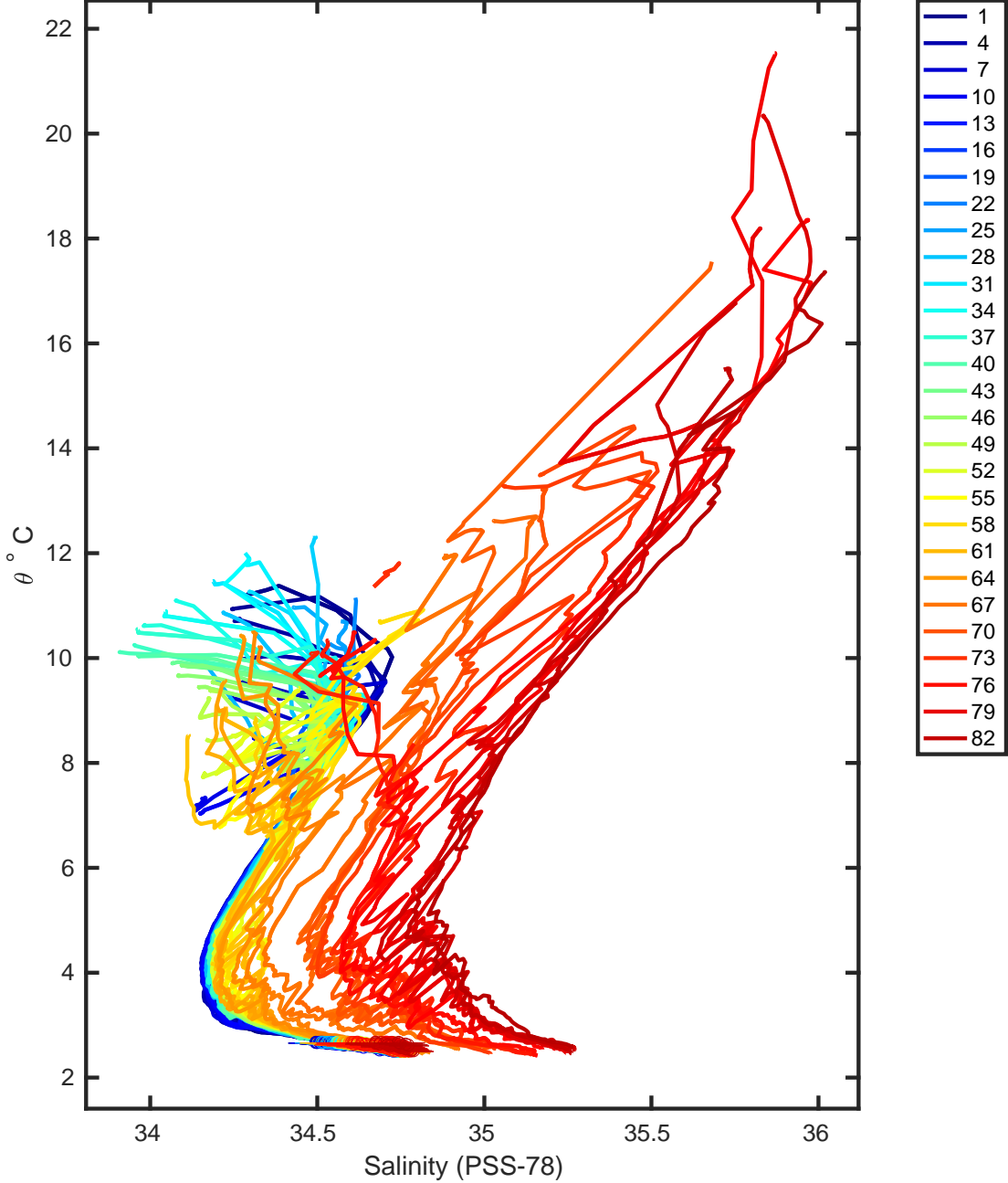
Figure 8: Float 3901889. Uncalibrated float data and mapped salinity.
