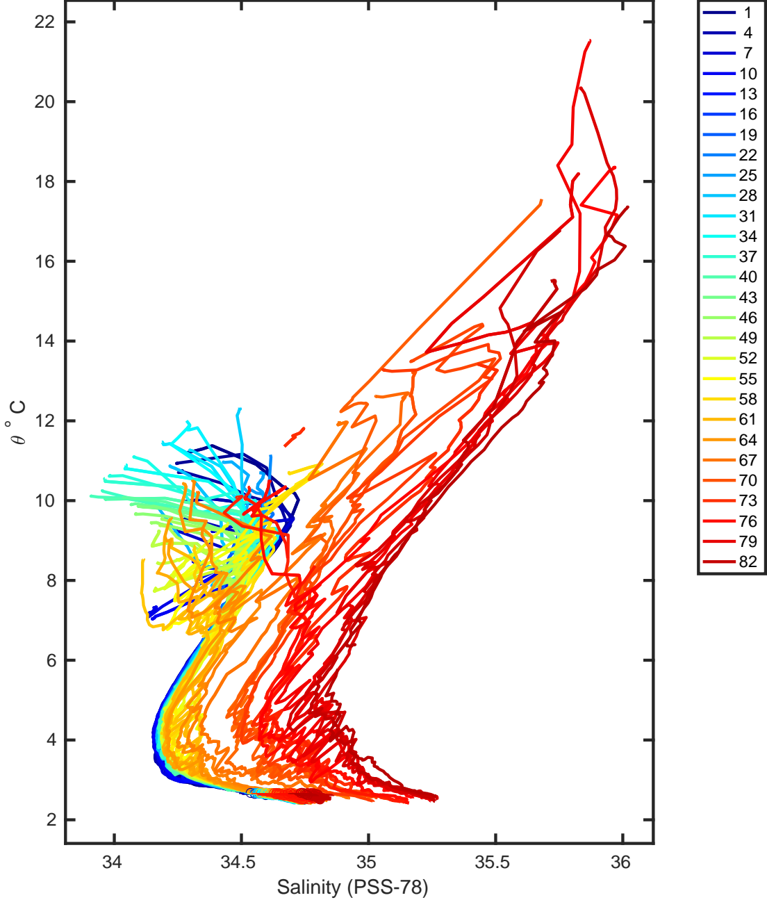
Figure 16: Float 3901889. Uncalibrated float data and mapped salinity.
