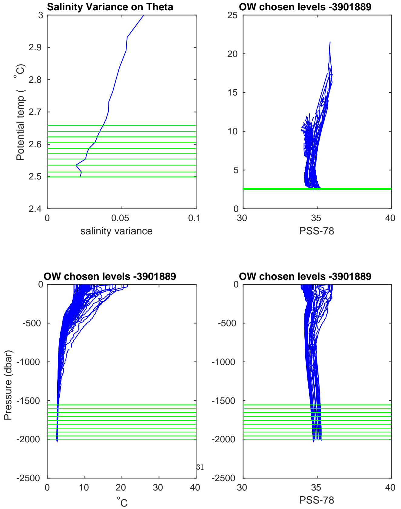
Figure 22: Float 3901889. Salinity, salinity variance on theta and OW chosen levels.
