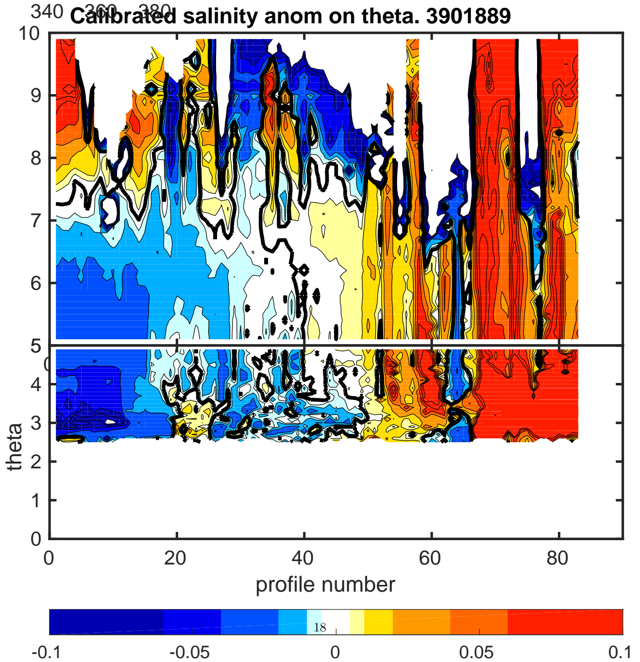
Figure 13: Float 3901889. Calibrated salinity anomaly on \theta levels.
