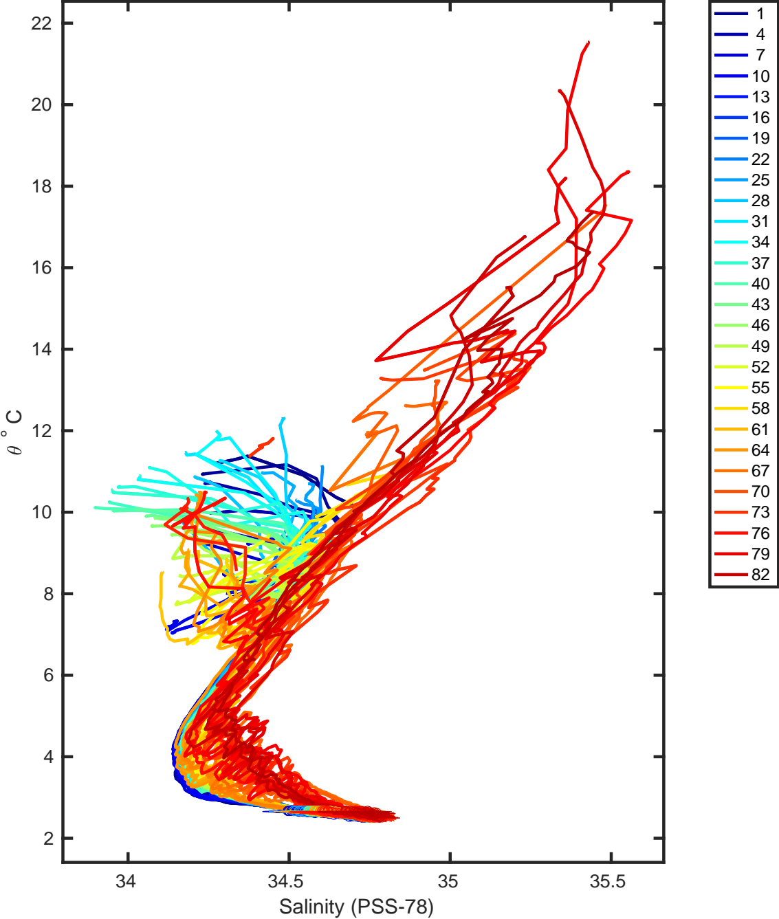
Figure 10: Float 3901889. Calibrated float data and mapped salinity.
