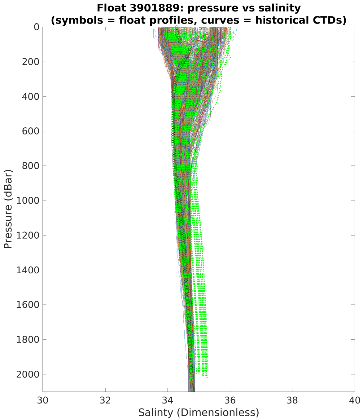
Figure 4: Float 3901889. Float profile of salinity (dimensionless) plotted with climatology from the spatial range of 10^\circ . The black and blue cycles indicates the first and the last Argo profile, respectively. Green symbols represent other Argo profiles.
