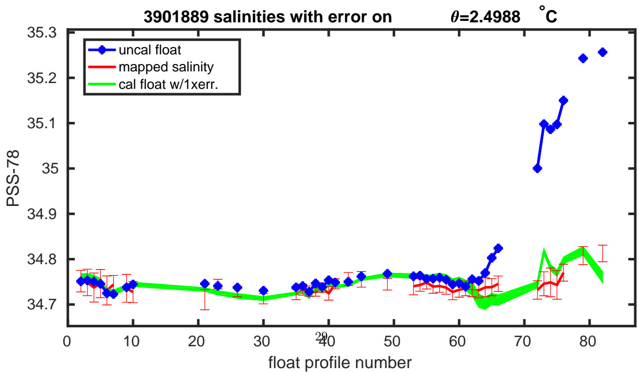
Figure 20: Float 3901889. Salinities with errors on \theta .
