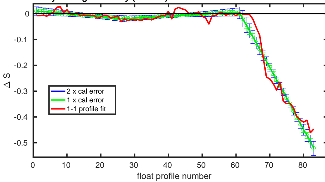
Figure 17: Float 3901889. Potential conductivity (top) and vertically averaged salinity (bottom) with errors.
