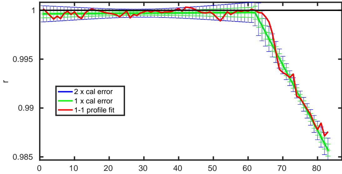
3901889 potential conductivity (mmho/cm) multiplicative correction r with errors
