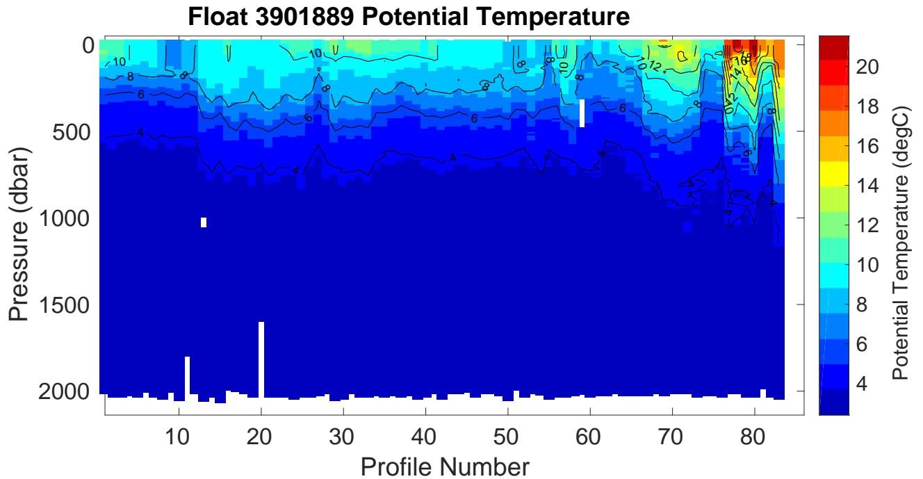
Figure 1: Float 3901889. Time series of the vertical distribution of potential temperature ( ^{\circ}\text{C} ).
