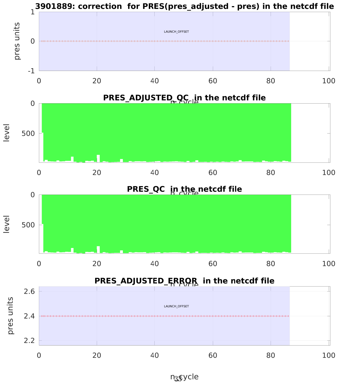
Figure 23: Float 3901889. Time series of applied pressure corrections.
