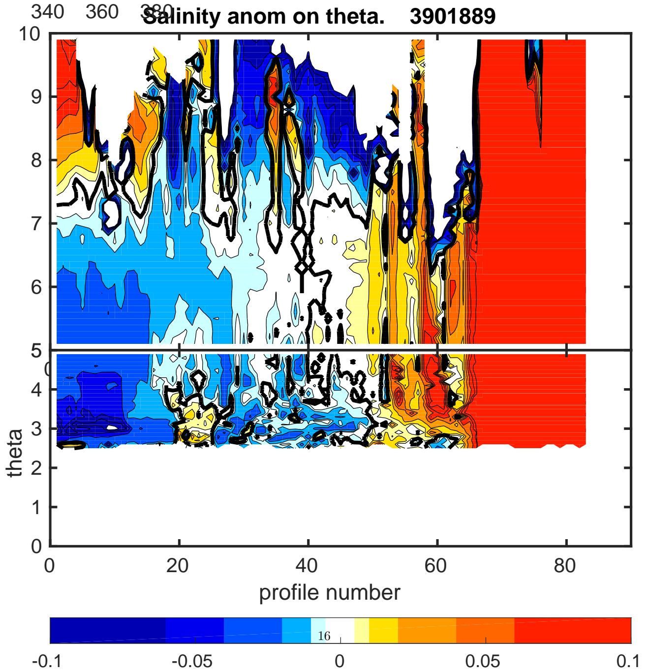
Figure 11: Float 3901889. Salinity anomaly on \theta levels.
