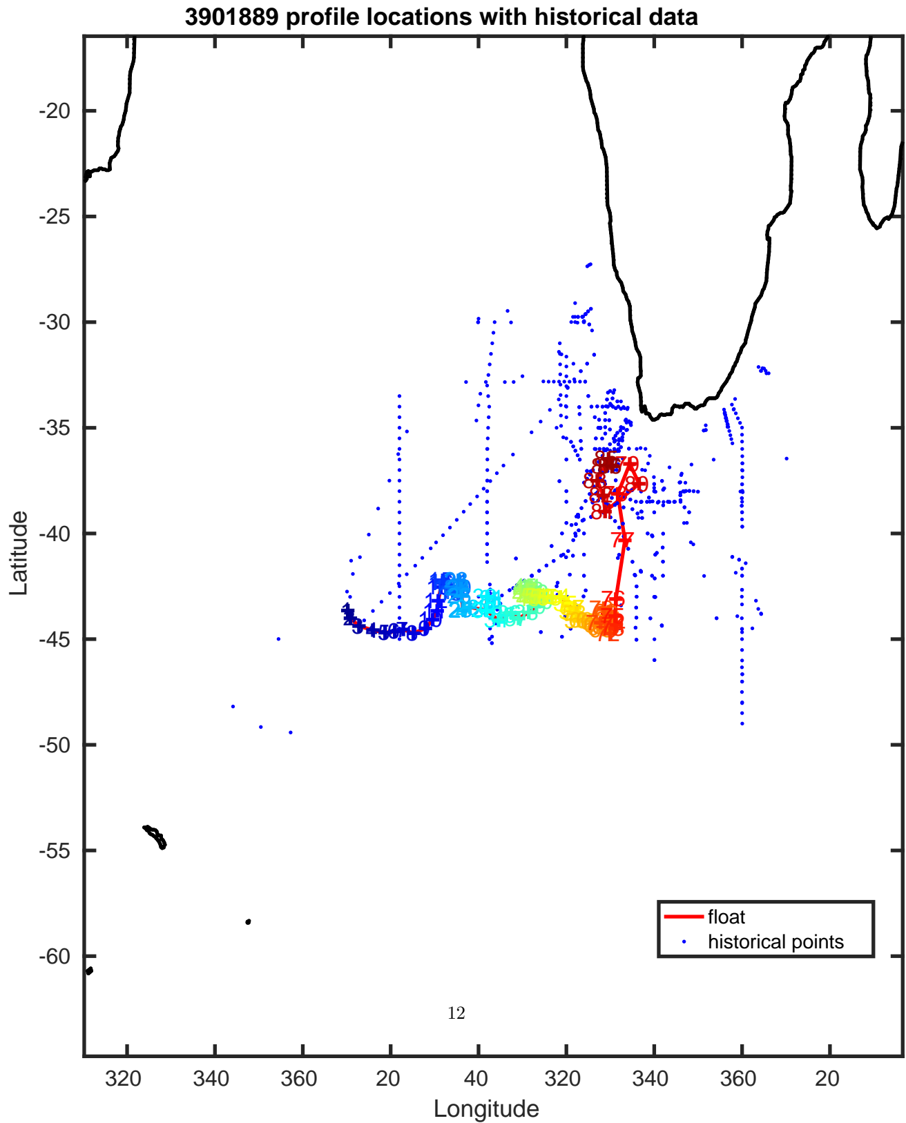
Figure 7: Float 3901889. Trajectory of the float with historical CTD data. The black contours indicate the bathymetry at 0, 200, 1000 and 2000 m.
