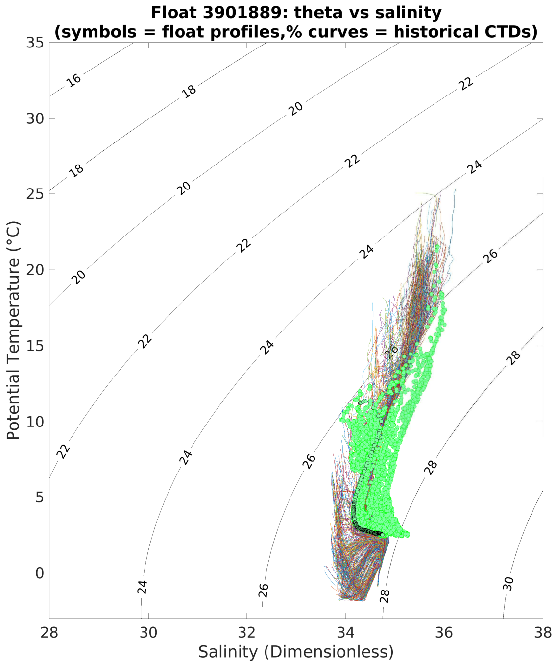
Figure 5: Float 3901889. Theta/S plotted with climatology from the spatial range of 10°. The black and blue cycles indicates the first and the last Argo profile, respectively. Green symbols represent other Argo profiles.
