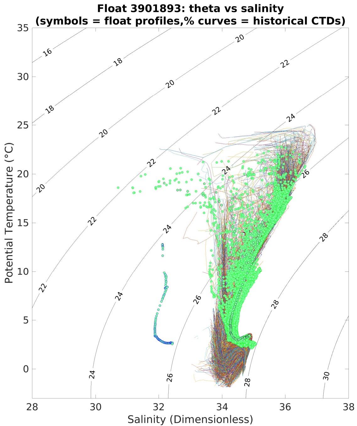
Figure 5: Float 3901893. Theta/S plotted with climatology from the spatial range of 10^{\circ} . The black and blue cycles indicates the first and the last Argo profile, respectively. Green symbols represent other Argo profiles.
