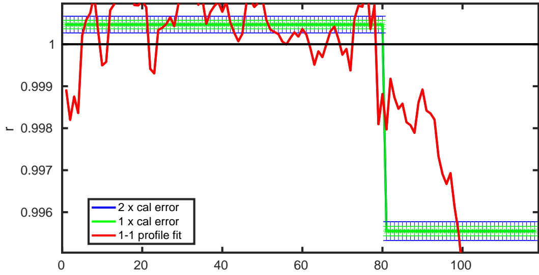
3901893 potential conductivity (mmho/cm) multiplicative correction r with errors
