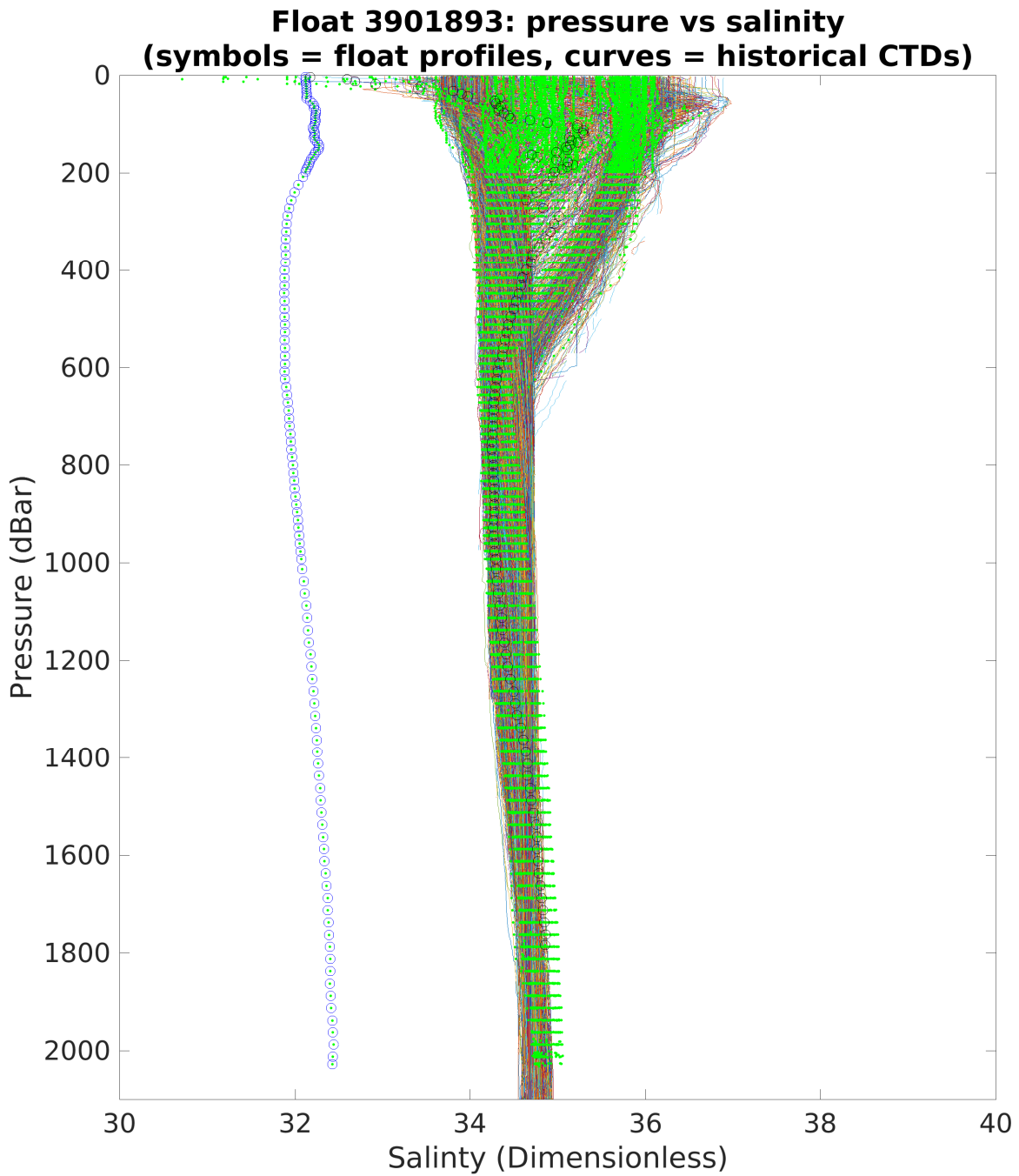
Figure 4: Float 3901893. Float profile of salinity (dimensionless) plotted with climatology from the spatial range of 10^\circ . The black and blue cycles indicates the first and the last Argo profile, respectively. Green symbols represent other Argo profiles.
