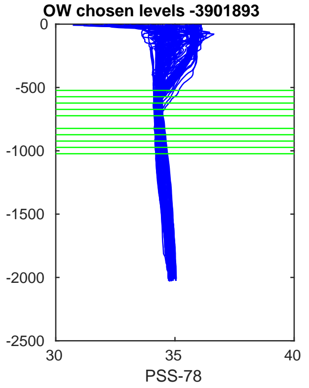
Figure 22: Float 3901893. Salinity, salinity variance on theta and OW chosen levels.
