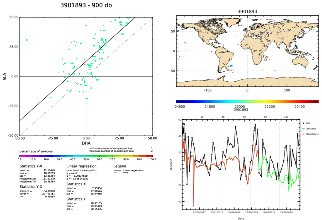
Figure 6: Float 3901893. The comparison between the Sea Surface Height (SSH) from the satellite altimetry and Dynamic Height Anomaly (DHA) extracted from the Argo float temperature and salinity data
