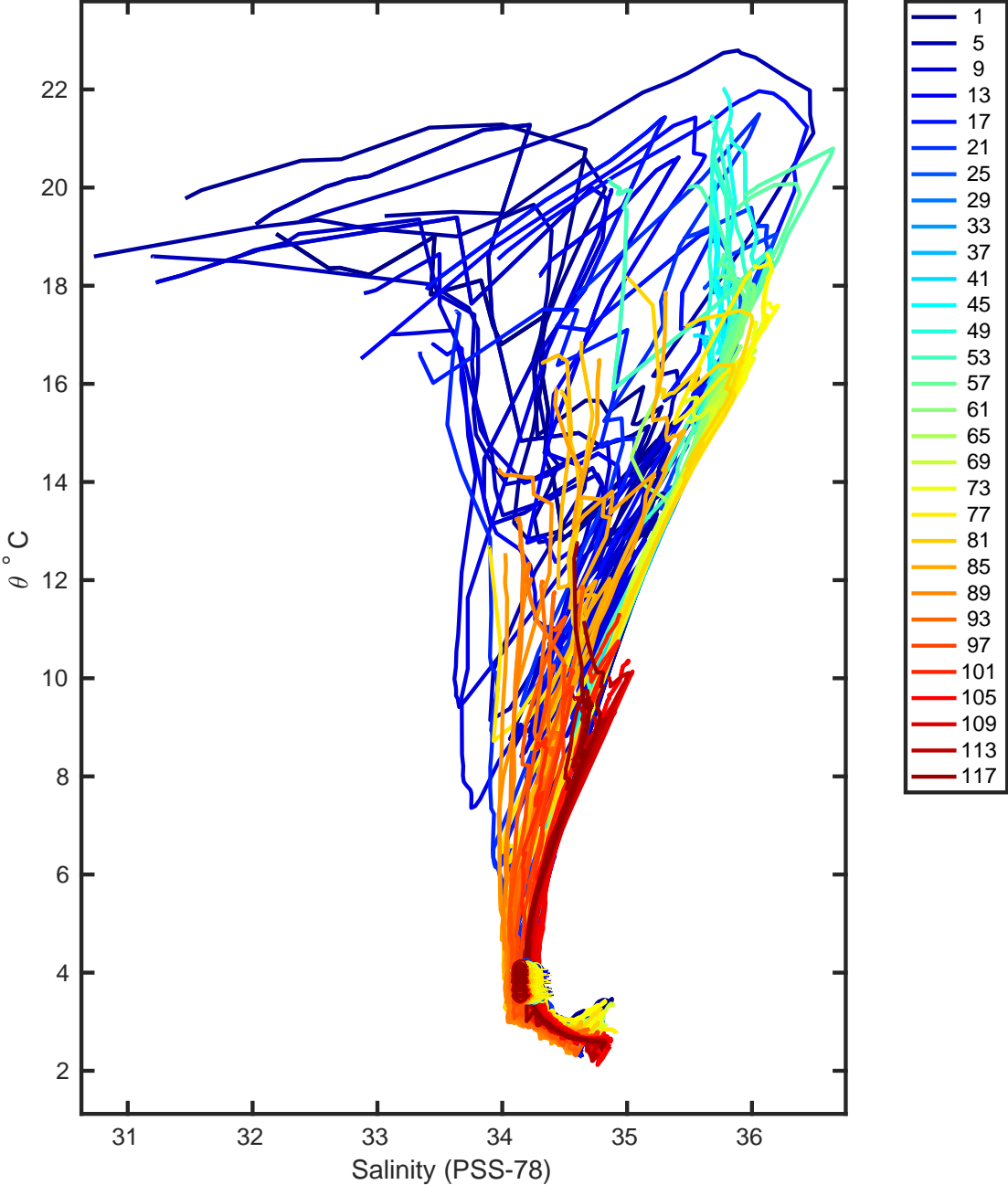
Figure 18: Float 3901893. Calibrated float data and mapped salinity.
