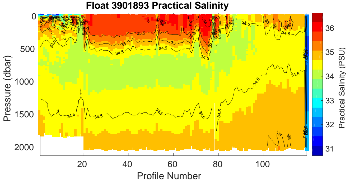
Figure 2: Float 3901893. Time series of the vertical distribution of practical salinity (PSU).
