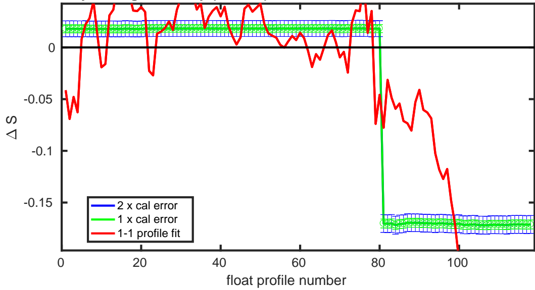
Figure 17: Float 3901893. Potential conductivity (top) and vertically averaged salinity (bottom) with errors.
