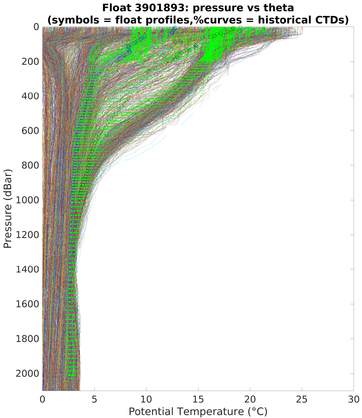
Figure 3: Float 3901893. Float profile of potential temperature (°C) plotted with climatology from the spatial range of 10 °. The black and blue cycles indicates the first and the last Argo profile, respectively. Green symbols represent other Argo profiles.
