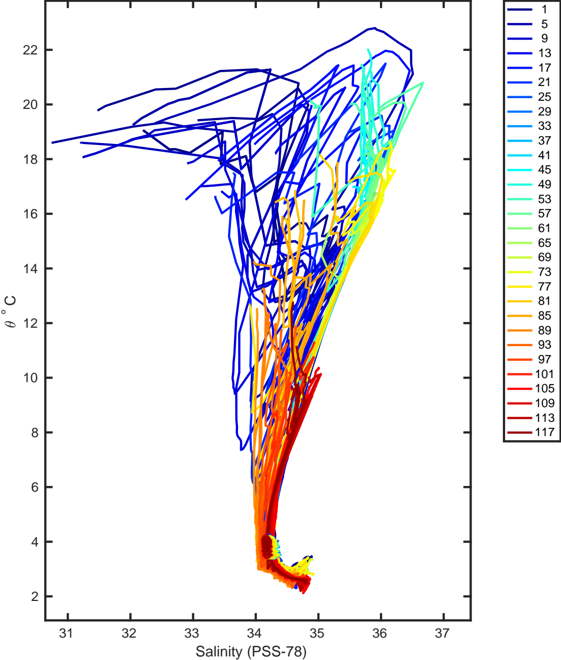
Figure 10: Float 3901893. Calibrated float data and mapped salinity.
