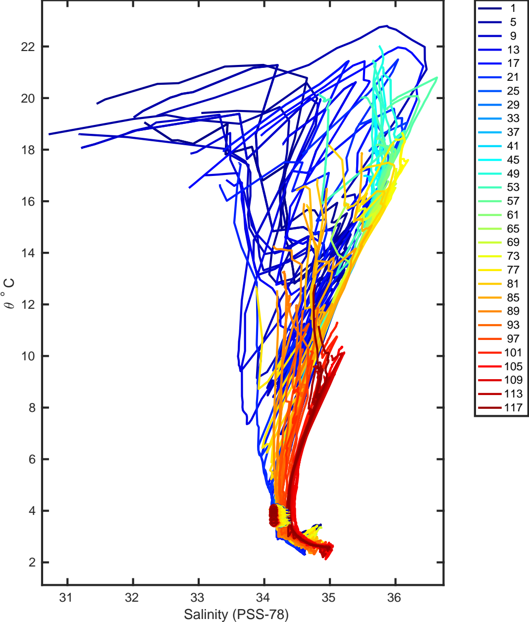
Figure 16: Float 3901893. Uncalibrated float data and mapped salinity.
