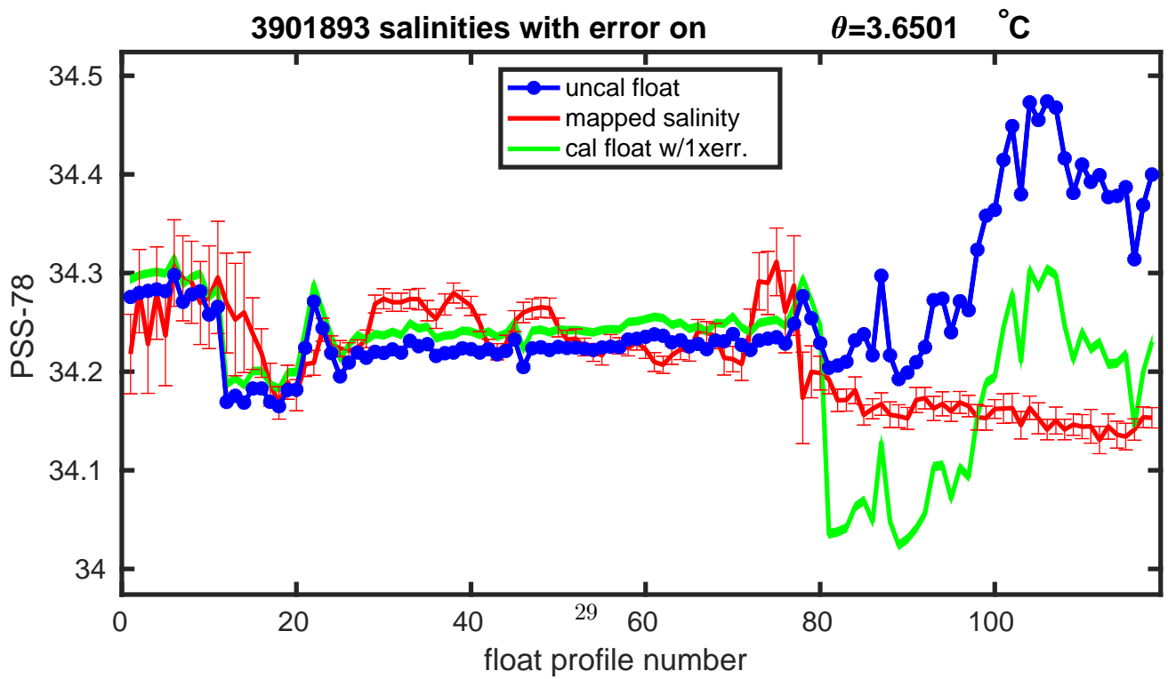
Figure 20: Float 3901893. Salinities with errors on \theta .
