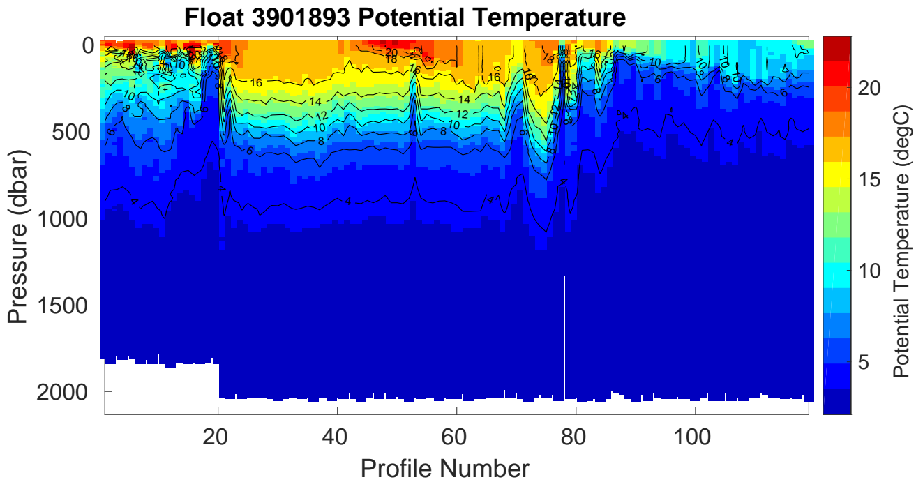
Figure 1: Float 3901893. Time series of the vertical distribution of potential temperature ( ^{\circ}\text{C} ).
