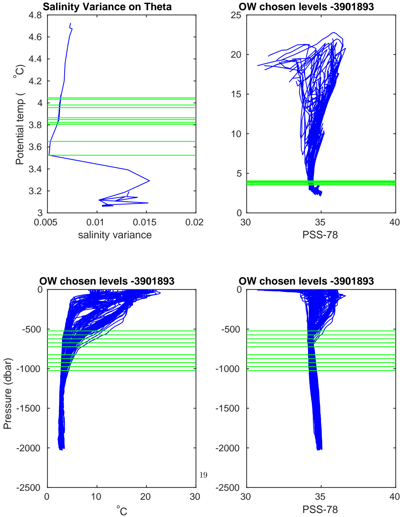
Figure 14: Float 3901893. Salinity, salinity variance on theta and OW chosen levels.
