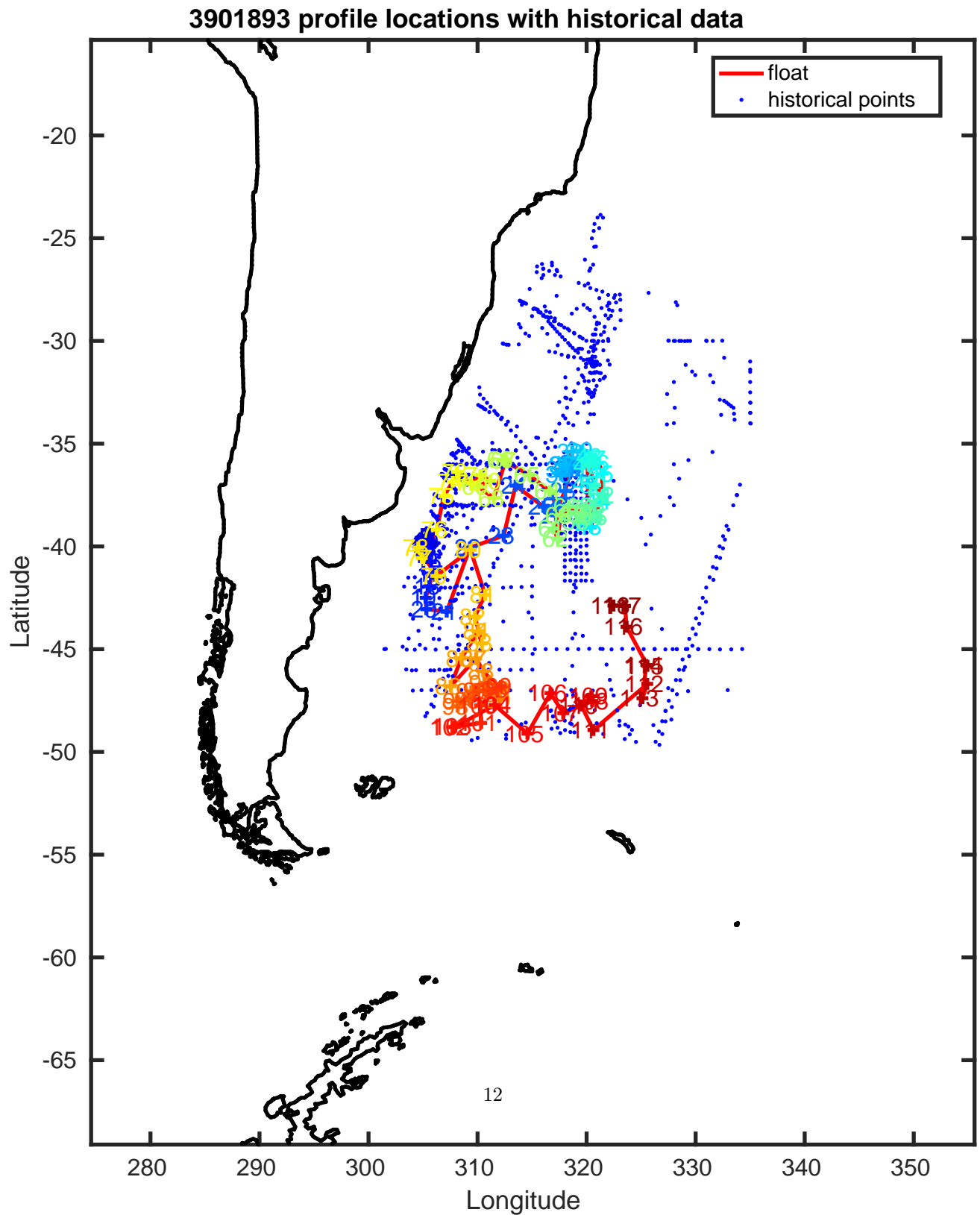
Figure 7: Float 3901893. Trajectory of the float with historical CTD data. The black contours indicate the bathymetry at 0, 200, 1000 and 2000 m.
