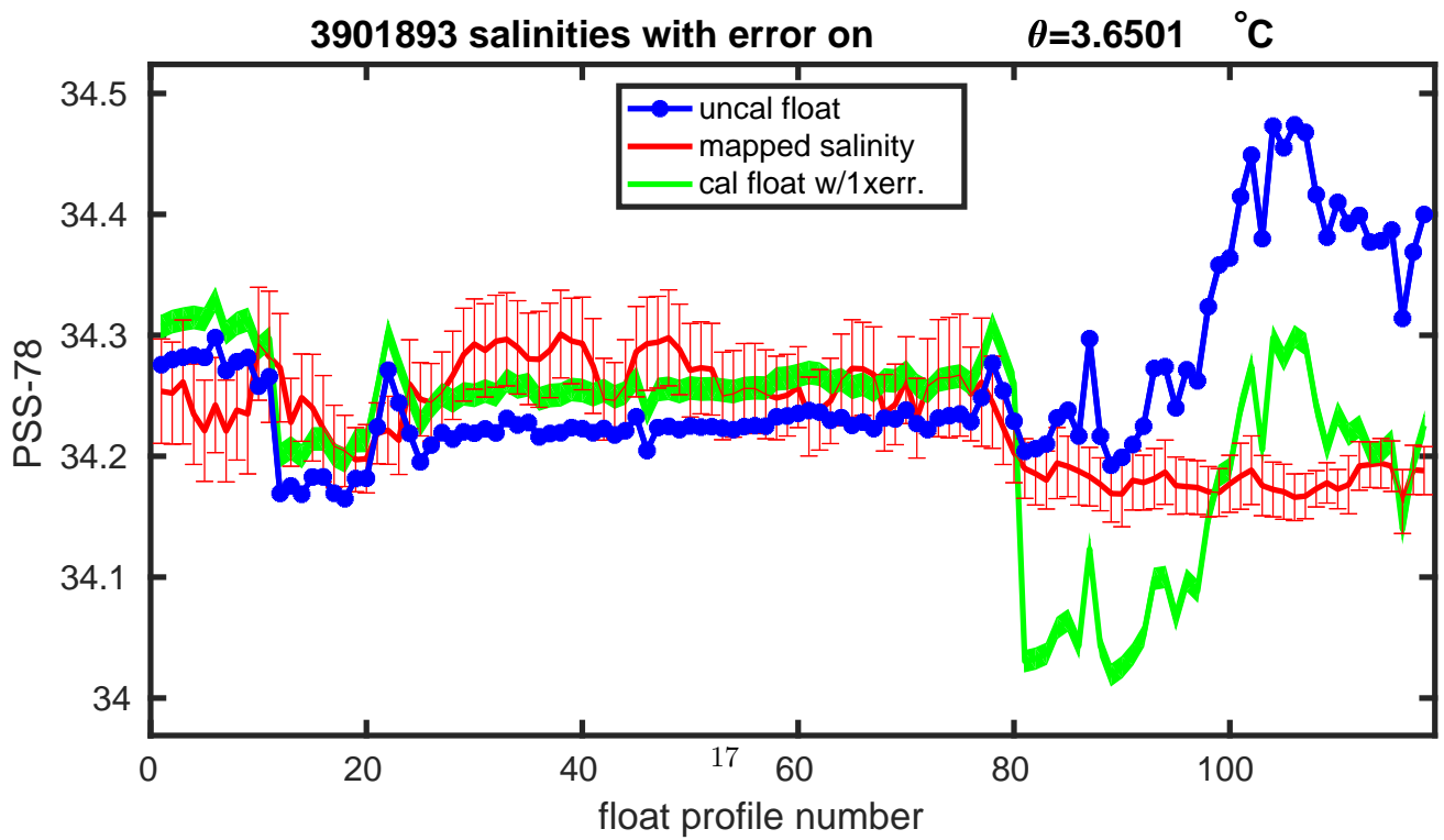
Figure 12: Float 3901893. Salinities with errors on \theta levels.
