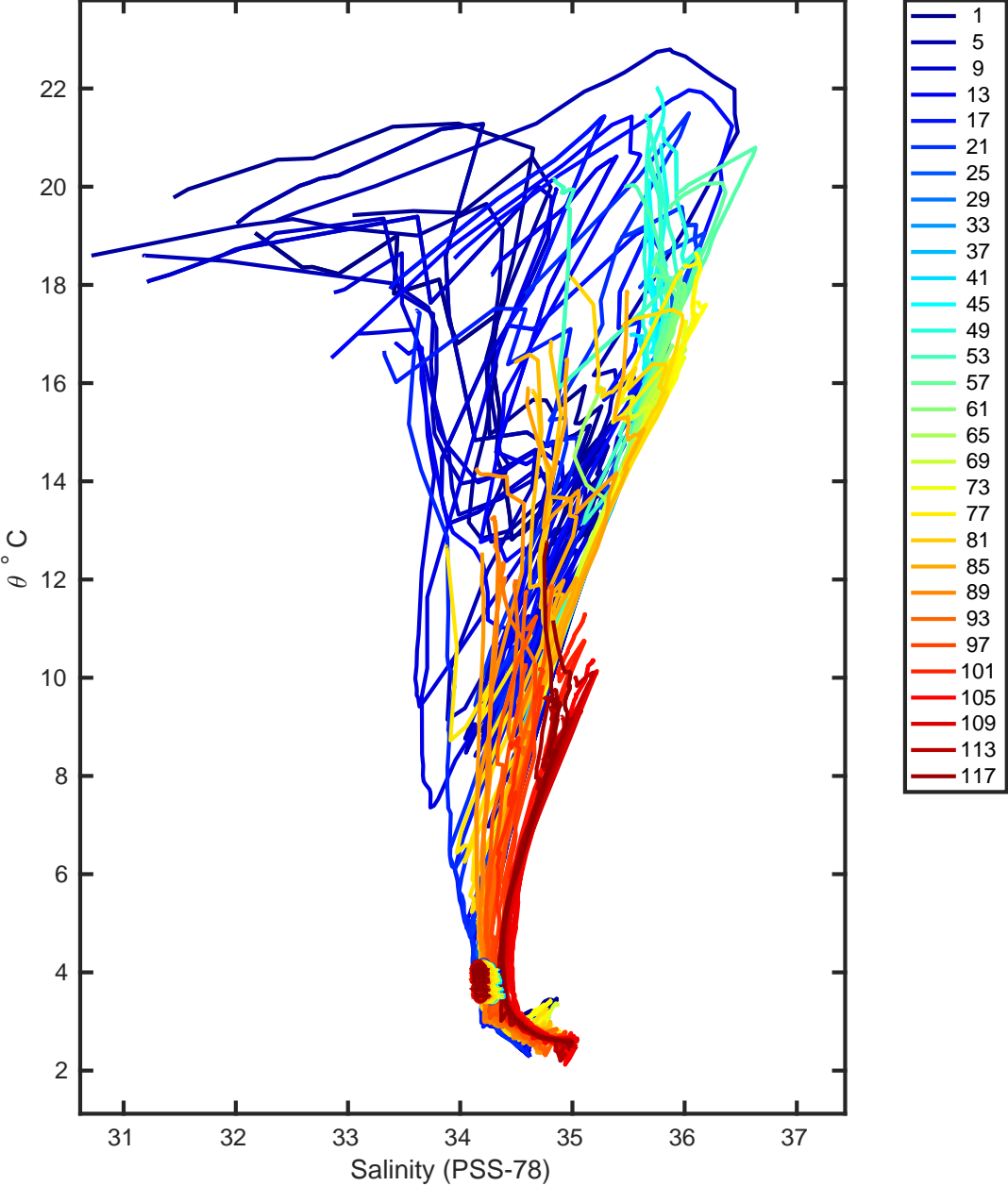
Figure 8: Float 3901893. Uncalibrated float data and mapped salinity.
