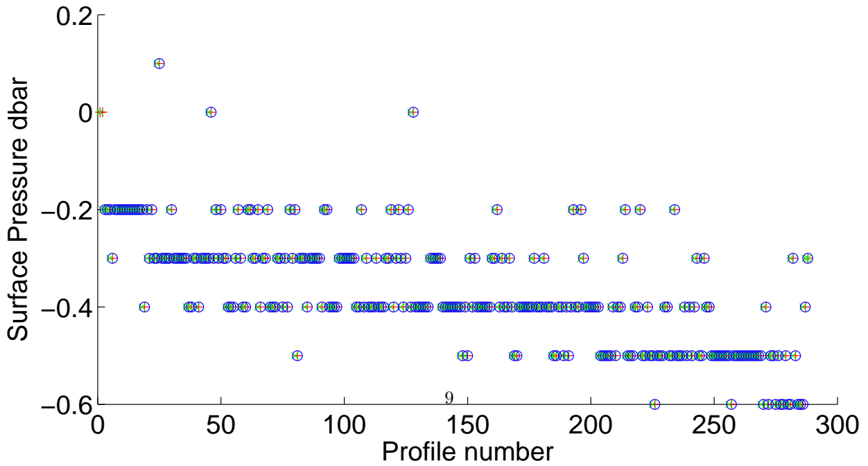
Figure 7: Float 6901121. Sea surface pressure data. The red cross indicate the raw pressure before float descent, recorded after sending data to GDAC. Blue circle indicate pressure value in the real-time. Green rotated cross shows the pressure correction applied from the previous float cycle.
