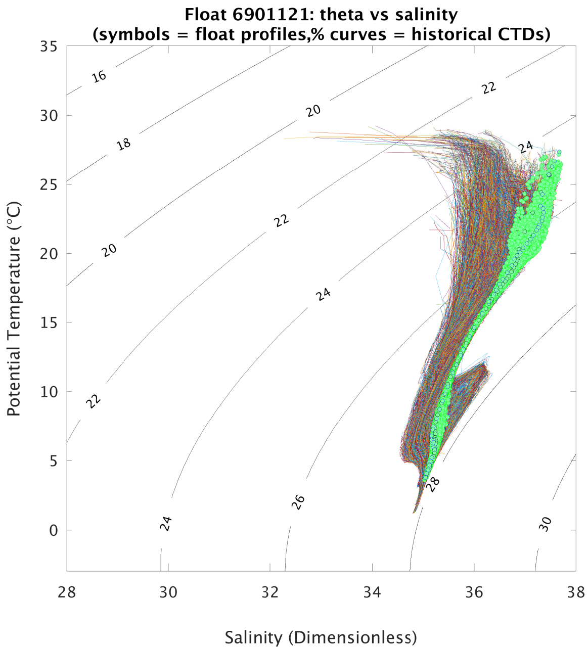
Figure 5: Float 6901121. Theta/S plotted with climatology from the spatial range of 10°. The black and blue cycles indicates the first and the last Argo profile, respectively. Green symbols represent other Argo profiles.
