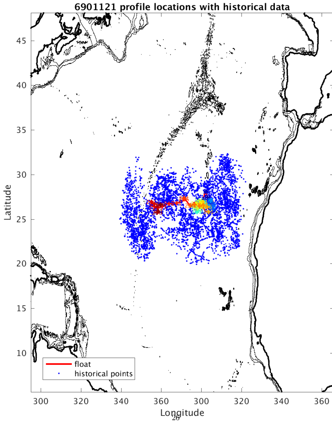
Figure 16: Float 6901121. Trajectory of the float with historical CTD data. The black contours indicate the bathymetry at 0, 200, 1000 and 2000 m.
