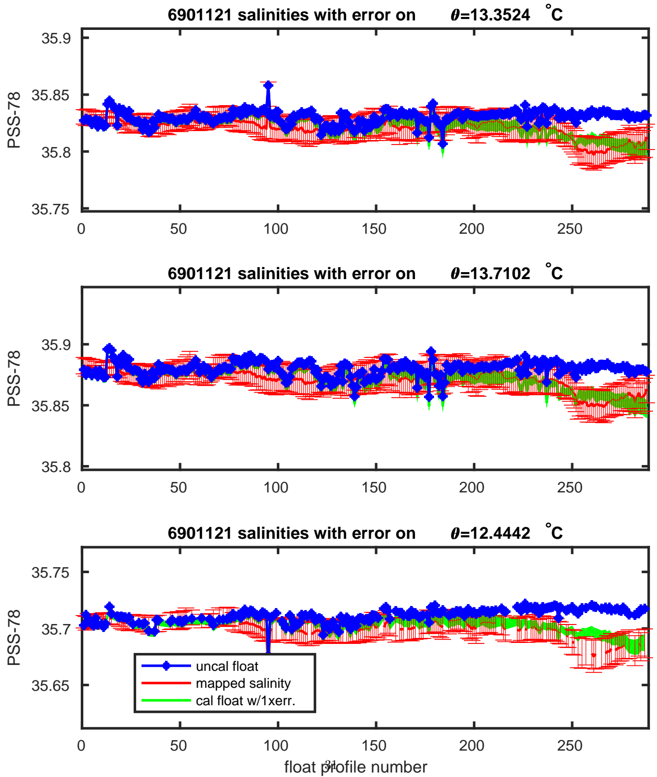
Figure 21: Float 6901121. Salinities with errors on \theta .
