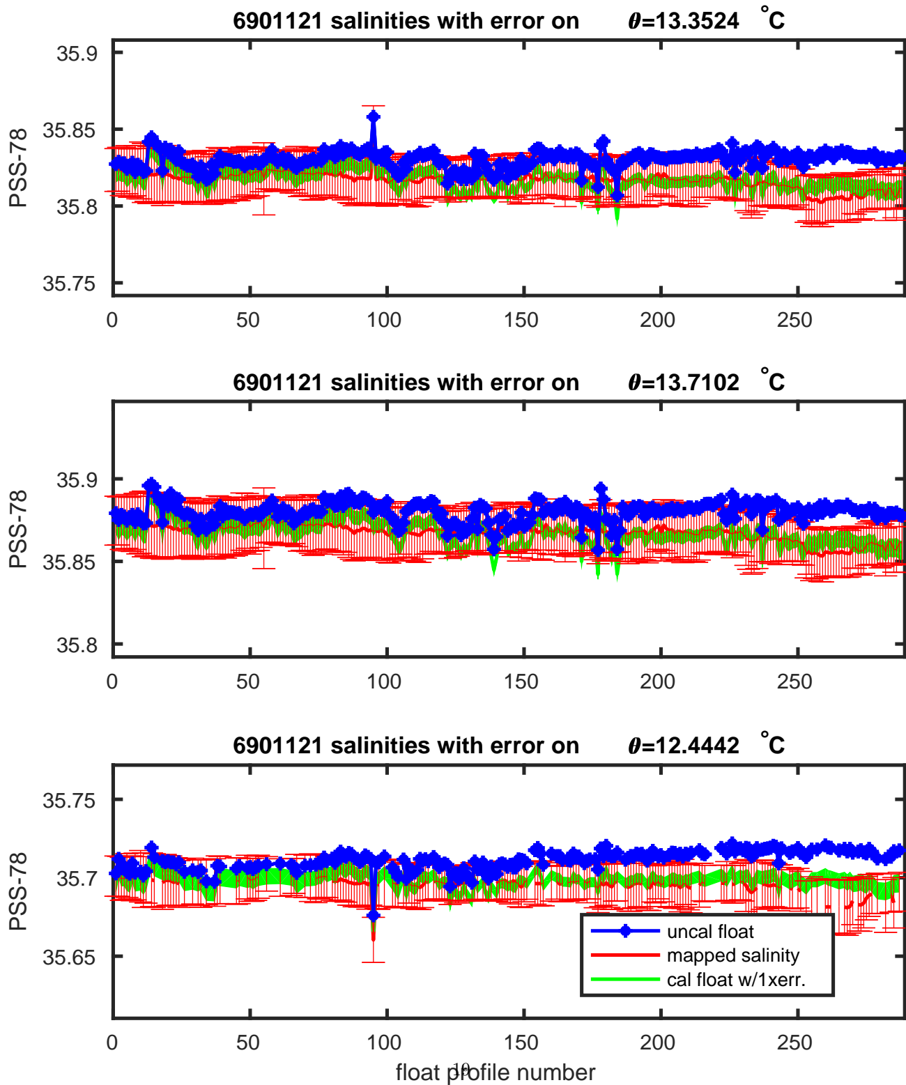
Figure 13: Float 6901121. Salinities with errors on \theta levels.
