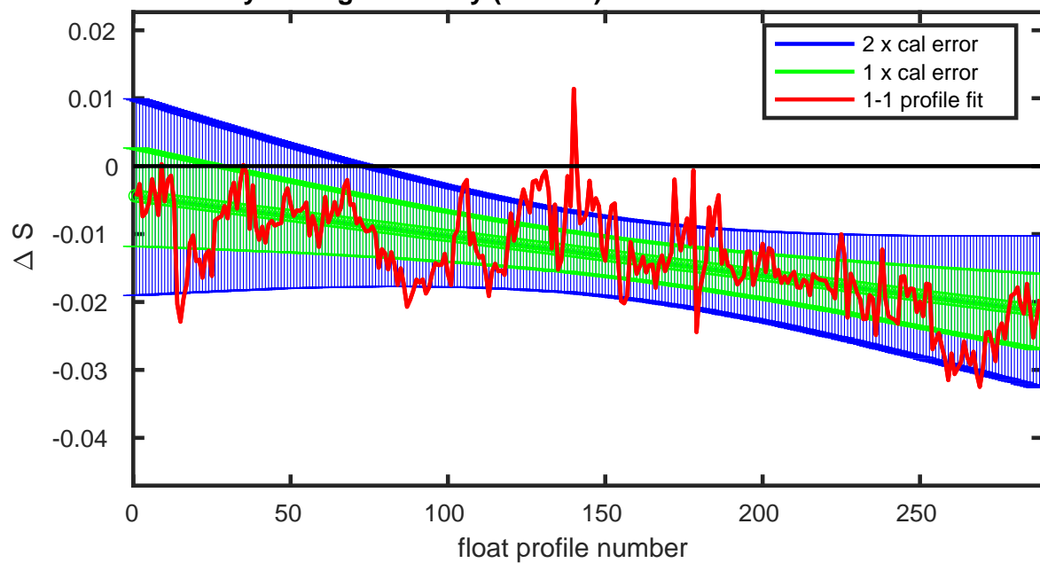
Figure 10: Float 6901121. Potential conductivity (top) and vertically averaged salinity (bottom) with errors.
