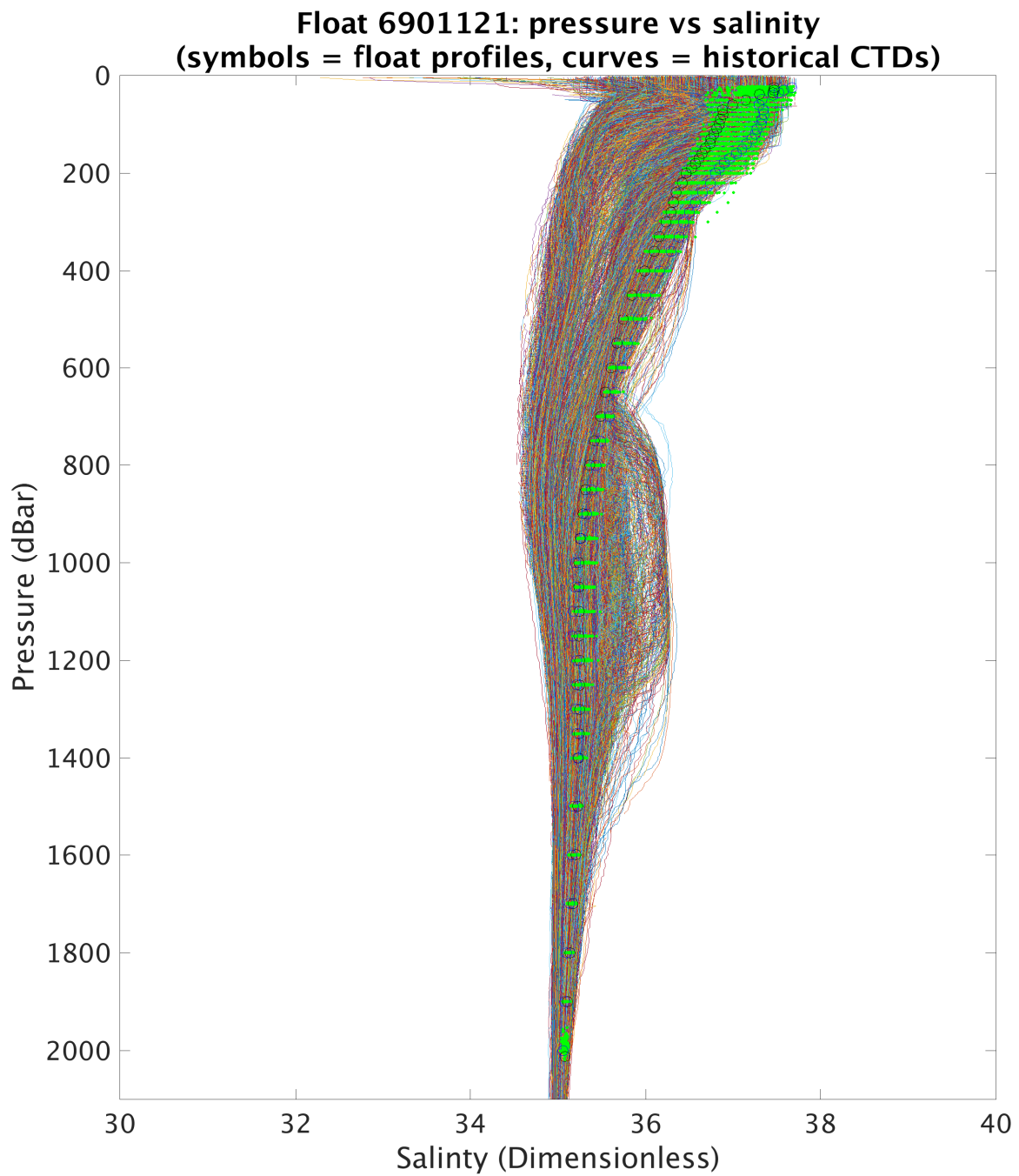
Figure 4: Float 6901121. Float profile of salinity (dimensionless) plotted with climatology from the spatial range of 10^\circ . The black and blue circles indicate the first and the last Argo profile, respectively. Green symbols represent other Argo profiles.
