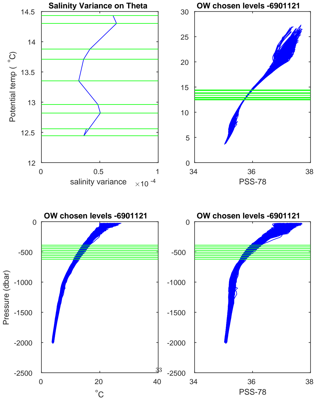
Figure 23: Float 6901121. Salinity, salinity variance on theta and OW chosen levels.
