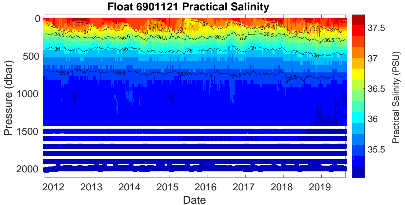
Figure 2: Float 6901121. Time series of the vertical distribution of practical salinity (PSU).
