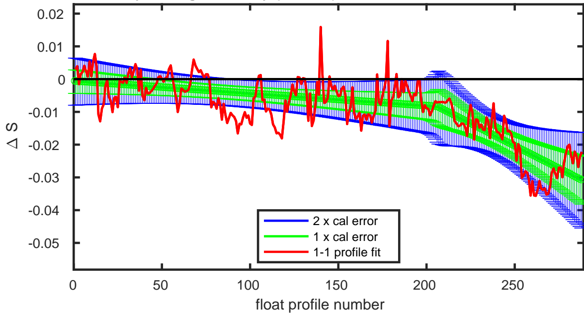
Figure 18: Float 6901121. Potential conductivity (top) and vertically averaged salinity (bottom) with errors.
