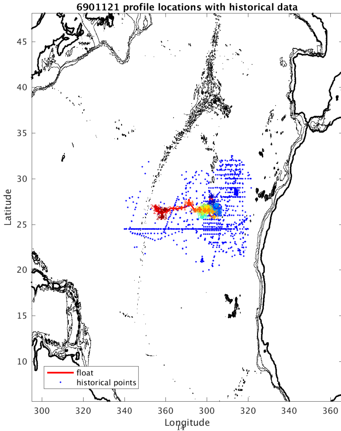
Figure 8: Float 6901121. Trajectory of the float with historical CTD data. The black contours indicate the bathymetry at 0, 200, 1000 and 2000 m.
