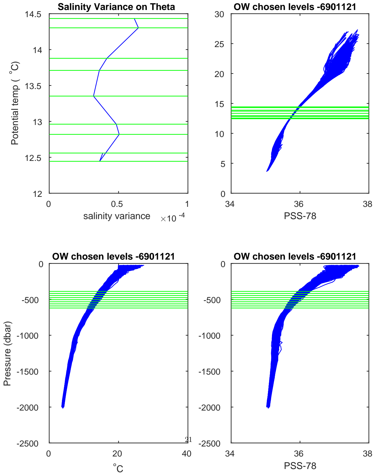
Figure 15: Float 6901121. Salinity, salinity variance on theta and OW chosen levels.
