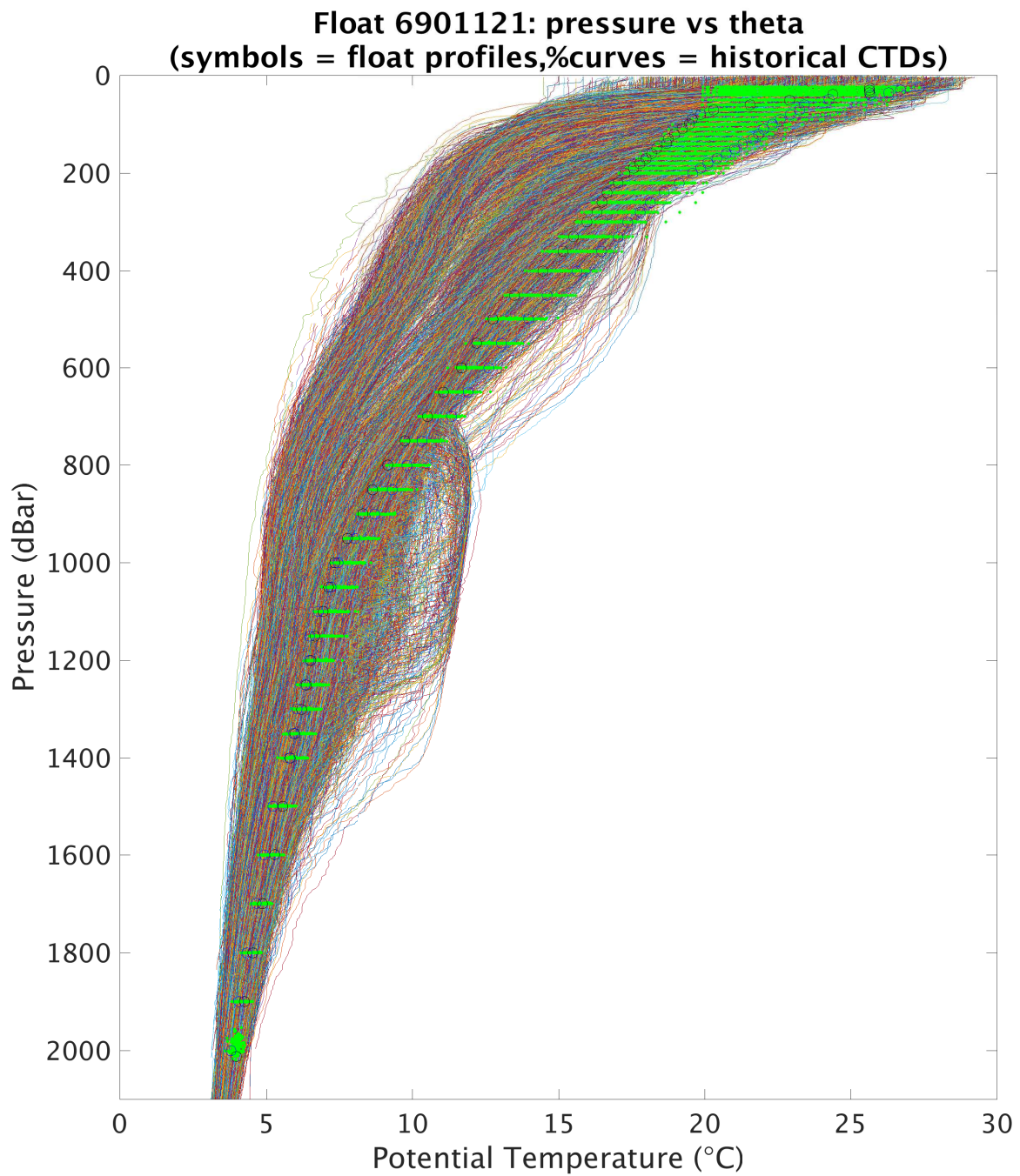
Figure 3: Float 6901121. Float profile of potential temperature (°C) plotted with climatology from the spatial range of 10 °. The black and blue cycles indicates the first and the last Argo profile, respectively. Green symbols represent other Argo profiles.
