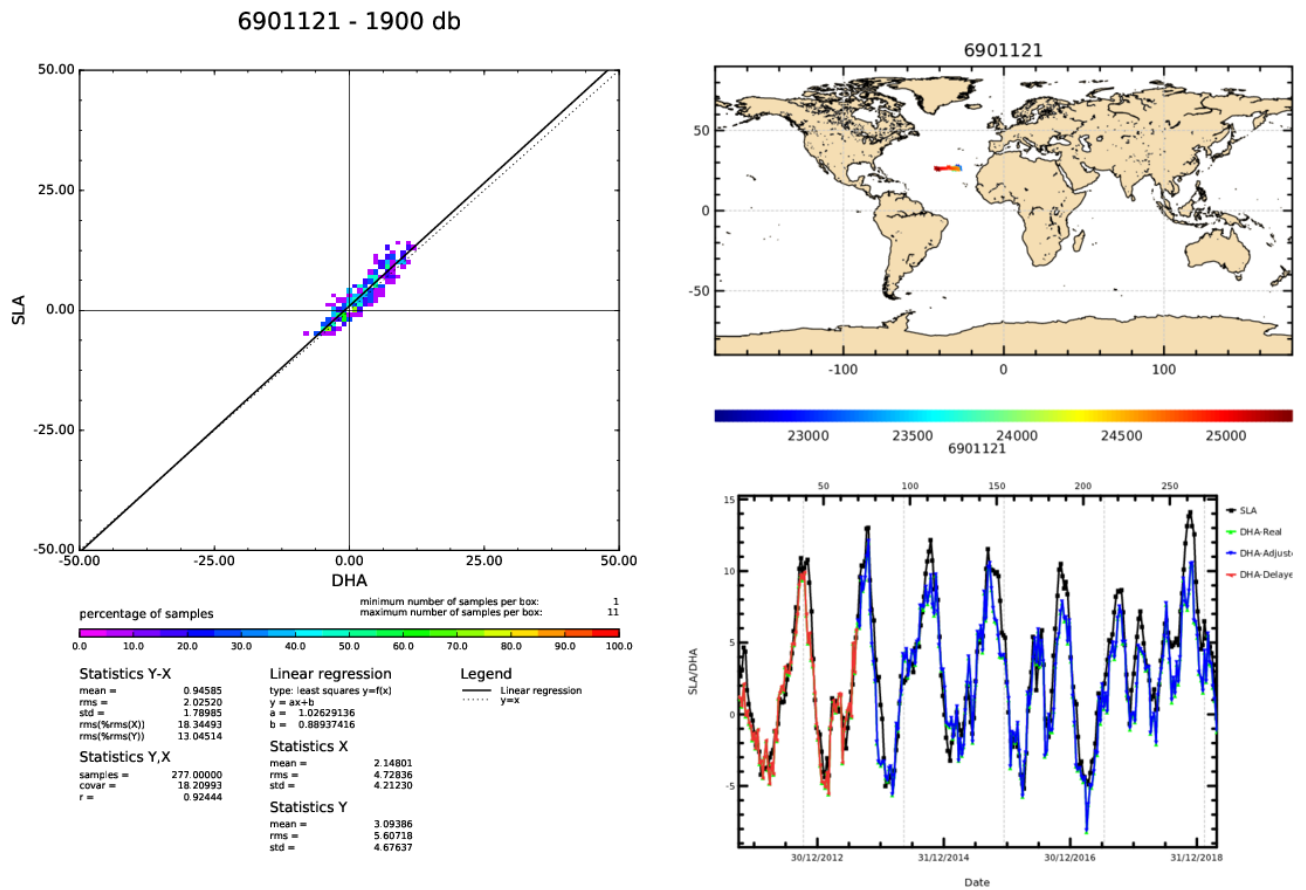
Figure 6: Float 6901121. The comparison between the Sea Surface Height (SSH) from the satellite altimetry and Dynamic Height Anomaly (DHA) extracted from the Argo float temperature and salinity data
