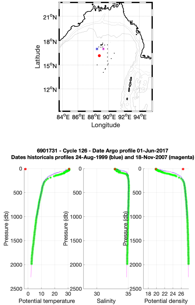
Figure 8: Float 6901731, cycle 126 - (Upper panel) Position of the Argo profile (red) and of the nearest Argo profiles (black). The nearest Argo profile in time is in magenta while the nearest Argo profile in space is in blue. (Lower panels) Temperature, salinity and potential density as function of pressure for the Argo profile (stars) and for the nearest Argo profile in time (magenta line) and for the nearest ARGO profile in space (blue line). The color of the Argo profile represents the QC flag (green for a QC=1 ; blue for a QC=2; orange for a QC=3 and red for a QC=4).
