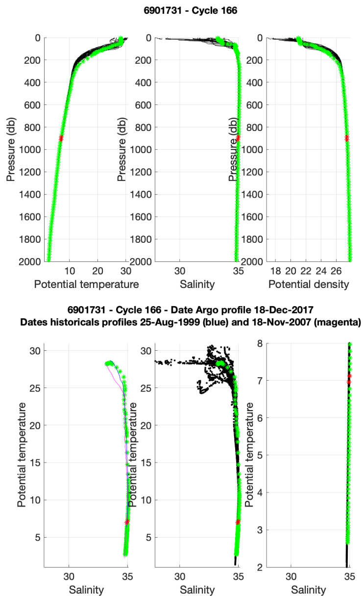
Figure 13: Float 6901731, cycle 166 : The Argo profile (stars) is compared to the nearest ARGO profiles (black line) and to two specific profiles : the nearest profile in time (magenta) and the nearest profile in space (blue). The color of the Argo profile represents the QC flag (green for a QC=1 ; blue for a QC=2; orange for a QC=3 and red for a QC=4). (Upper panels) Temperature (left panel), salinity (middle panel) and potential density (right panel) as function of pressure. (Lower panels) \theta/S diagrams.
