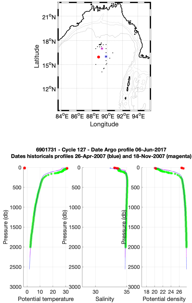
Figure 10: Float 6901731, cycle 127 - (Upper panel) Position of the Argo profile (red) and of the nearest Argo profiles (black). The nearest Argo profile in time is in magenta while the nearest Argo profile in space is in blue. (Lower panels) Temperature, salinity and potential density as function of pressure for the Argo profile (stars) and for the nearest Argo profile in time (magenta line) and for the nearest ARGO profile in space (blue line). The color of the Argo profile represents the QC flag (green for a QC=1 ; blue for a QC=2; orange for a QC=3 and red for a QC=4).
