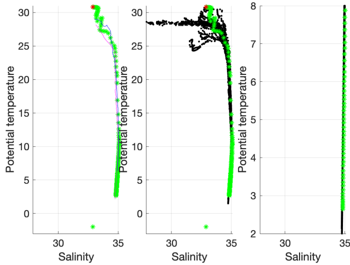
Figure 9: Float 6901731, cycle 126 : The Argo profile (stars) is compared to the nearest ARGO profiles (black line) and to two specific profiles : the nearest profile in time (magenta) and the nearest profile in space (blue). The color of the Argo profile represents the QC flag (green for a QC=1 ; blue for a QC=2; orange for a QC=3 and red for a QC=4). (Upper panels) Temperature (left panel), salinity (middle panel) and potential density (right panel) as function of pressure. (Lower panels) \theta/S diagrams.
