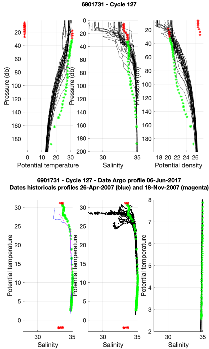
Figure 11: Float 6901731, cycle 127 : The Argo profile (stars) is compared to the nearest ARGO profiles (black line) and to two specific profiles : the nearest profile in time (magenta) and the nearest profile in space (blue). The color of the Argo profile represents the QC flag (green for a QC=1 ; blue for a QC=2; orange for a QC=3 and red for a QC=4). (Upper panels) Temperature (left panel), salinity (middle panel) and potential density (right panel) as function of pressure. (Lower panels) \theta/S diagrams.
