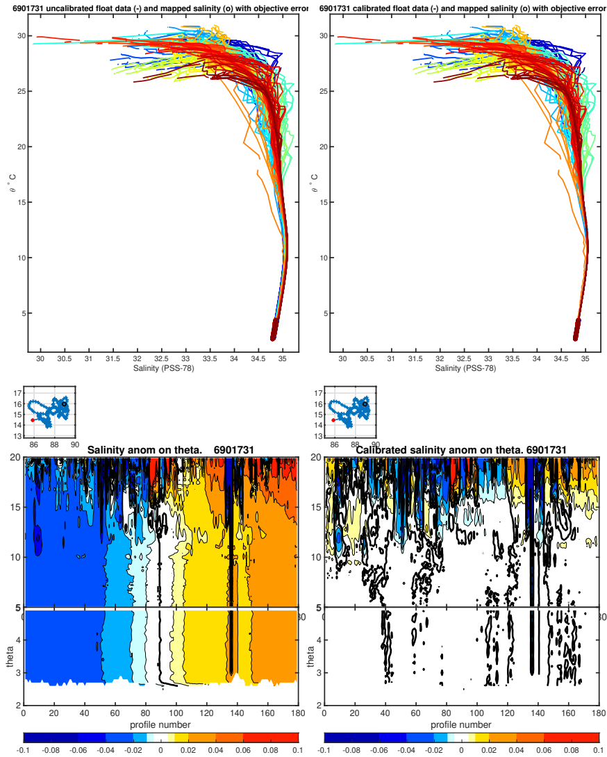
Figure 16: ( top panel ) : Comparison of the \theta/S diagram of the float with the historial database. (left) raw data. (right) corrected data using the OW correction. (bottom panel) : Salinity anomaly. (left) raw data. (right) corrected data using the OW correction.
