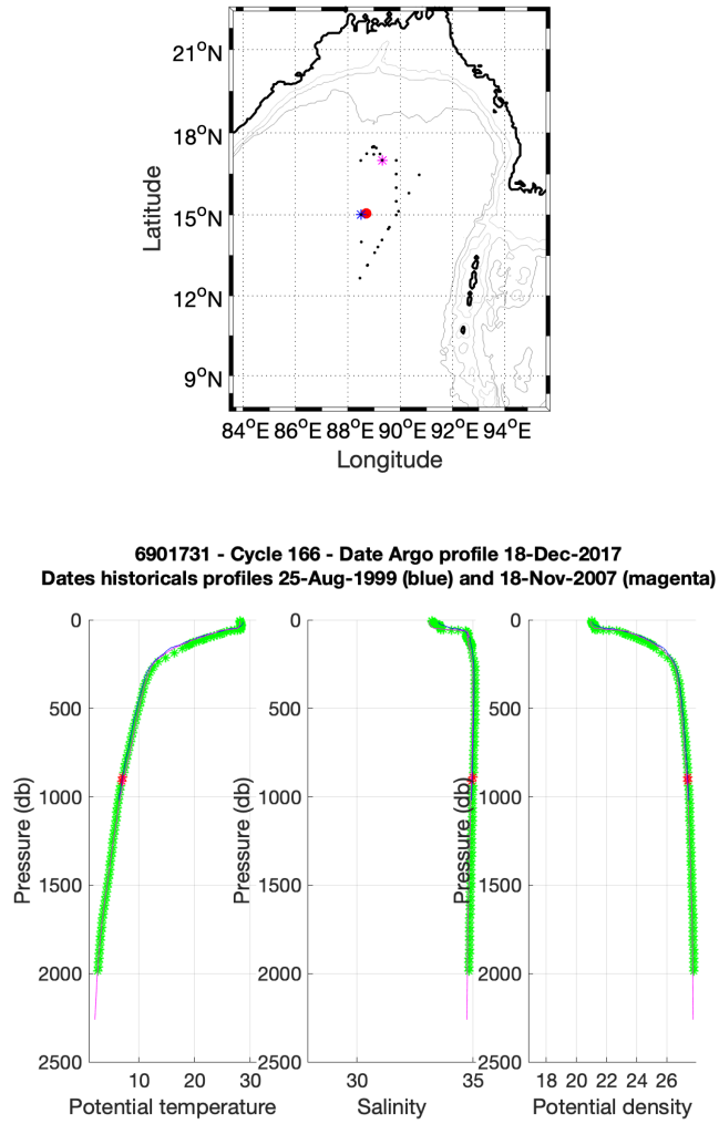
Figure 12: Float 6901731, cycle 166 - (Upper panel) Position of the Argo profile (red) and of the nearest Argo profiles (black). The nearest Argo profile in time is in magenta while the nearest Argo profile in space is in blue. (Lower panels) Temperature, salinity and potential density as function of pressure for the Argo profile (stars) and for the nearest Argo profile in time (magenta line) and for the nearest ARGO profile in space (blue line). The color of the Argo profile represents the QC flag (green for a QC=1 ; blue for a QC=2; orange for a QC=3 and red for a QC=4).
