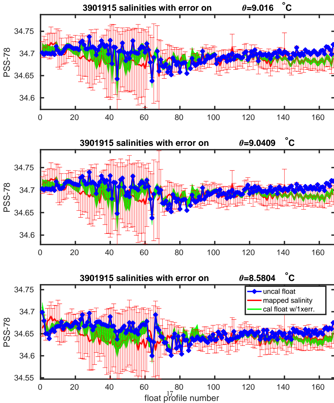
Figure 12: Float 3901915. Salinities with errors on \theta levels.
