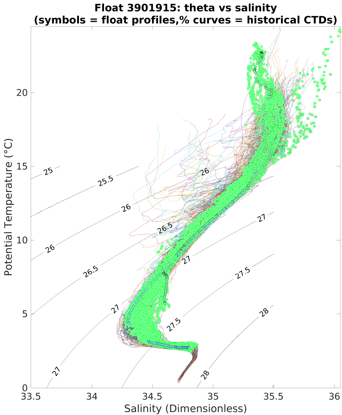
Figure 5: Float 3901915. Theta/S plotted with climatology from the spatial range of 10^{\circ} . The black and blue cycles indicates the first and the last Argo profile, respectively. Green symbols represent other Argo profiles.
