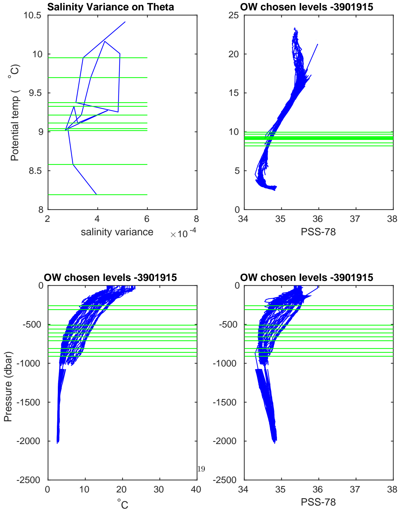
Figure 14: Float 3901915. Salinity, salinity variance on theta and OW chosen levels.
