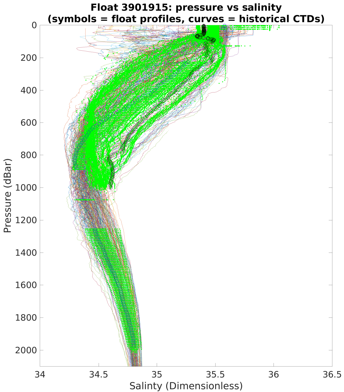
Figure 4: Float 3901915. Float profile of salinity (dimensionless) plotted with climatology from the spatial range of 10°. The black and blue cycles indicates the first and the last Argo profile, respectively. Green symbols represent other Argo profiles.
