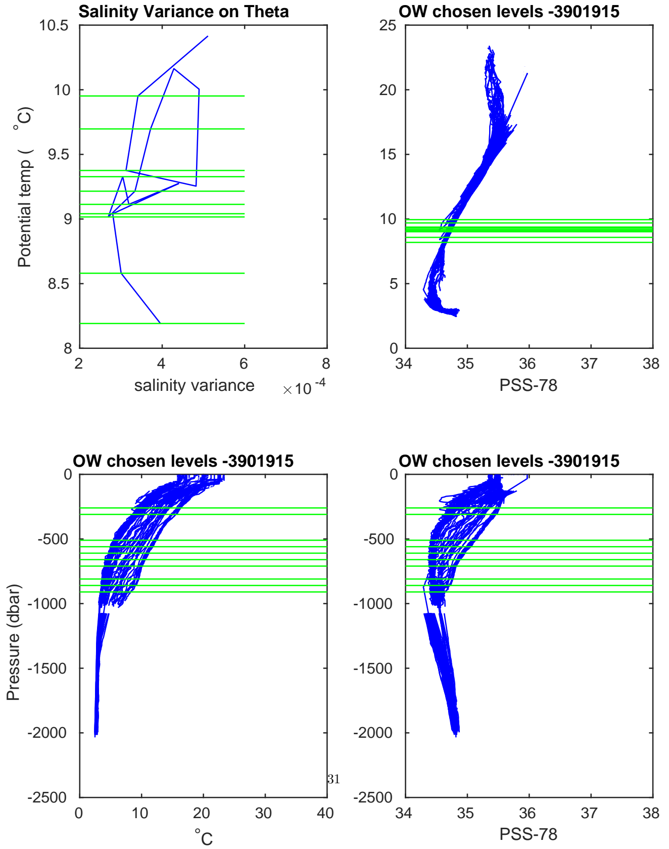
Figure 22: Float 3901915. Salinity, salinity variance on theta and OW chosen levels.
