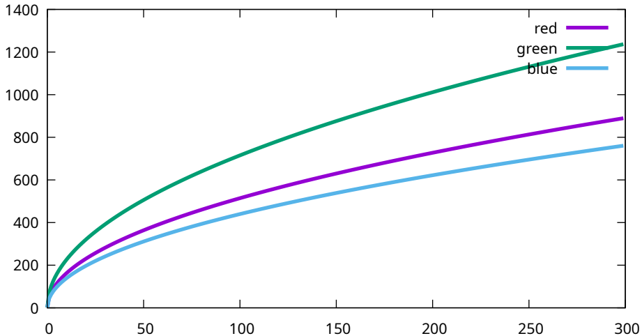
Conversion curves - Canon, EOS R5m2, 200 ISO (9T0A0165)
