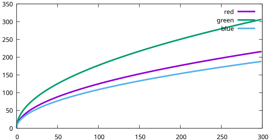
Conversion curves - Canon, EOS R5m2, 4000 ISO (9T0A0180)
