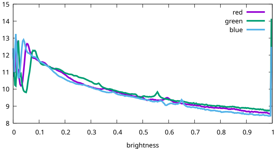
Flat histogram - Canon, EOS R5m2, 1000 ISO (9T0A0174)
