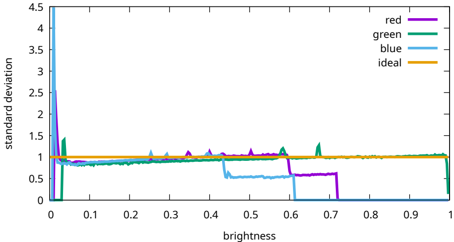
Flat noise levels - Canon, EOS R5m2, 125 ISO (9T0A0163)
