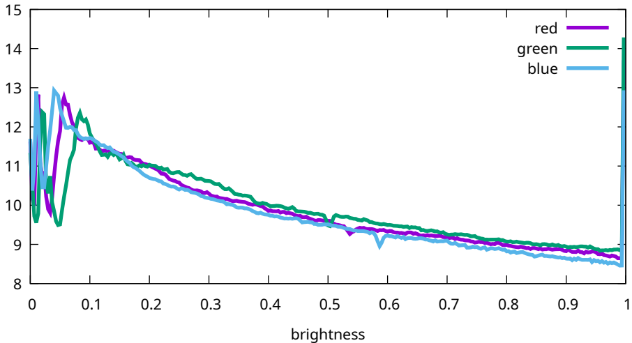
Flat histogram - Canon, EOS R5m2, 125 ISO (9T0A0163)
