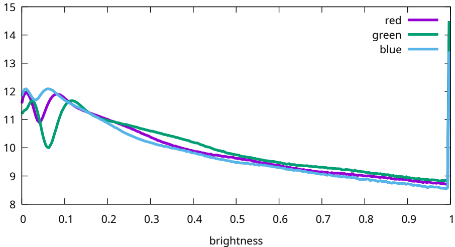
Flat histogram - Canon, EOS R5m2, 32000 ISO (9T0A0189)
