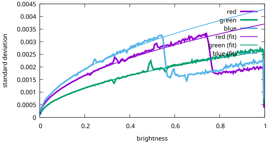
Noise levels - Canon, EOS R5m2, 640 ISO (9T0A0172)
