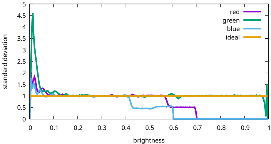
Flat noise levels - Canon, EOS R5m2, 3200 ISO (9T0A0179)
