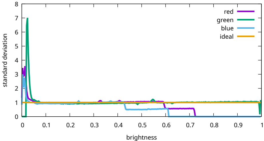
Flat noise levels - Canon, EOS R5m2, 400 ISO (9T0A0170)
