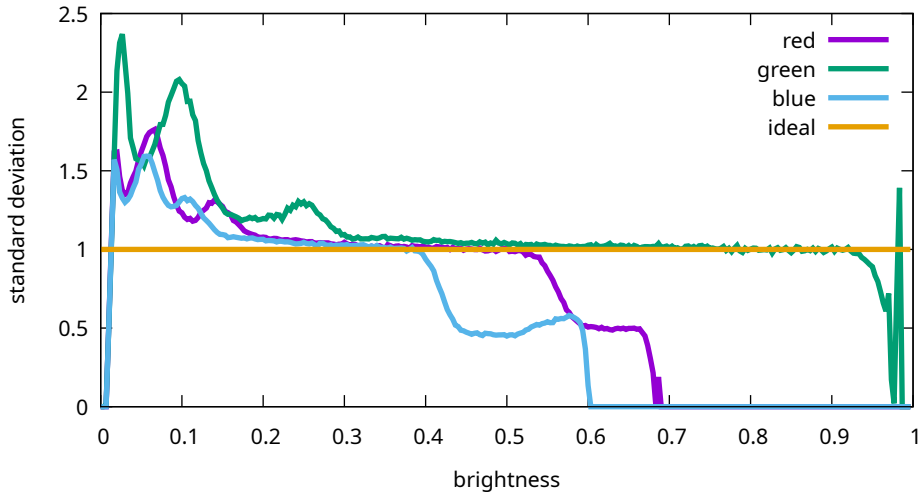
Flat noise levels - Canon, EOS R5m2, 25600 ISO (9T0A0188)
