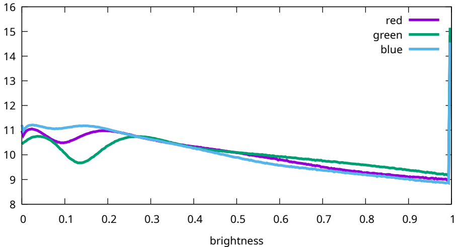
Flat histogram - Canon, EOS R5m2, 102400 ISO (9T0A0192)
