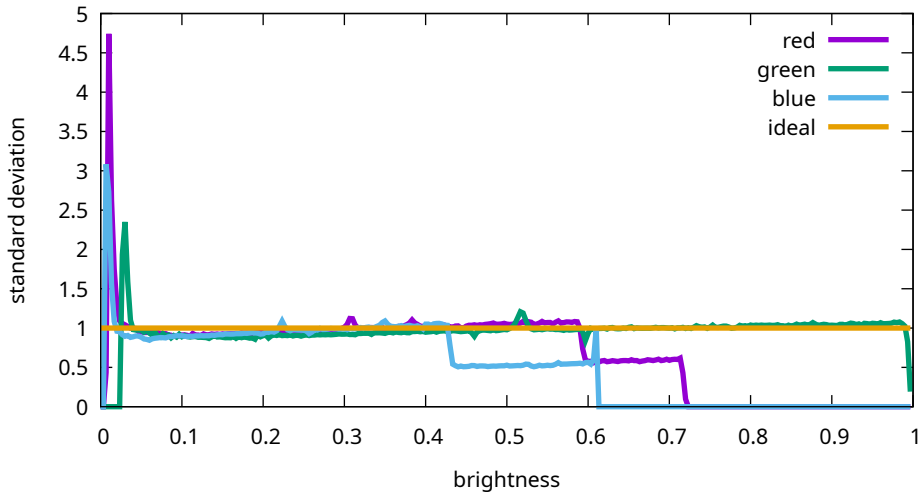
Flat noise levels - Canon, EOS R5m2, 200 ISO (9T0A0167)
