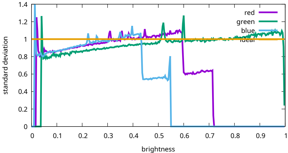
Flat noise levels - Canon, EOS R5m2, 50 ISO (9T0A0129)
