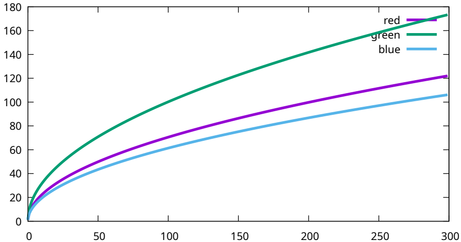
Conversion curves - Canon, EOS R5m2, 12800 ISO (9T0A0185)
