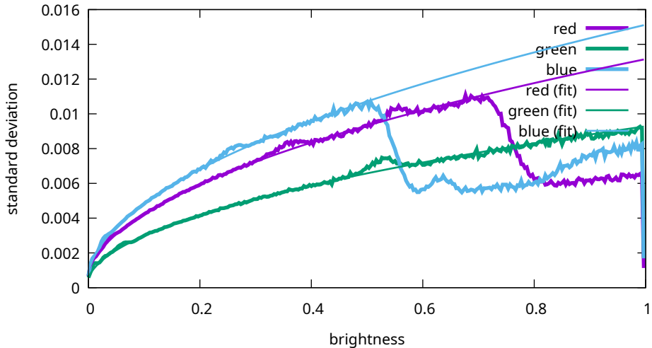
Noise levels - Canon, EOS R5m2, 8000 ISO (9T0A0183)
