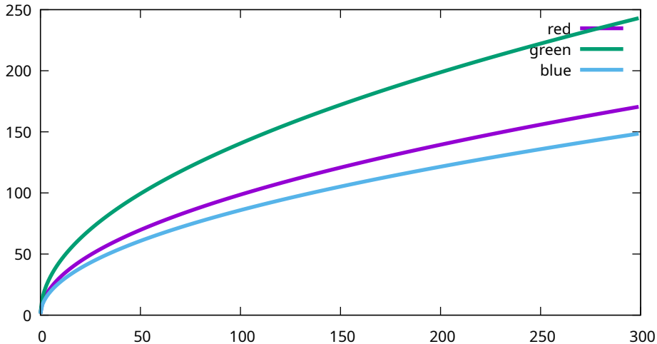
Conversion curves - Canon, EOS R5m2, 6400 ISO (9T0A0182)
