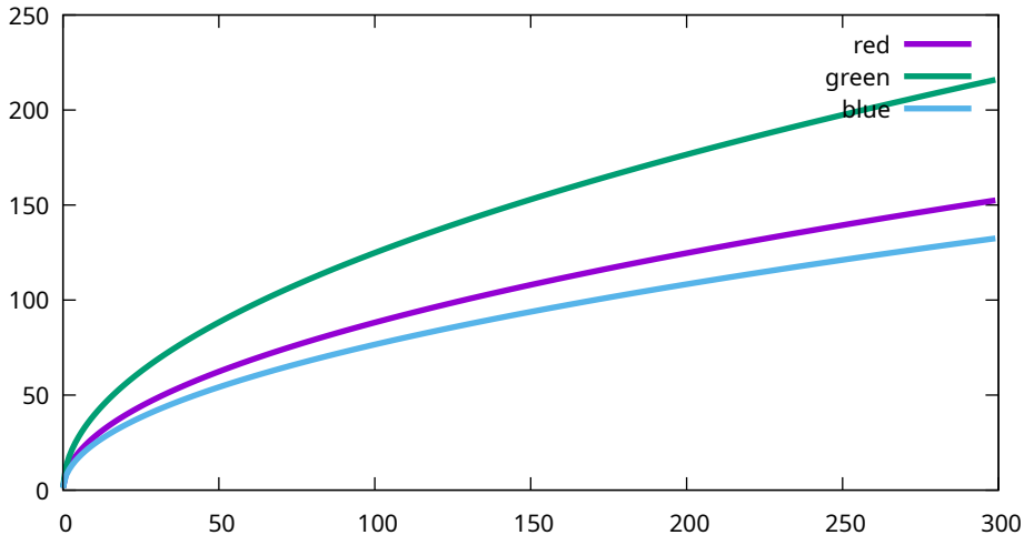
Conversion curves - Canon, EOS R5m2, 8000 ISO (9T0A0183)
