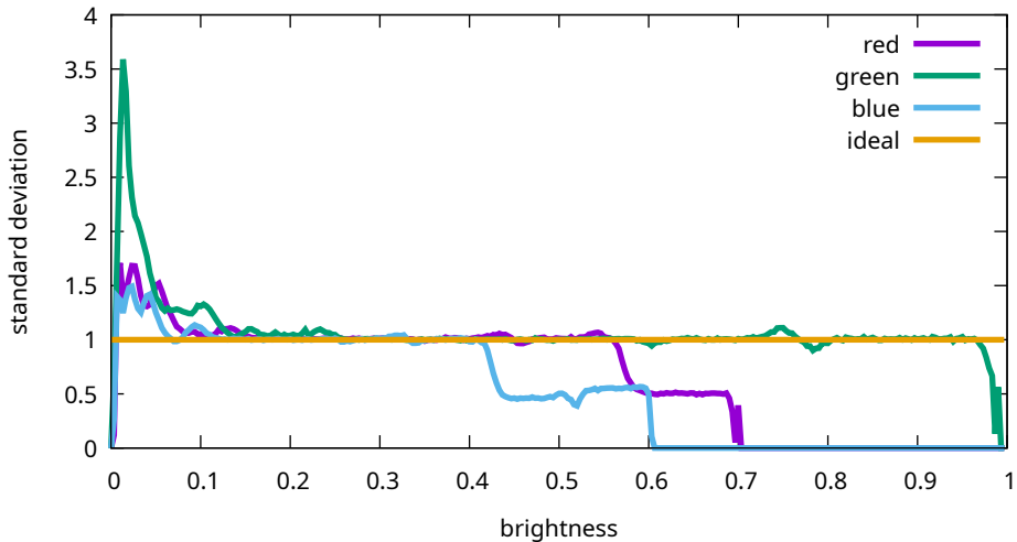
Flat noise levels - Canon, EOS R5m2, 5000 ISO (9T0A0181)
