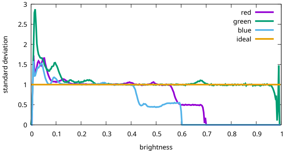
Flat noise levels - Canon, EOS R5m2, 8000 ISO (9T0A0183)
