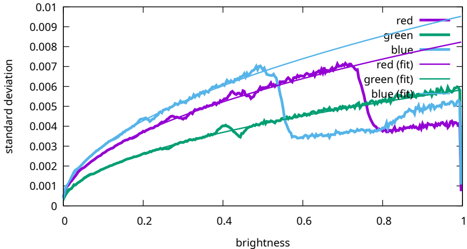
Noise levels - Canon, EOS R5m2, 3200 ISO (9T0A0179)
