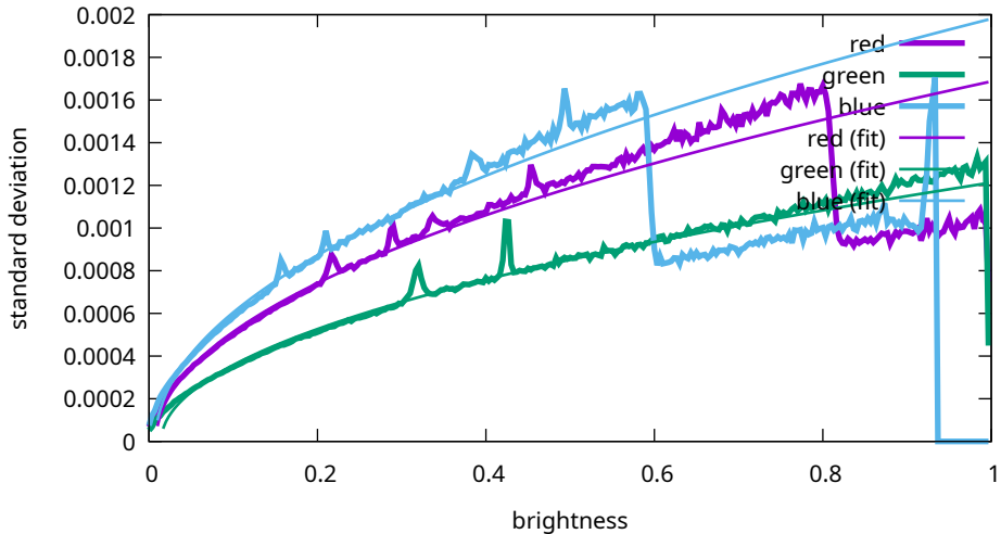
Noise levels - Canon, EOS R5m2, 50 ISO (9T0A0129)
