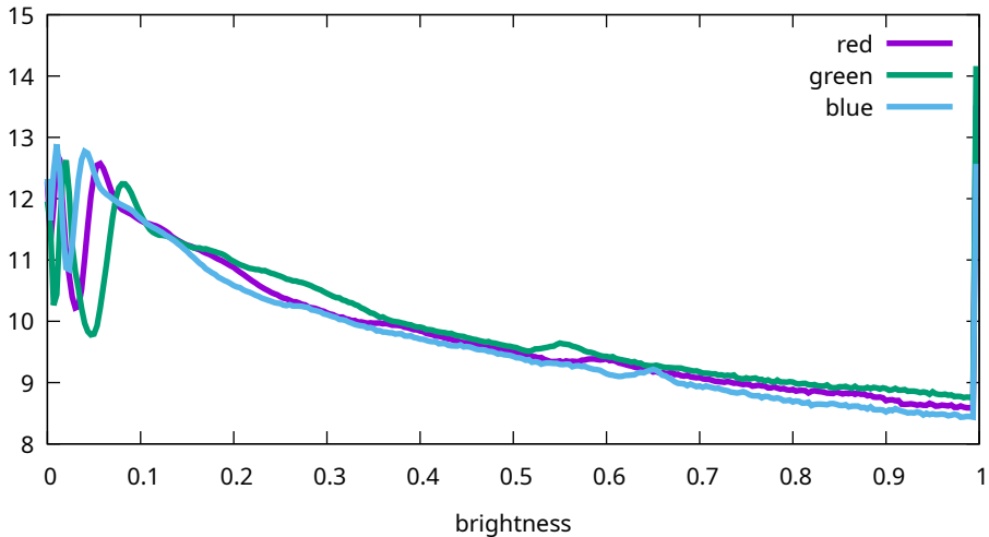
Flat histogram - Canon, EOS R5m2, 4000 ISO (9T0A0180)
