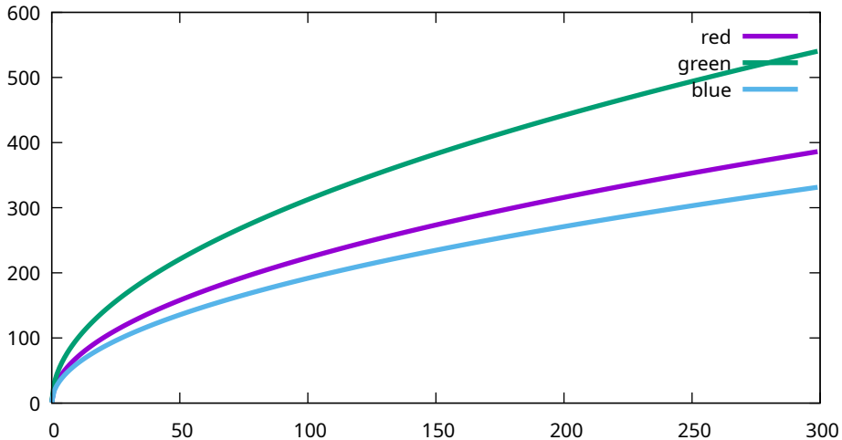
Conversion curves - Canon, EOS R5m2, 1250 ISO (9T0A0175)
