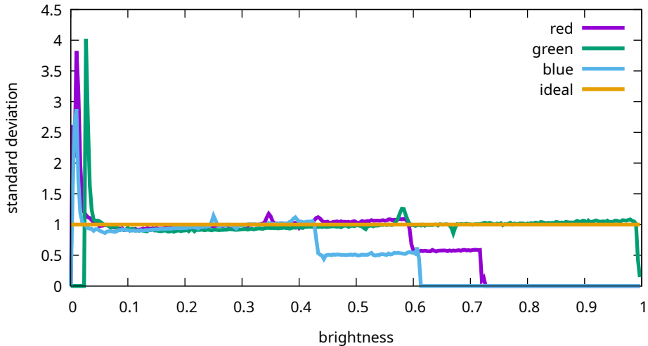
Flat noise levels - Canon, EOS R5m2, 250 ISO (9T0A0168)
