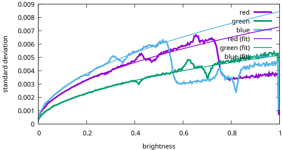
Noise levels - Canon, EOS R5m2, 2500 ISO (9T0A0178)
