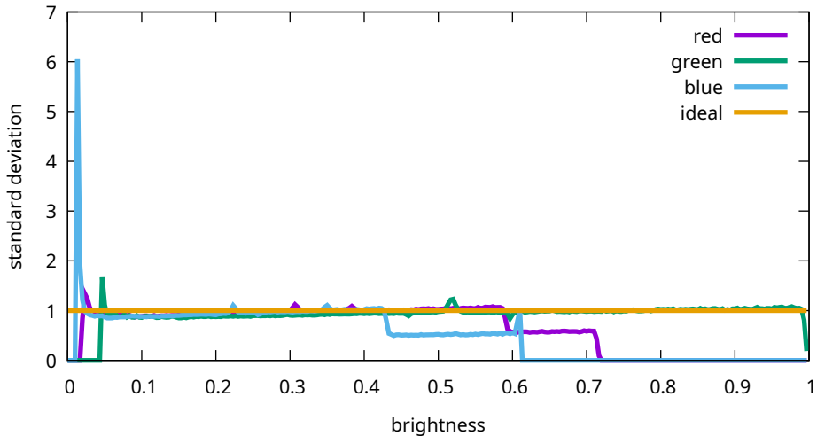
Flat noise levels - Canon, EOS R5m2, 200 ISO (9T0A0165)
