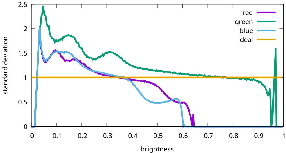
Flat noise levels - Canon, EOS R5m2, 102400 ISO (9T0A0192)
