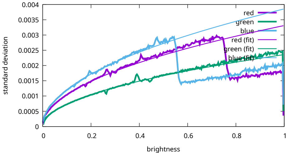
Noise levels - Canon, EOS R5m2, 500 ISO (9T0A0171)
