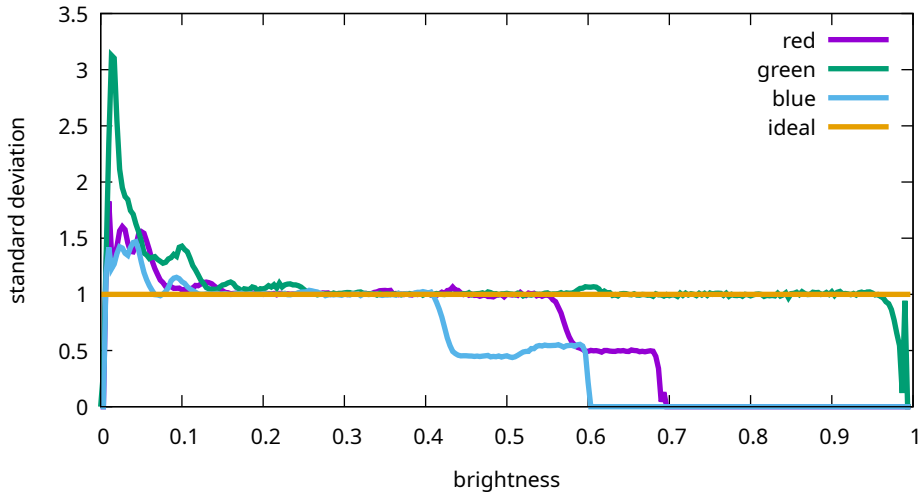
Flat noise levels - Canon, EOS R5m2, 6400 ISO (9T0A0182)
