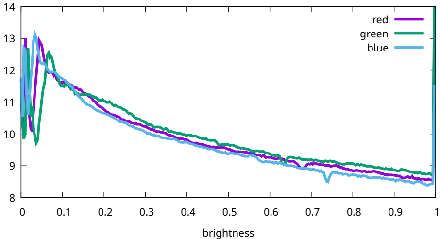
Flat histogram - Canon, EOS R5m2, 160 ISO (9T0A0164)
