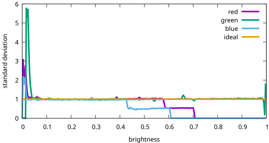
Flat noise levels - Canon, EOS R5m2, 640 ISO (9T0A0172)
