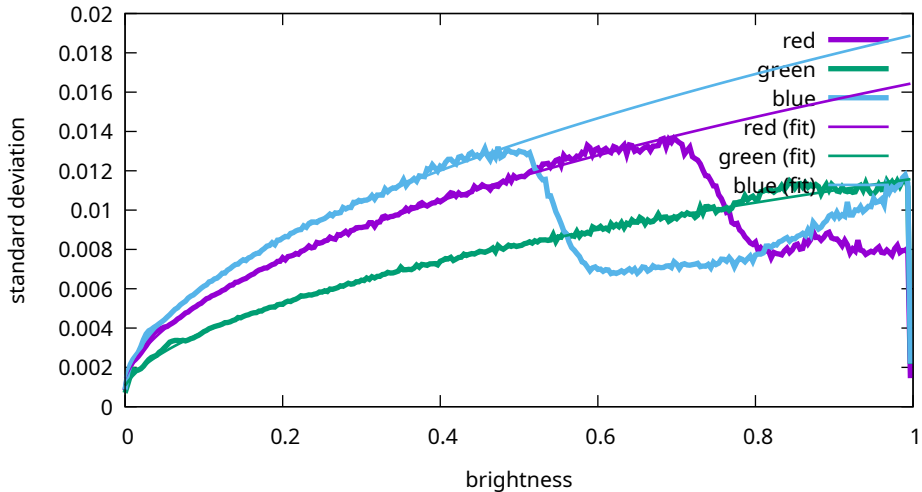
Noise levels - Canon, EOS R5m2, 12800 ISO (9T0A0185)
