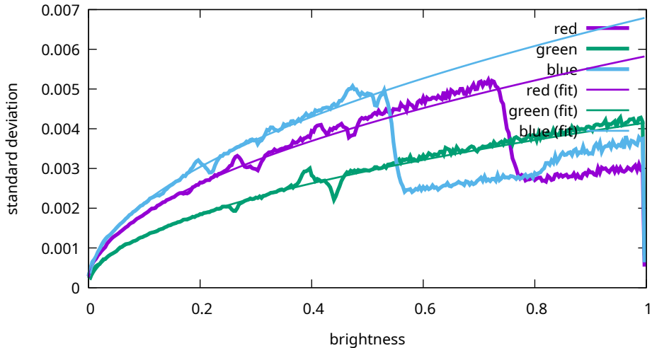
Noise levels - Canon, EOS R5m2, 1600 ISO (9T0A0176)
