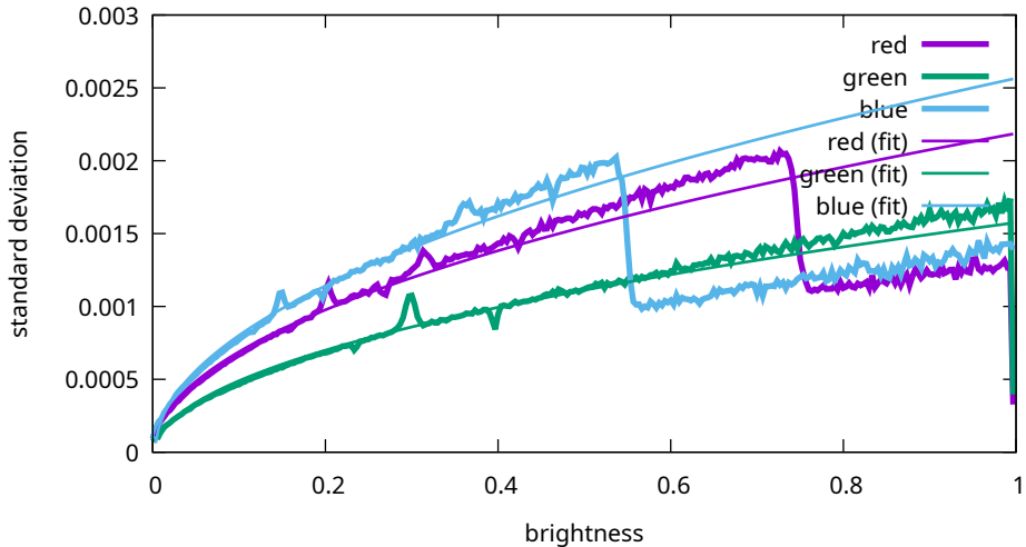
Noise levels - Canon, EOS R5m2, 200 ISO (9T0A0166)
