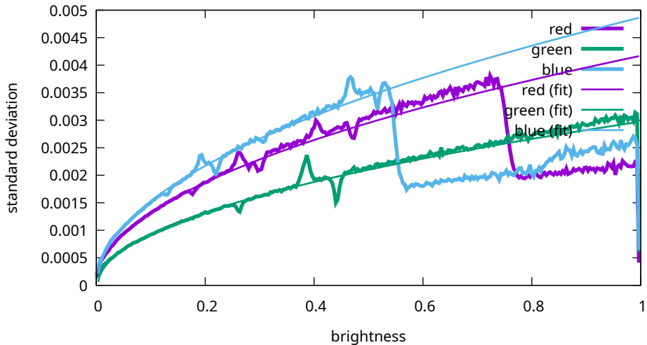
Noise levels - Canon, EOS R5m2, 800 ISO (9T0A0173)
