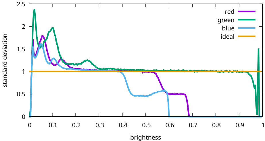
Flat noise levels - Canon, EOS R5m2, 20000 ISO (9T0A0187)
