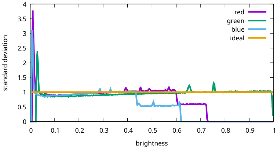
Flat noise levels - Canon, EOS R5m2, 160 ISO (9T0A0164)
