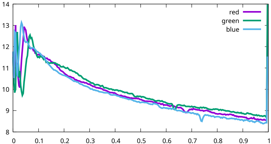
Histogram - Canon, EOS R5m2, 160 ISO (9T0A0164)
