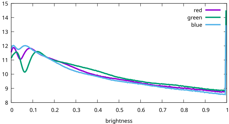
Flat histogram - Canon, EOS R5m2, 40000 ISO (9T0A0190)
