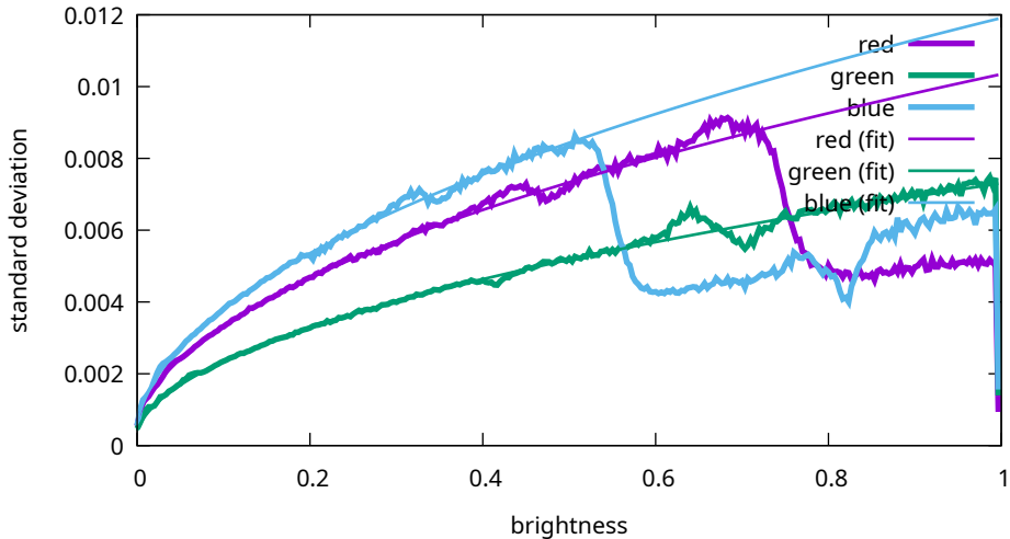
Noise levels - Canon, EOS R5m2, 5000 ISO (9T0A0181)
