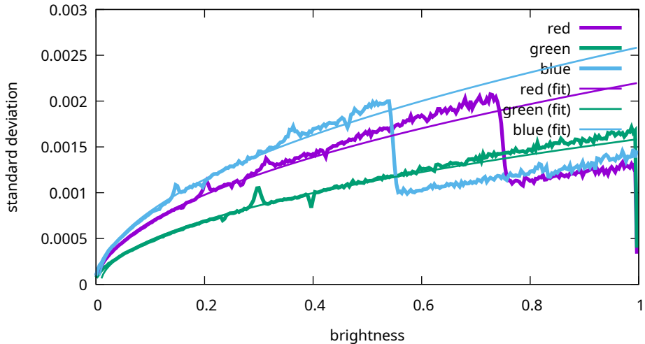
Noise levels - Canon, EOS R5m2, 200 ISO (9T0A0167)
