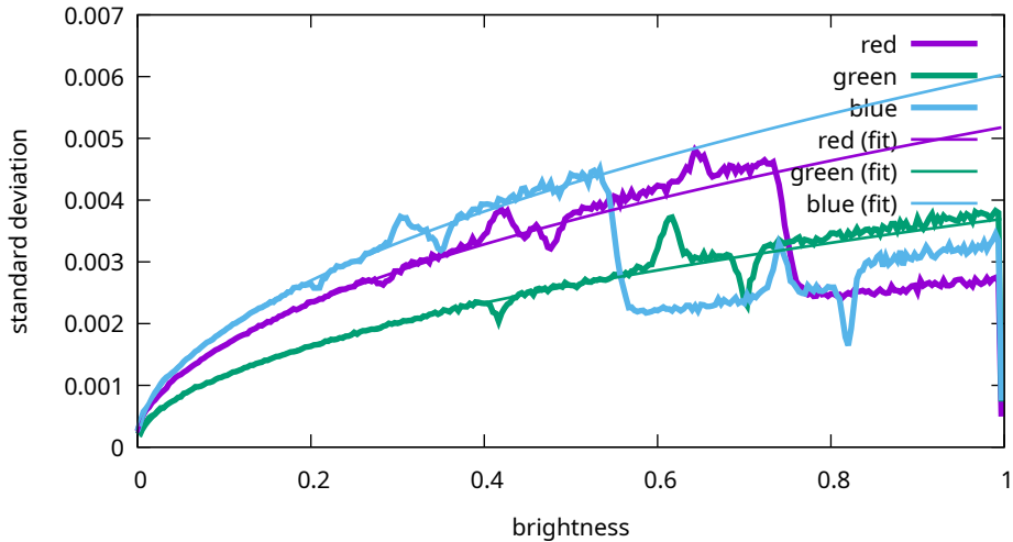
Noise levels - Canon, EOS R5m2, 1250 ISO (9T0A0175)
