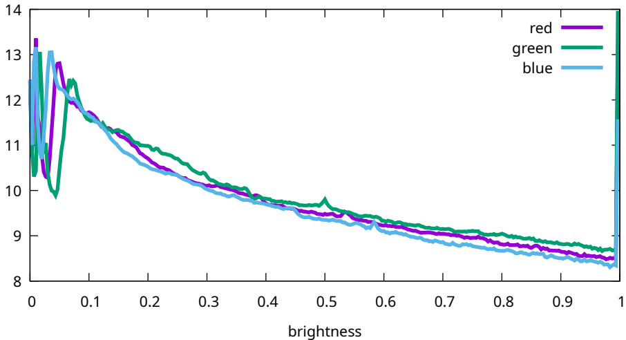
Flat histogram - Canon, EOS R5m2, 250 ISO (9T0A0168)
