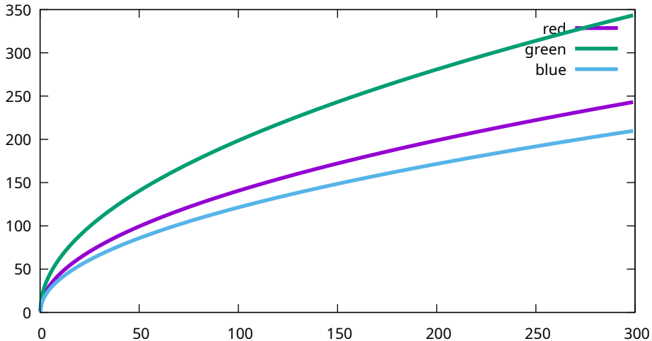
Conversion curves - Canon, EOS R5m2, 3200 ISO (9T0A0179)
