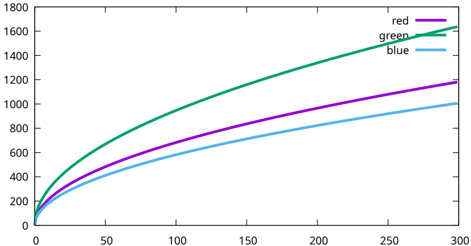
Conversion curves - Canon, EOS R5m2, 50 ISO (9T0A0129)
