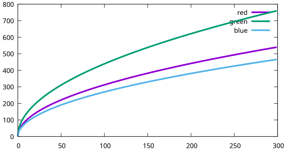
Conversion curves - Canon, EOS R5m2, 640 ISO (9T0A0172)
