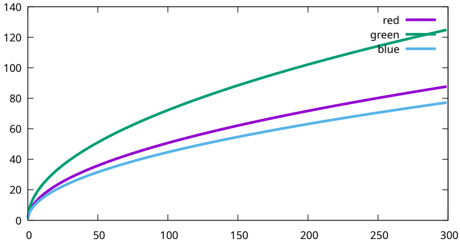
Conversion curves - Canon, EOS R5m2, 25600 ISO (9T0A0188)
