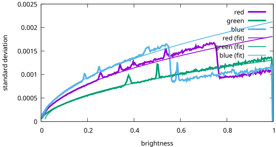
Noise levels - Canon, EOS R5m2, 125 ISO (9T0A0163)
