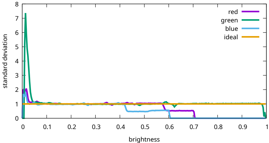
Flat noise levels - Canon, EOS R5m2, 1600 ISO (9T0A0176)
