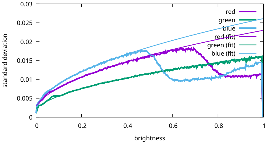
Noise levels - Canon, EOS R5m2, 25600 ISO (9T0A0188)
