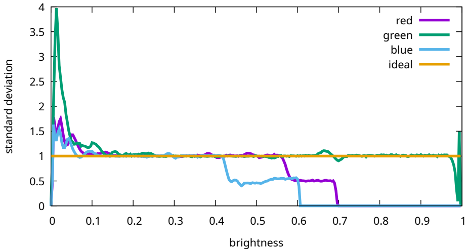
Flat noise levels - Canon, EOS R5m2, 4000 ISO (9T0A0180)
