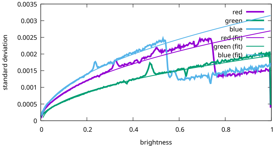
Noise levels - Canon, EOS R5m2, 320 ISO (9T0A0169)
