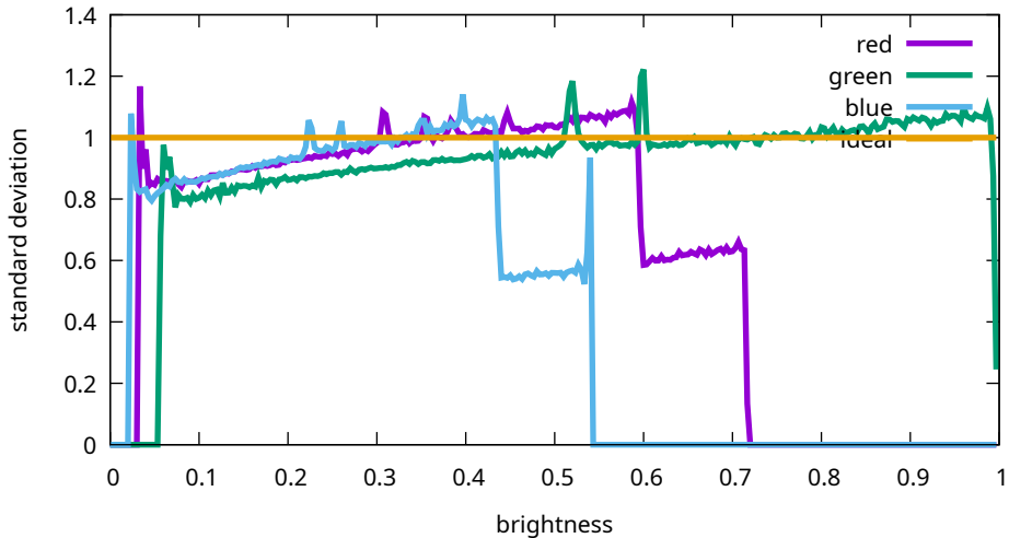
Flat noise levels - Canon, EOS R5m2, 100 ISO (9T0A0159)
