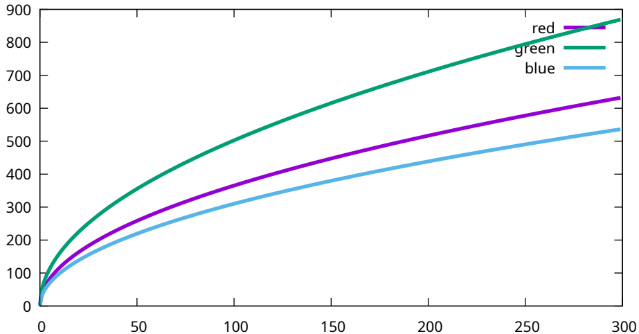
Conversion curves - Canon, EOS R5m2, 400 ISO (9T0A0170)
