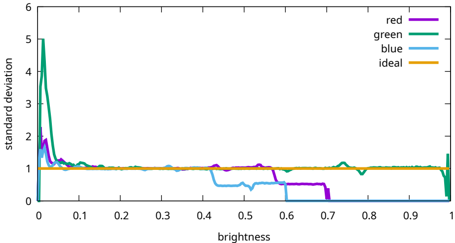
Flat noise levels - Canon, EOS R5m2, 2500 ISO (9T0A0178)
