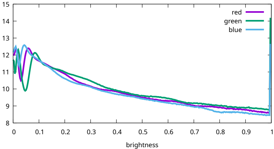
Flat histogram - Canon, EOS R5m2, 10000 ISO (9T0A0184)
