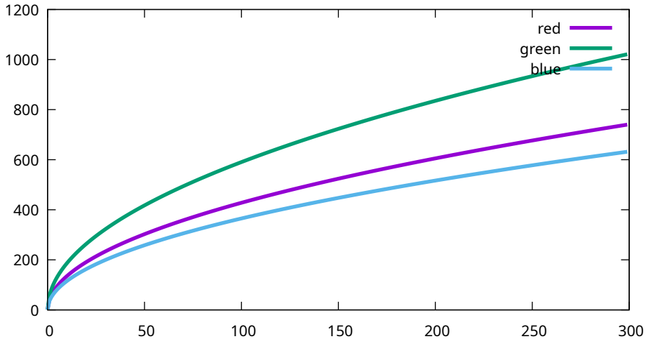
Conversion curves - Canon, EOS R5m2, 320 ISO (9T0A0169)
