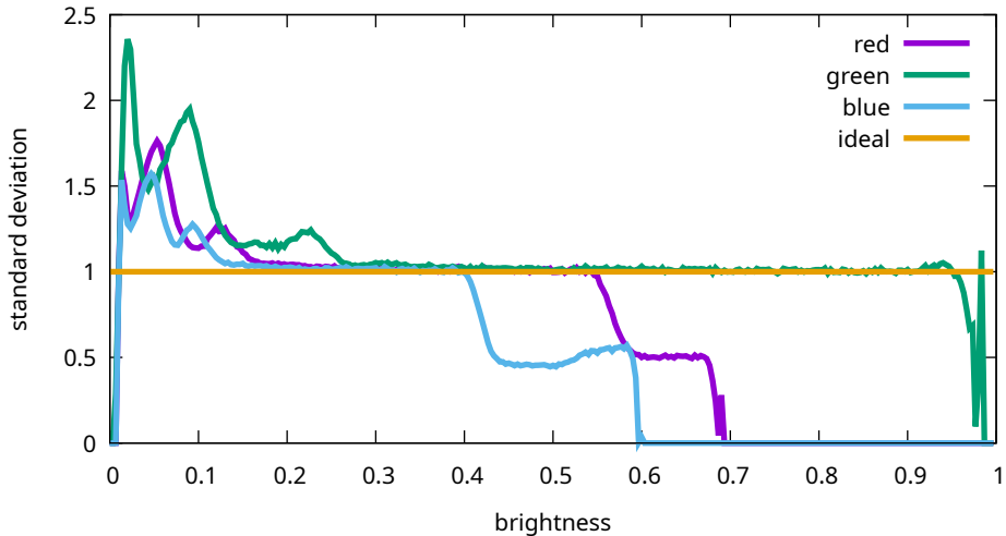
Flat noise levels - Canon, EOS R5m2, 16000 ISO (9T0A0186)
