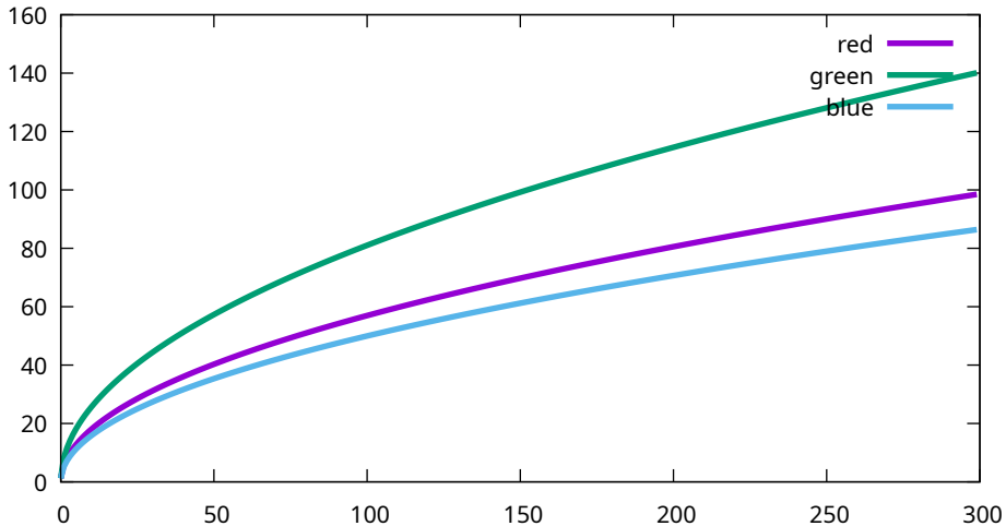
Conversion curves - Canon, EOS R5m2, 20000 ISO (9T0A0187)
