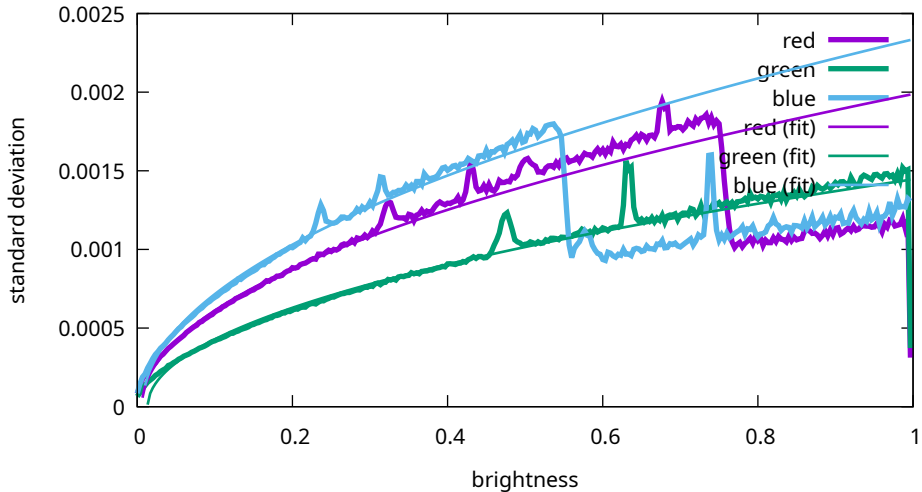
Noise levels - Canon, EOS R5m2, 160 ISO (9T0A0164)
