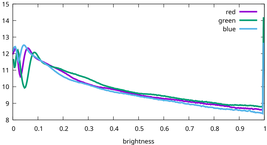
Flat histogram - Canon, EOS R5m2, 12800 ISO (9T0A0185)
