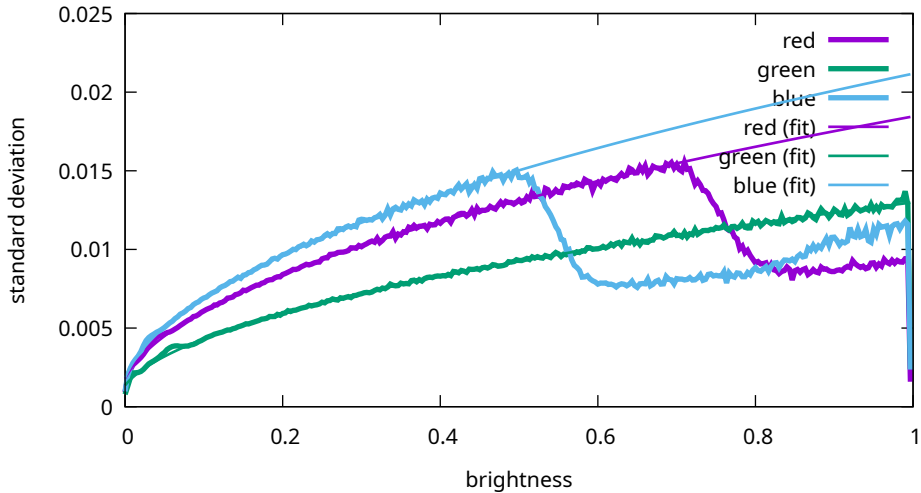
Noise levels - Canon, EOS R5m2, 16000 ISO (9T0A0186)
