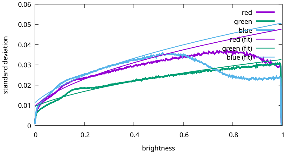
Noise levels - Canon, EOS R5m2, 102400 ISO (9T0A0192)
