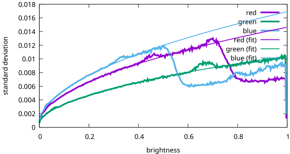
Noise levels - Canon, EOS R5m2, 10000 ISO (9T0A0184)
