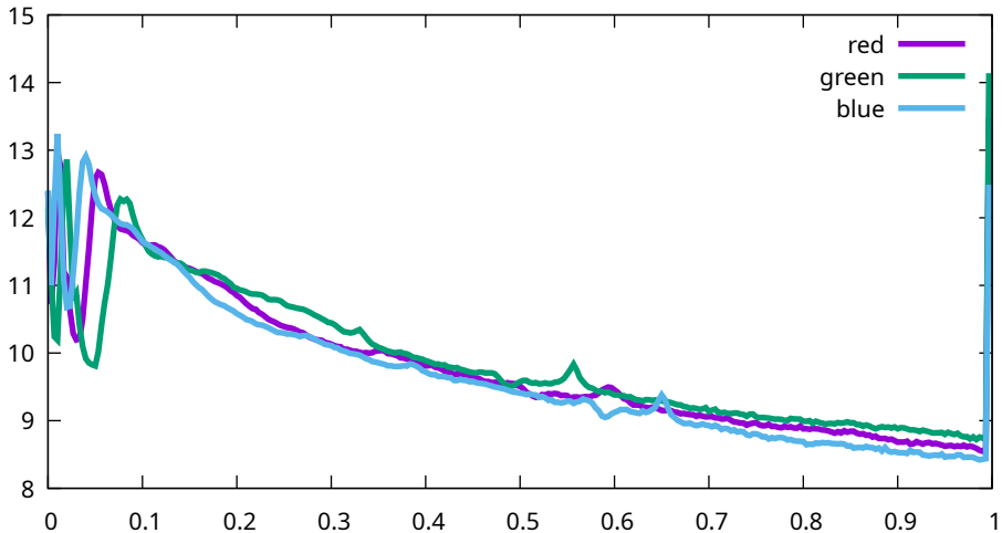
Histogram - Canon, EOS R5m2, 1000 ISO (9T0A0174)
