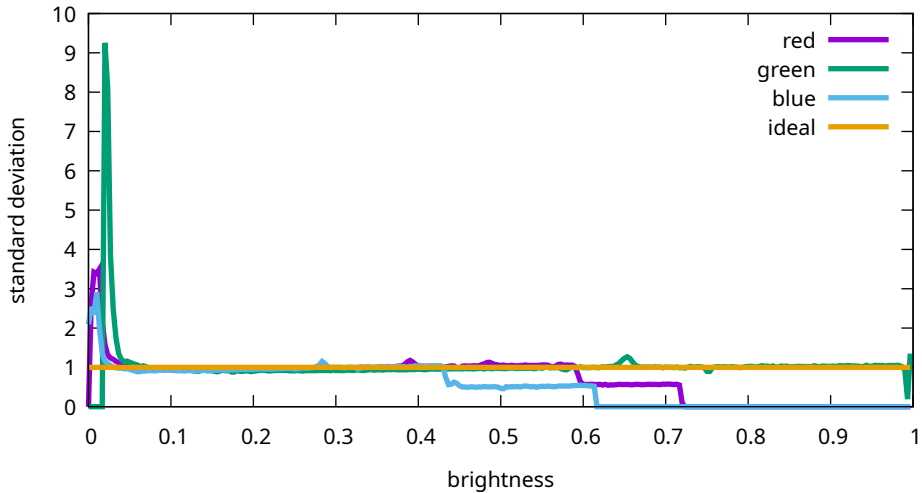
Flat noise levels - Canon, EOS R5m2, 320 ISO (9T0A0169)
