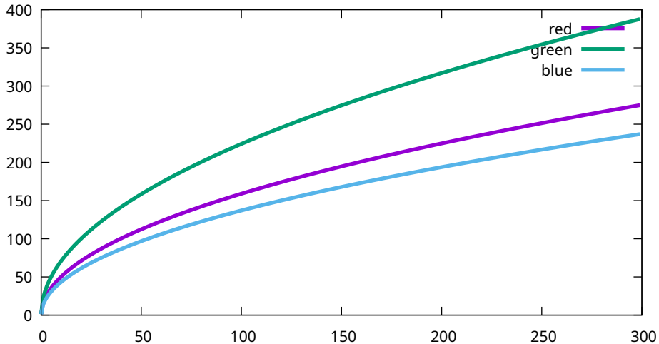
Conversion curves - Canon, EOS R5m2, 2500 ISO (9T0A0178)
