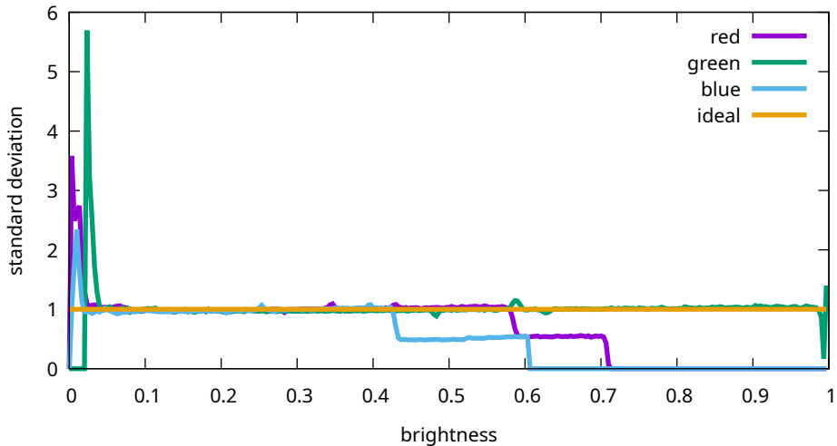
Flat noise levels - Canon, EOS R5m2, 500 ISO (9T0A0171)
