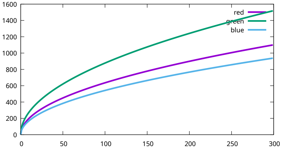
Conversion curves - Canon, EOS R5m2, 125 ISO (9T0A0163)
