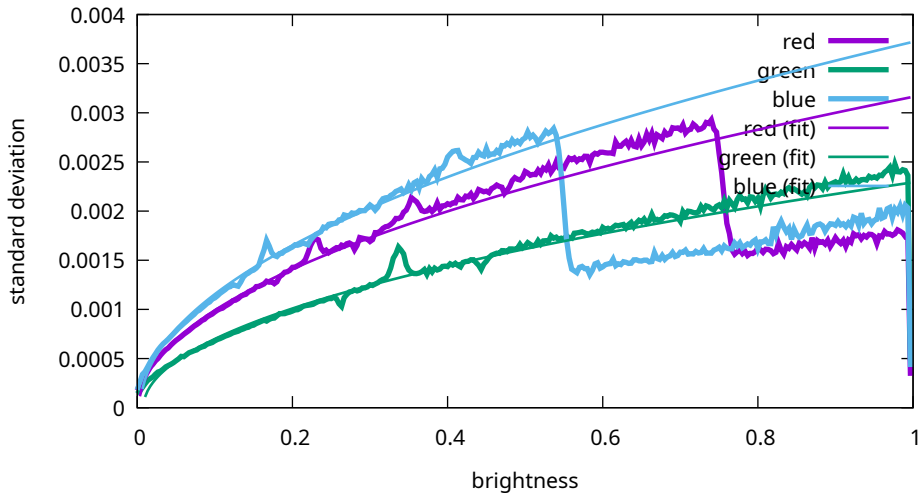
Noise levels - Canon, EOS R5m2, 400 ISO (9T0A0170)
