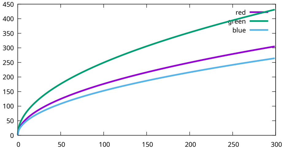
Conversion curves - Canon, EOS R5m2, 2000 ISO (9T0A0177)
