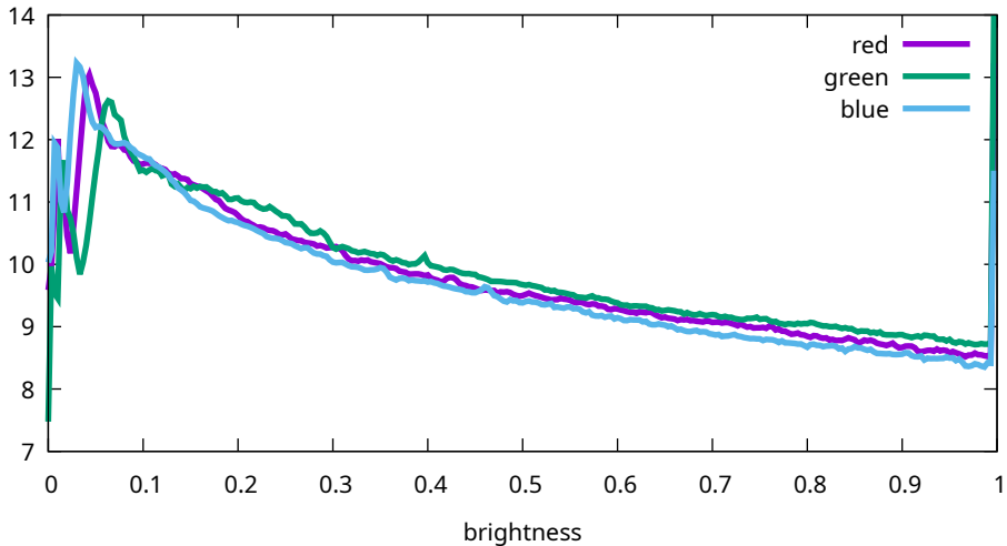
Flat histogram - Canon, EOS R5m2, 200 ISO (9T0A0165)
