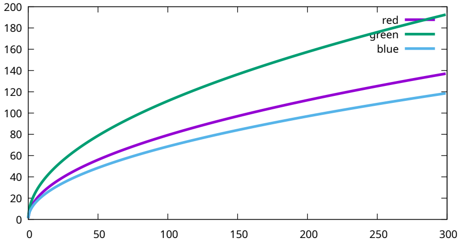
Conversion curves - Canon, EOS R5m2, 10000 ISO (9T0A0184)
