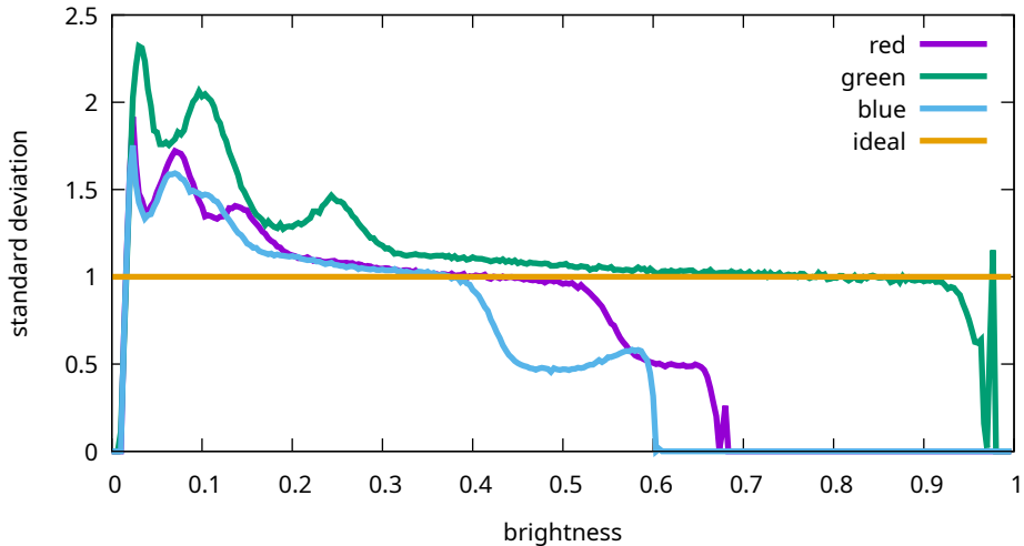
Flat noise levels - Canon, EOS R5m2, 40000 ISO (9T0A0190)
