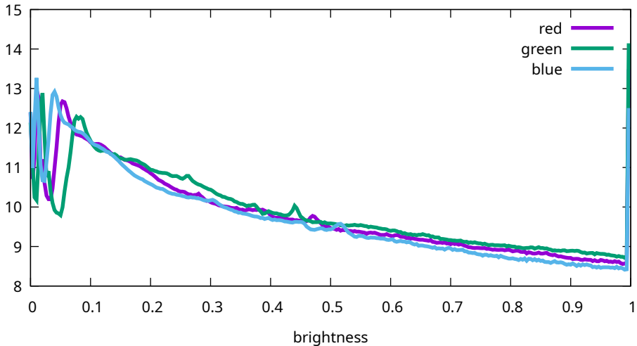
Flat histogram - Canon, EOS R5m2, 800 ISO (9T0A0173)
