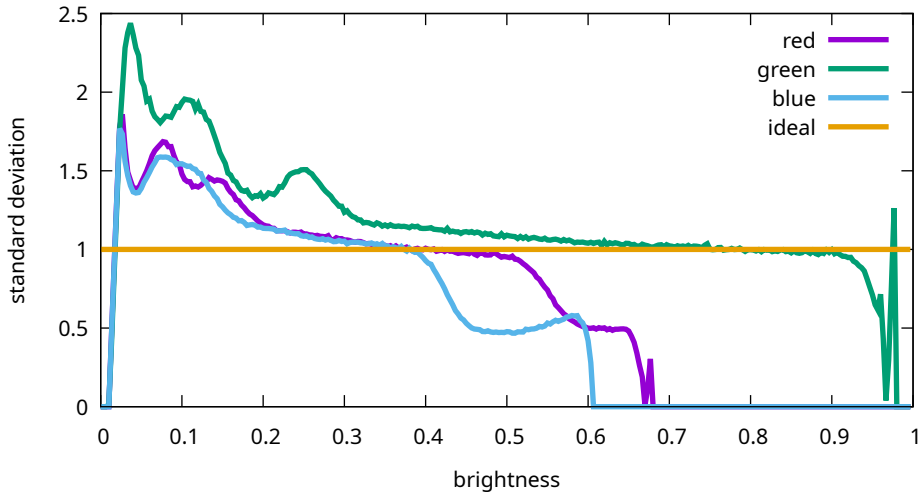
Flat noise levels - Canon, EOS R5m2, 51200 ISO (9T0A0191)
