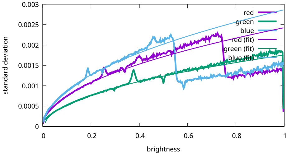
Noise levels - Canon, EOS R5m2, 250 ISO (9T0A0168)
