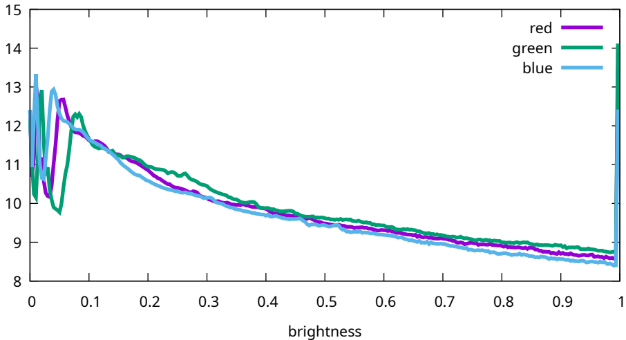
Flat histogram - Canon, EOS R5m2, 500 ISO (9T0A0171)
