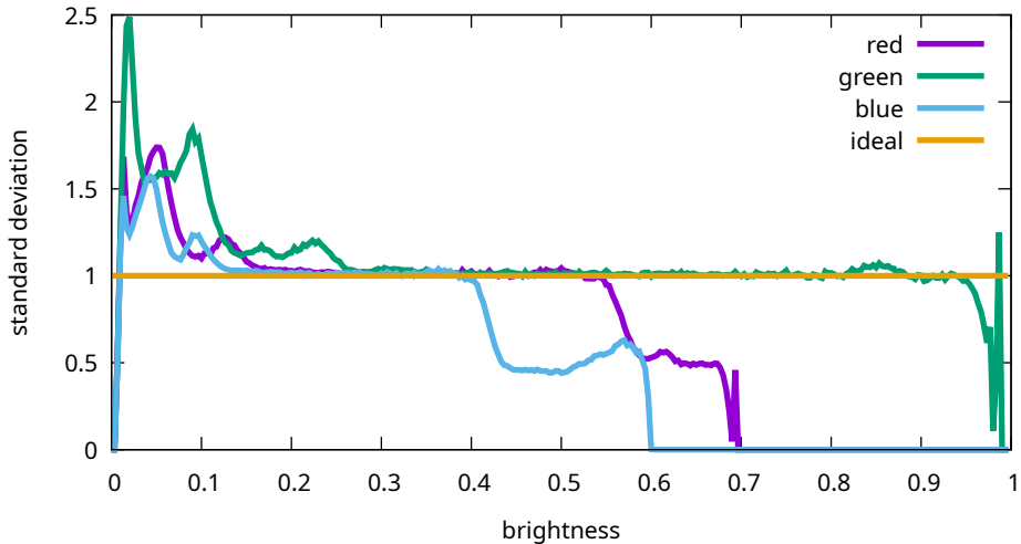
Flat noise levels - Canon, EOS R5m2, 12800 ISO (9T0A0185)
