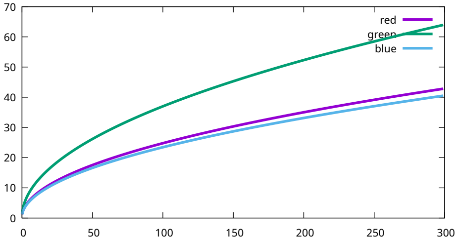
Conversion curves - Canon, EOS R5m2, 102400 ISO (9T0A0192)
