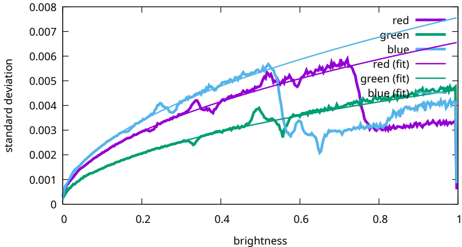
Noise levels - Canon, EOS R5m2, 2000 ISO (9T0A0177)
