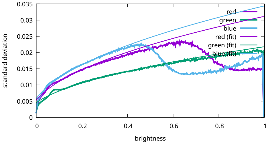
Noise levels - Canon, EOS R5m2, 51200 ISO (9T0A0191)
