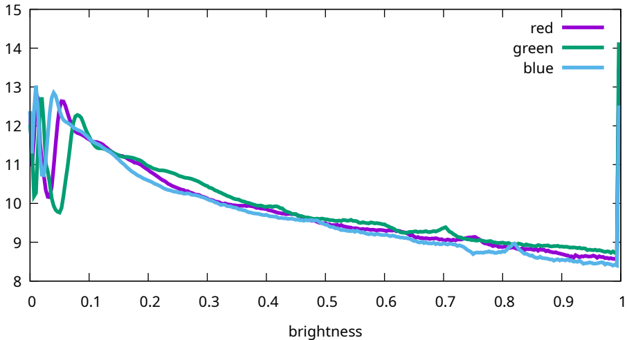
Flat histogram - Canon, EOS R5m2, 2500 ISO (9T0A0178)
