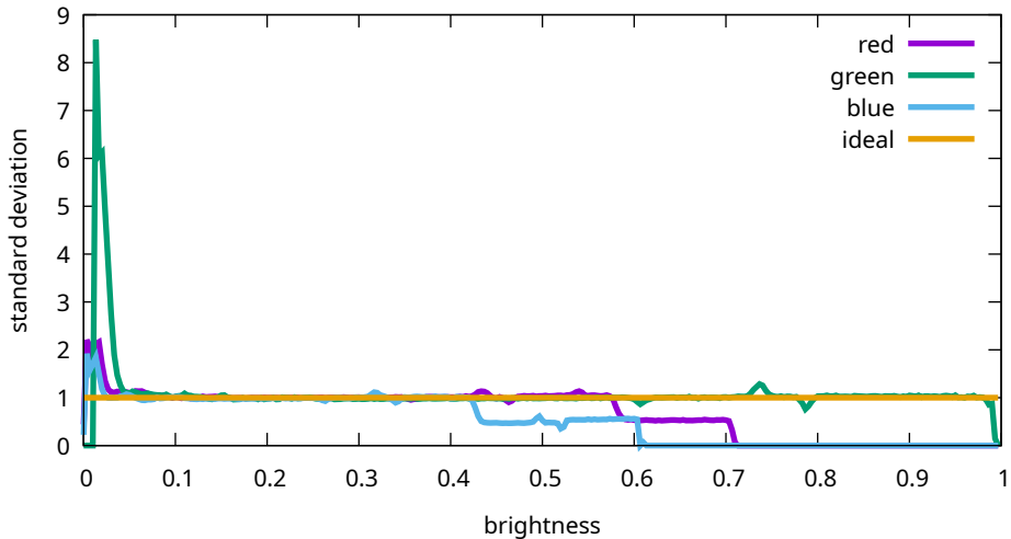
Flat noise levels - Canon, EOS R5m2, 1250 ISO (9T0A0175)
