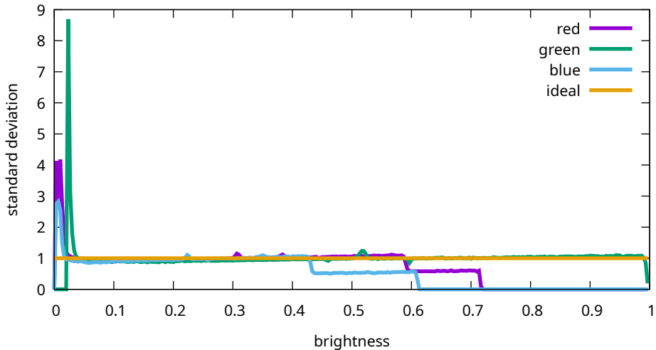
Flat noise levels - Canon, EOS R5m2, 200 ISO (9T0A0166)
