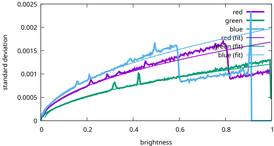
Noise levels - Canon, EOS R5m2, 100 ISO (9T0A0159)
