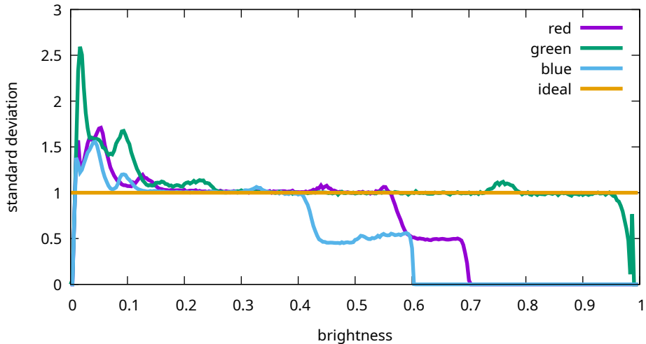
Flat noise levels - Canon, EOS R5m2, 10000 ISO (9T0A0184)
