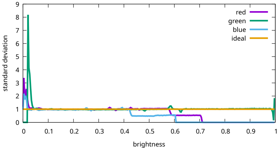
Flat noise levels - Canon, EOS R5m2, 800 ISO (9T0A0173)
