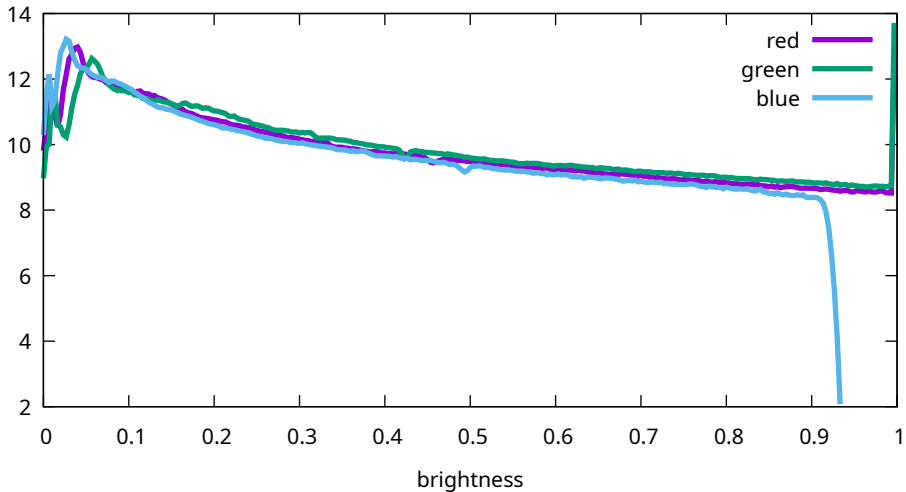
Flat histogram - Canon, EOS R5m2, 50 ISO (9T0A0129)
