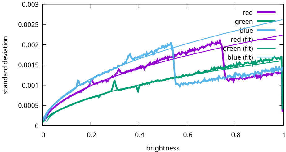
Noise levels - Canon, EOS R5m2, 200 ISO (9T0A0165)
