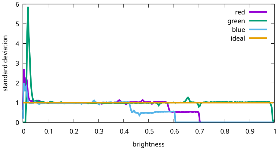
Flat noise levels - Canon, EOS R5m2, 1000 ISO (9T0A0174)
