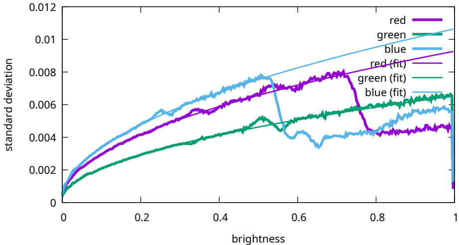
Noise levels - Canon, EOS R5m2, 4000 ISO (9T0A0180)
