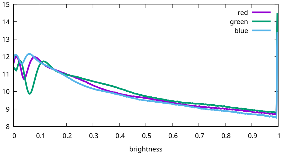
Flat histogram - Canon, EOS R5m2, 25600 ISO (9T0A0188)
