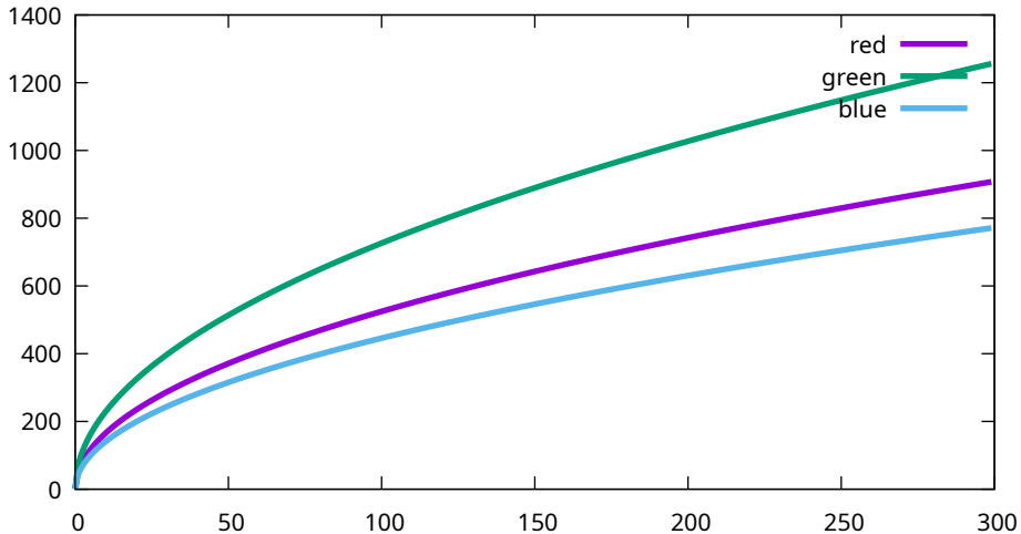
Conversion curves - Canon, EOS R5m2, 200 ISO (9T0A0167)
